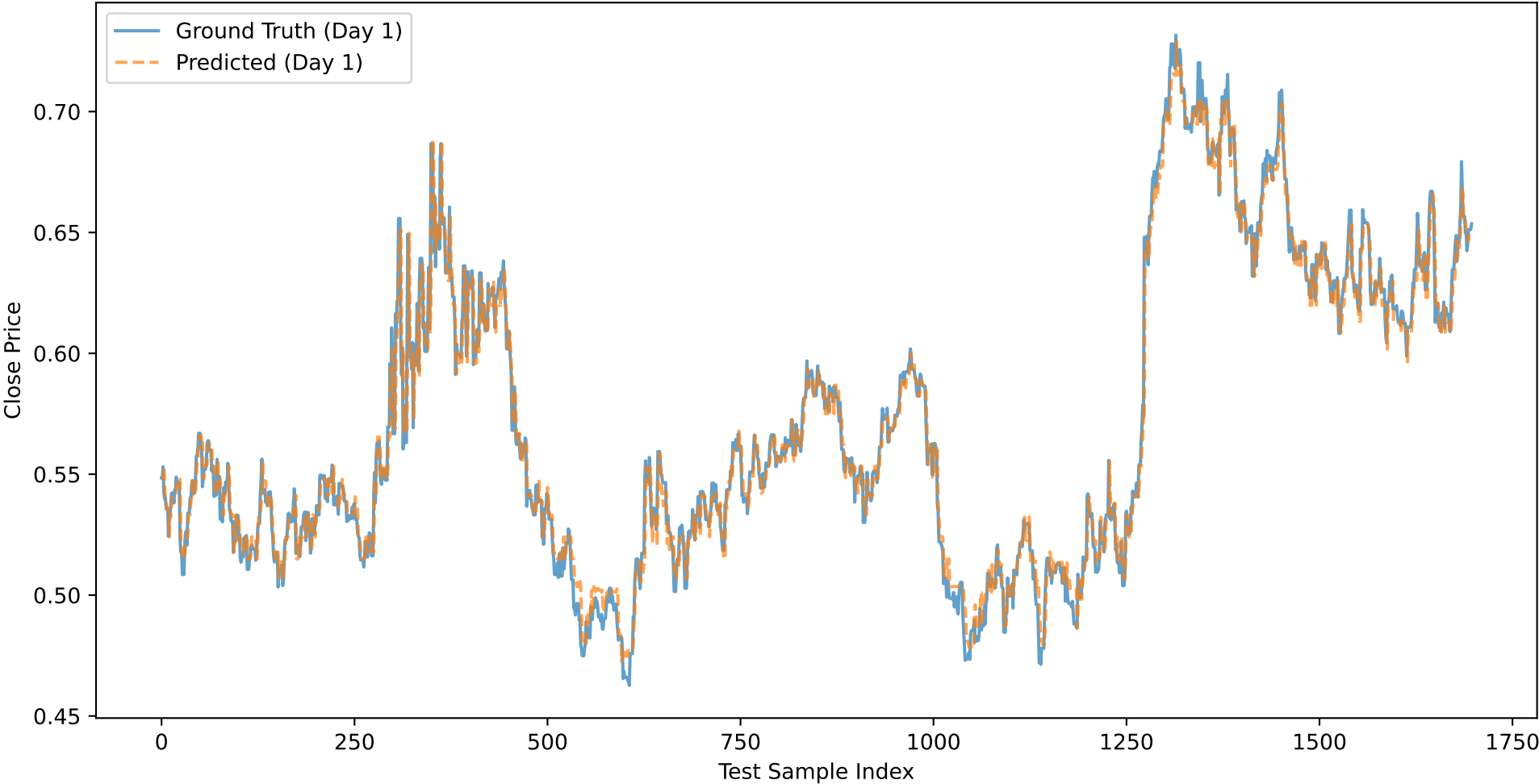
GILD: Close Price Prediction (Day 1) - BASELINE_XGB_CLOSE
