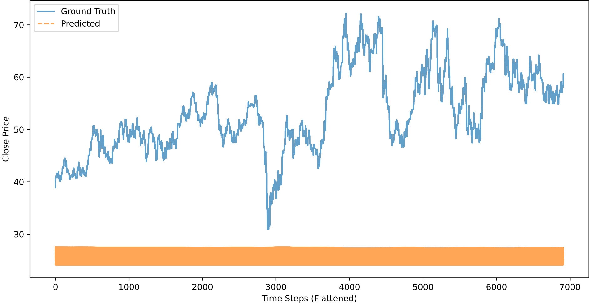
BHP: Close Price - Ground Truth vs Predicted (BASELINE_CLOSE, 21 stocks)
