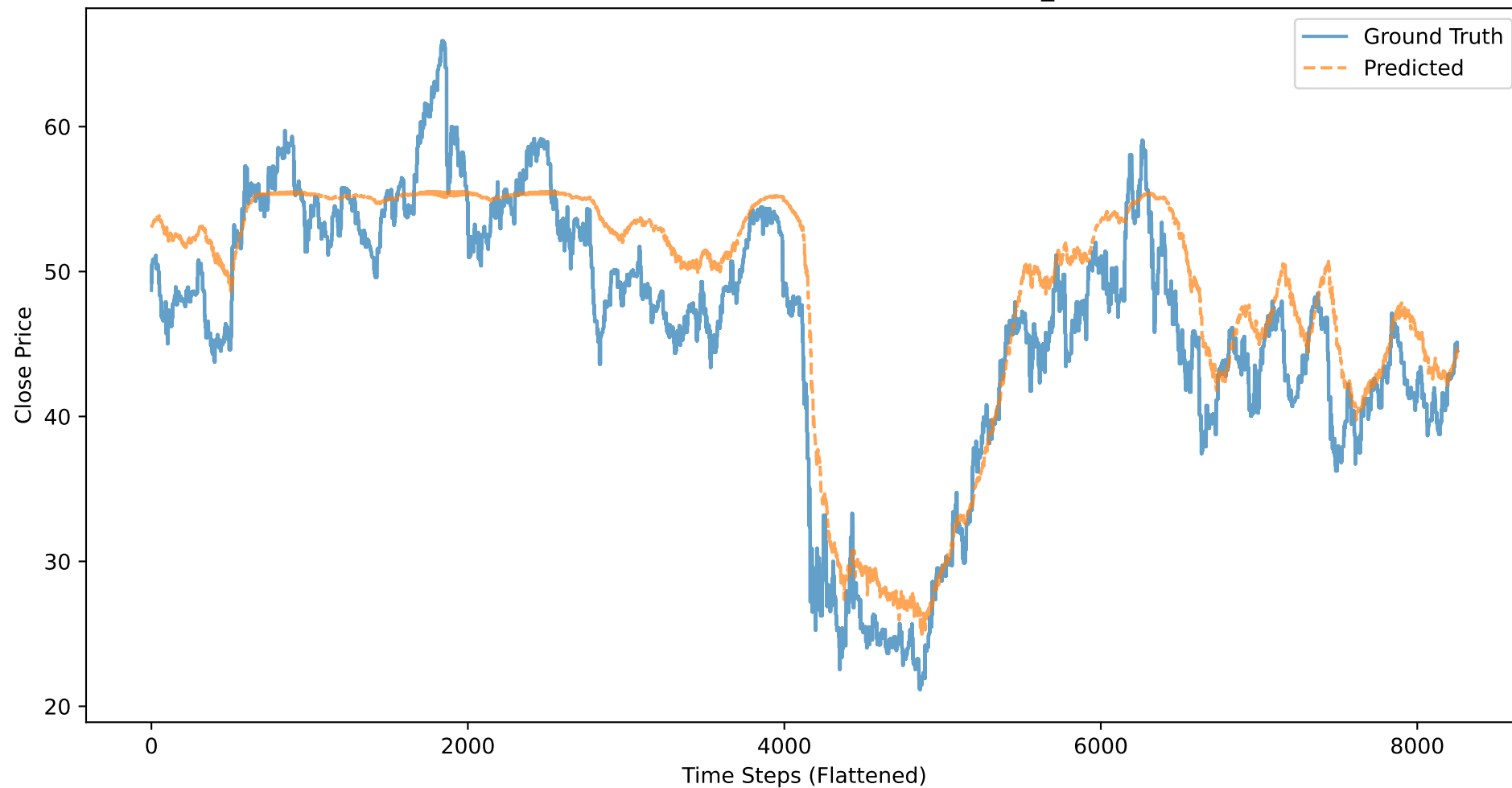
WFC: Close Price - Ground Truth vs Predicted (BASELINE_CLOSE, 50 stocks)
