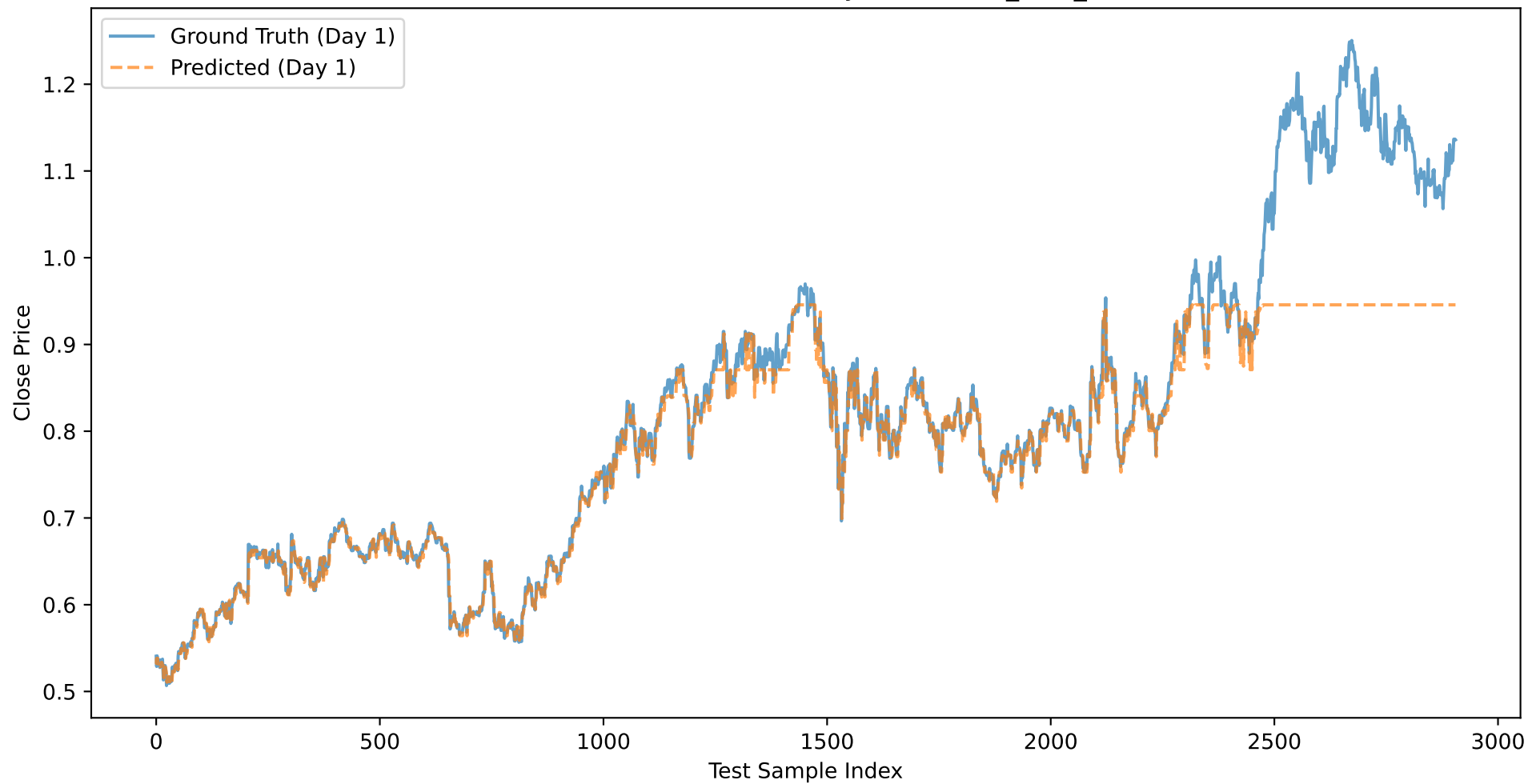
MRK: Close Price Prediction (Day 1) - NOVEL_XGB_CLOSE
