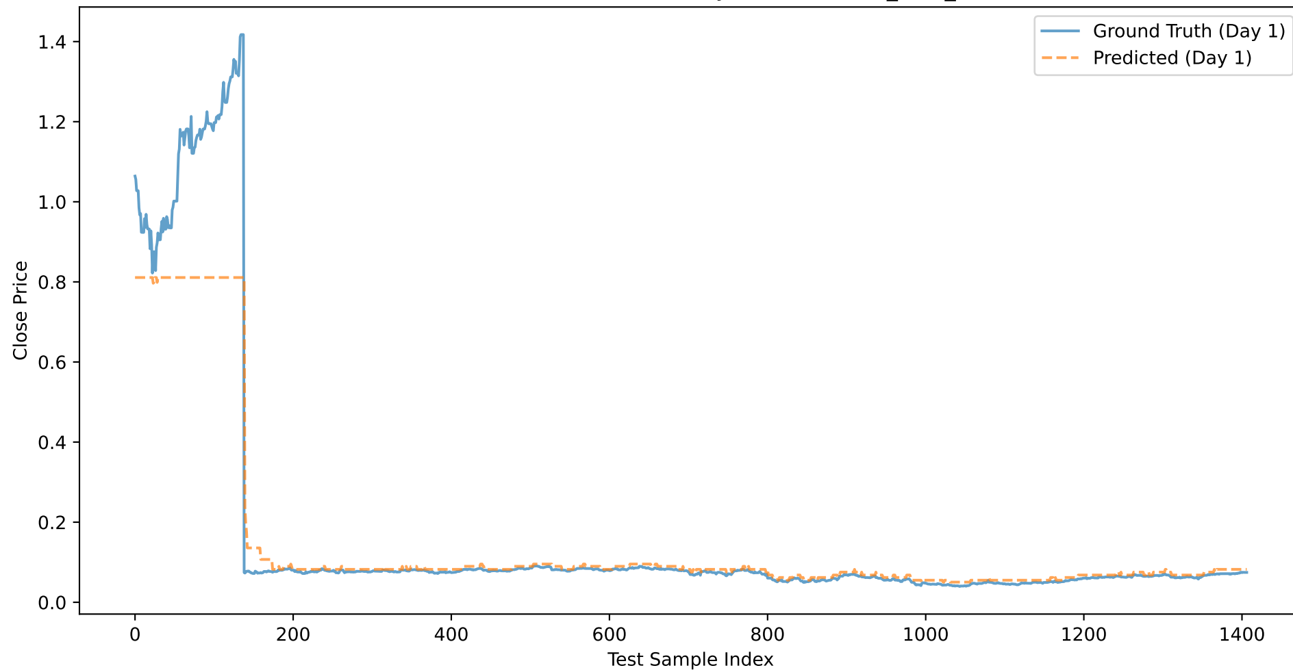
AMZN: Close Price Prediction (Day 1) - BASELINE_XGB_CLOSE
