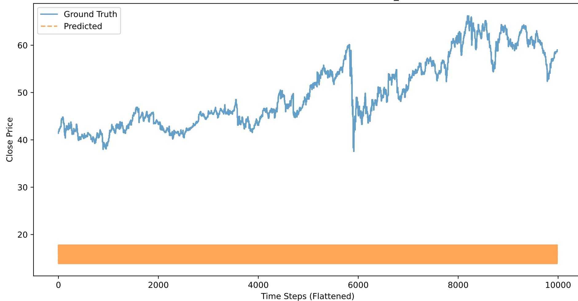
KO: Close Price - Ground Truth vs Predicted (BASELINE_CLOSE, 21 stocks)
