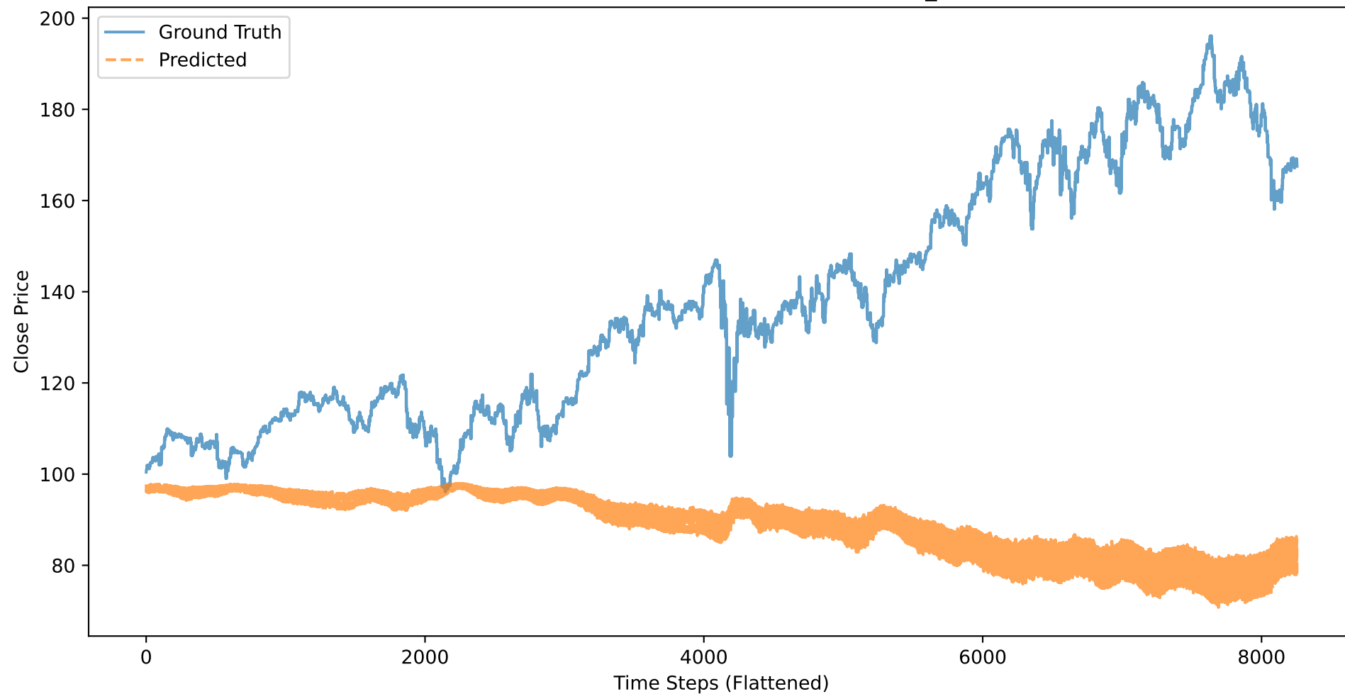
PEP: Close Price - Ground Truth vs Predicted (BASELINE_CLOSE, 50 stocks)
