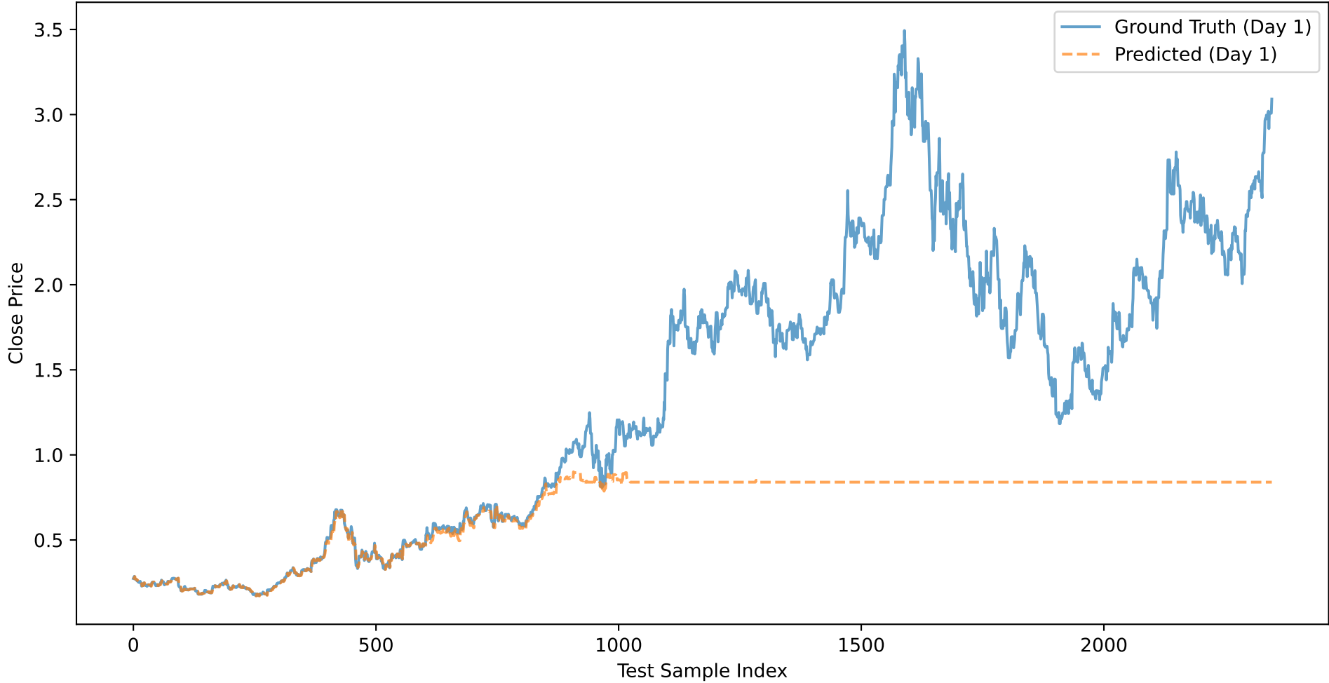
AMD: Close Price Prediction (Day 1) - BASELINE_XGB_CLOSE
