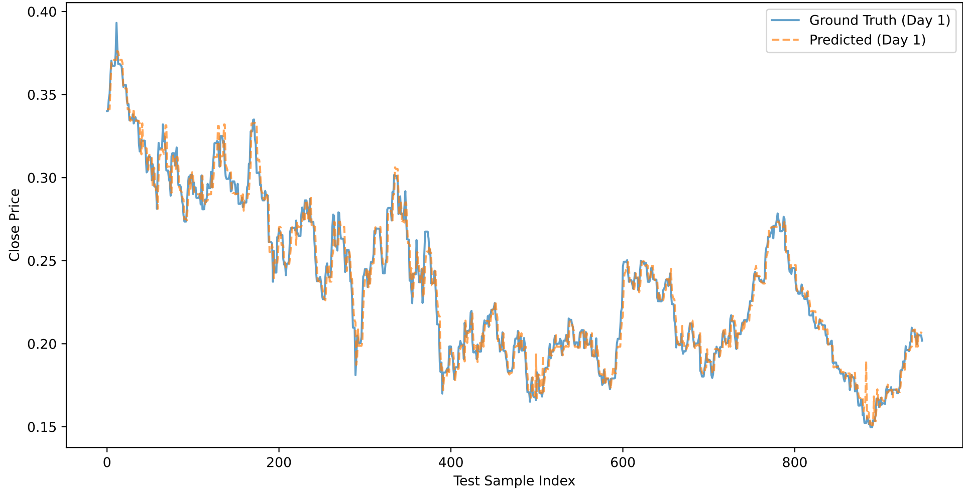
AAL: Close Price Prediction (Day 1) - NOVEL_XGB_CLOSE
