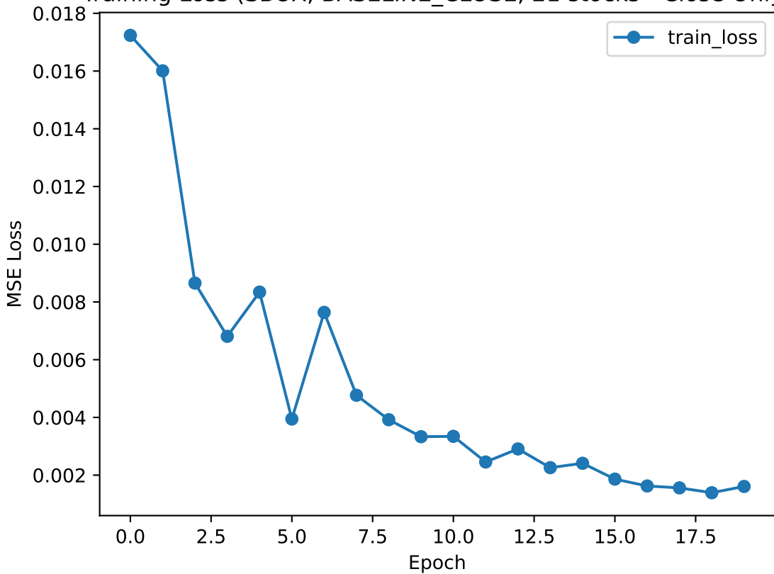
Training Loss (SBUX, BASELINE_CLOSE, 21 stocks - Close Only)
