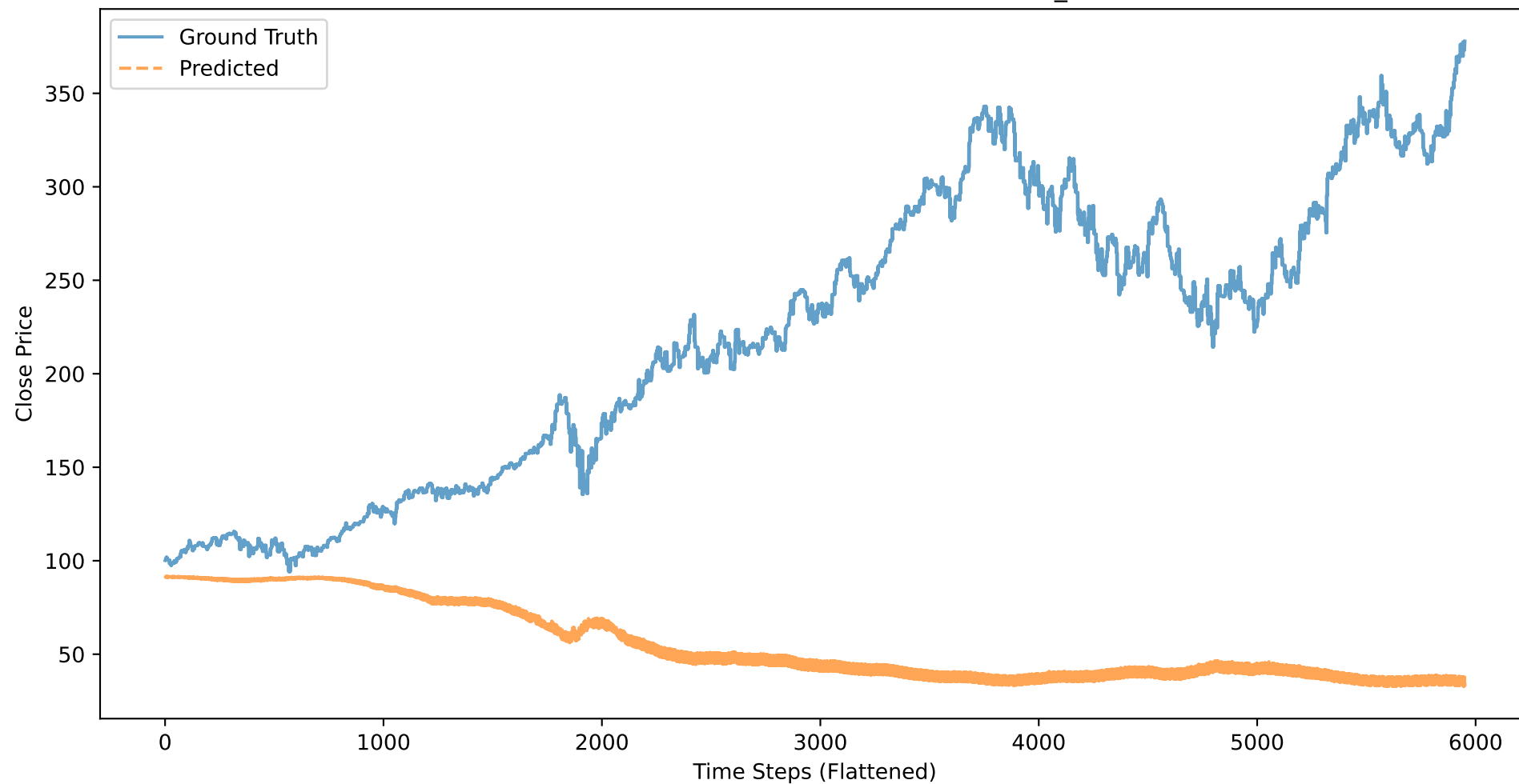
MSFT: Close Price - Ground Truth vs Predicted (BASELINE_CLOSE, 50 stocks)
