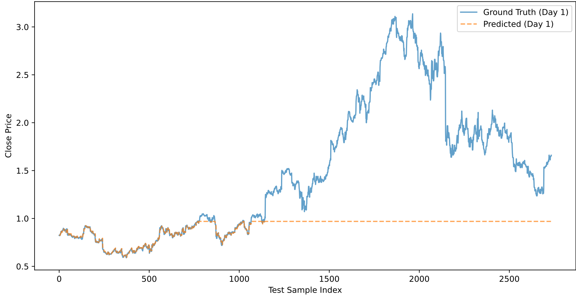
TGT: Close Price Prediction (Day 1) - NOVEL_XGB_CLOSE
