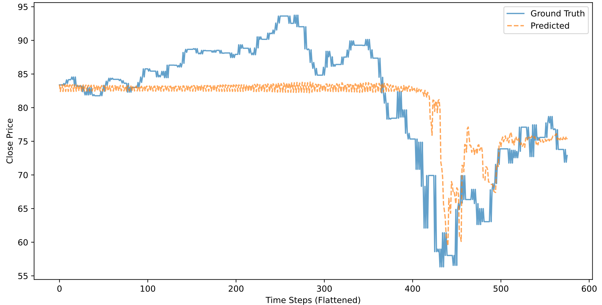
SBUX: Close Price - Ground Truth vs Predicted (BASELINE_CLOSE, 21 stocks)
