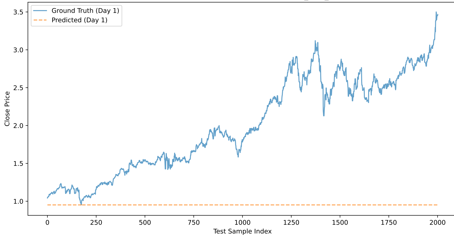
COST: Close Price Prediction (Day 1) - NOVEL_XGB_CLOSE
