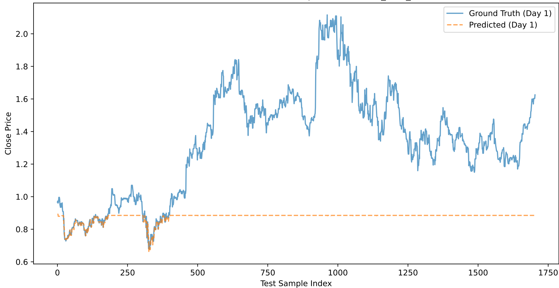
QCOM: Close Price Prediction (Day 1) - BASELINE_XGB_CLOSE
