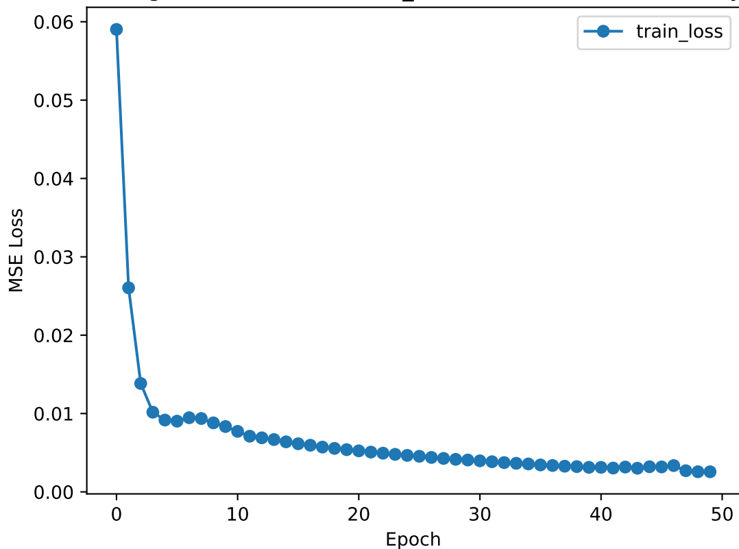
Training Loss (CRM, BASELINE_CLOSE, 50 stocks - Close Only)
