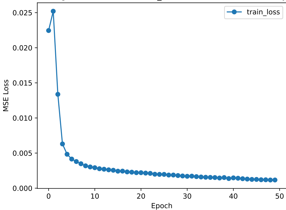
Training Loss (USO, BASELINE_CLOSE, 50 stocks - Close Only)
