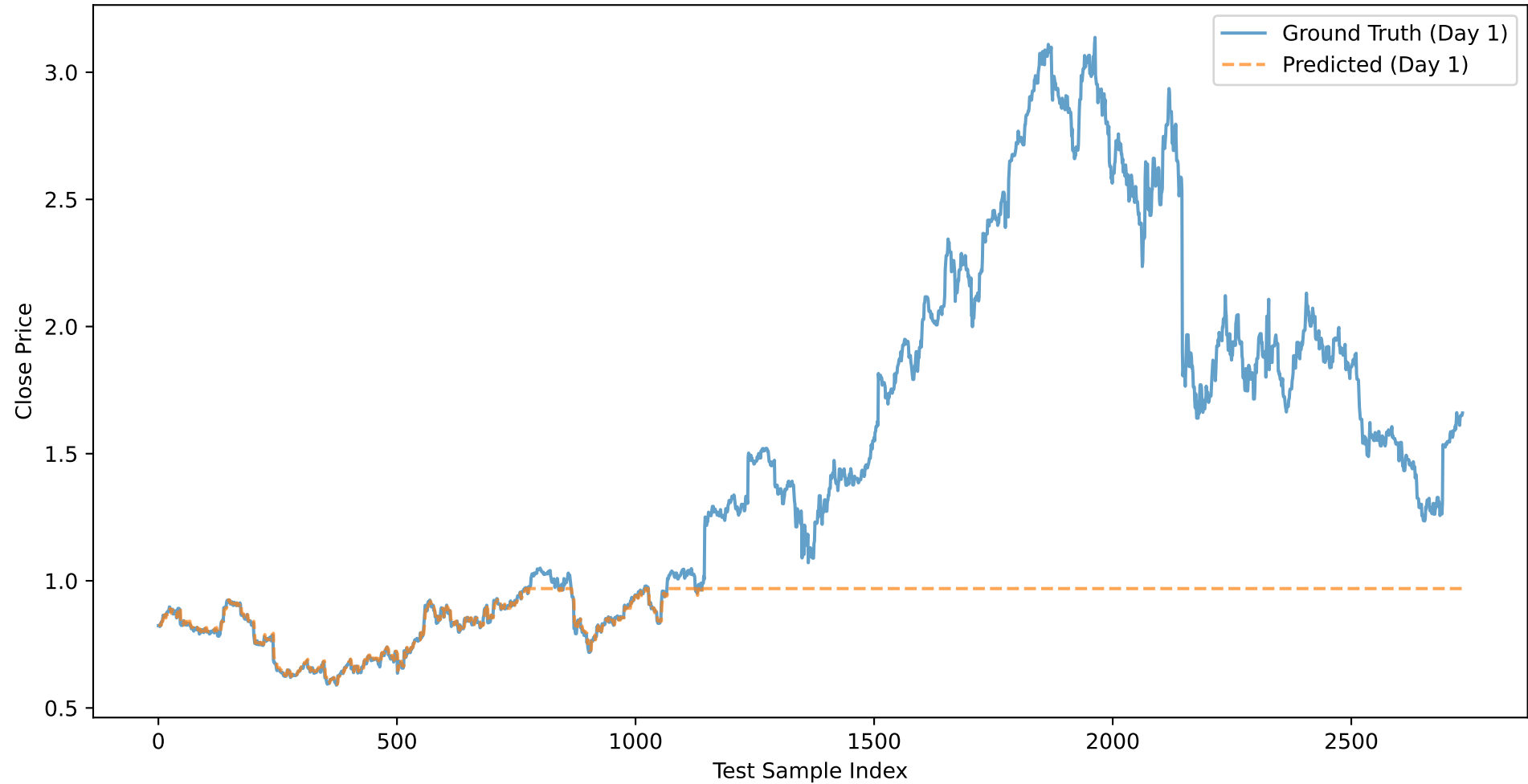
TGT: Close Price Prediction (Day 1) - BASELINE_XGB_CLOSE
