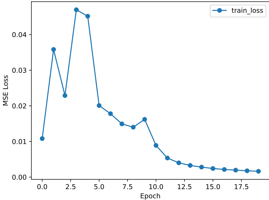
Training Loss (COST, BASELINE_CLOSE, 21 stocks - Close Only)
