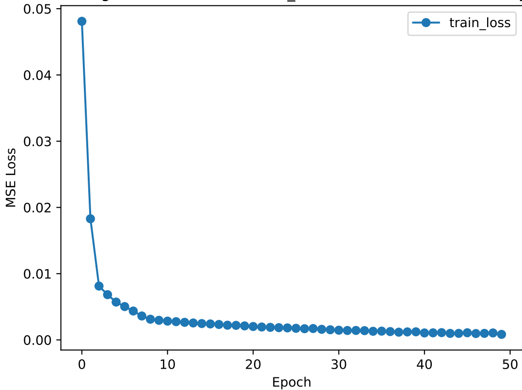
Training Loss (MSFT, BASELINE_CLOSE, 50 stocks - Close Only)
