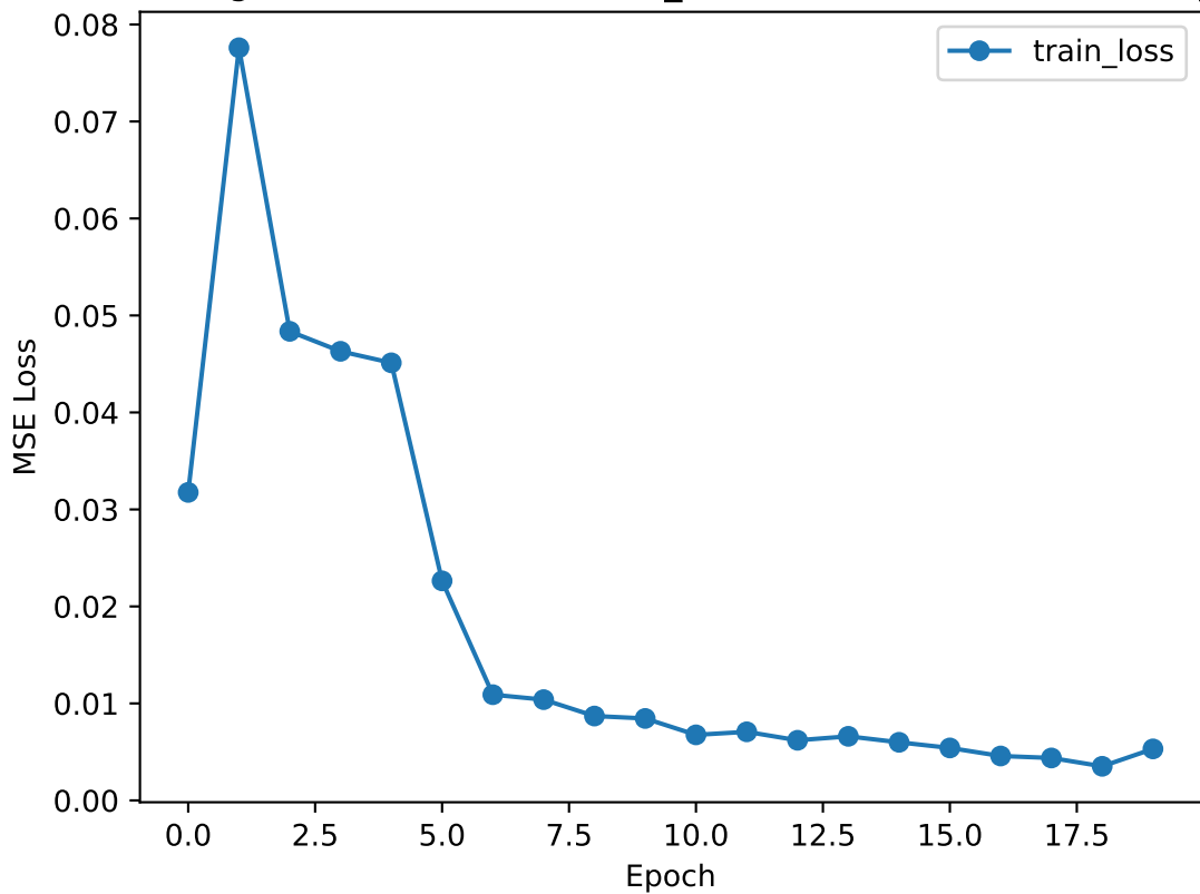
Training Loss (NVDA, BASELINE_CLOSE, 21 stocks - Close Only)
