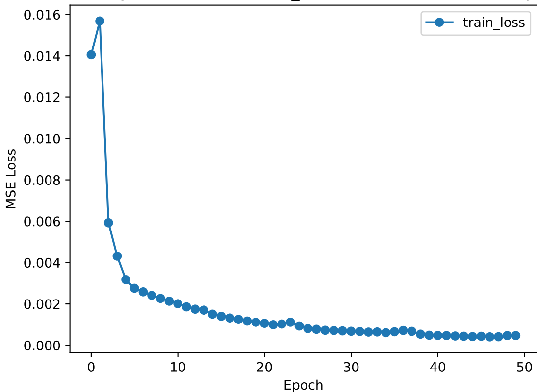
Training Loss (DIS, BASELINE_CLOSE, 50 stocks - Close Only)
