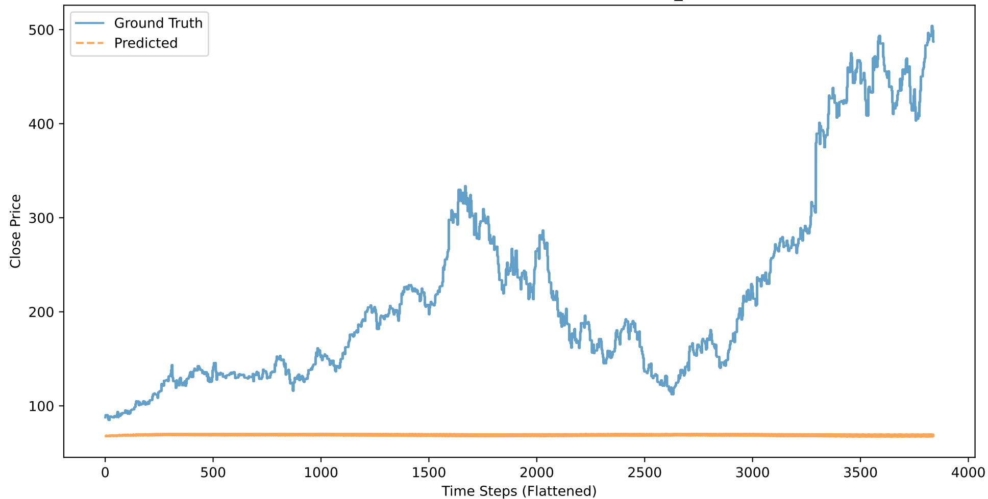
NVDA: Close Price - Ground Truth vs Predicted (BASELINE_CLOSE, 50 stocks)
