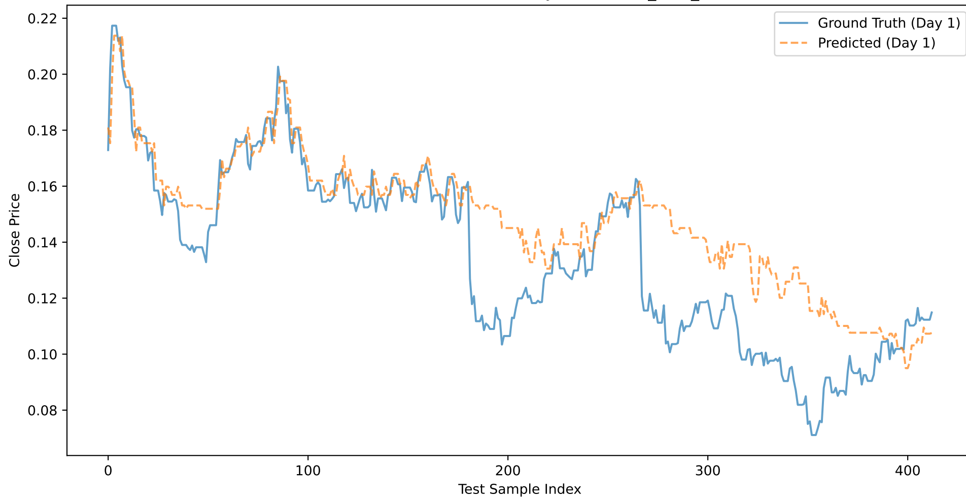
PYPL: Close Price Prediction (Day 1) - NOVEL_XGB_CLOSE
