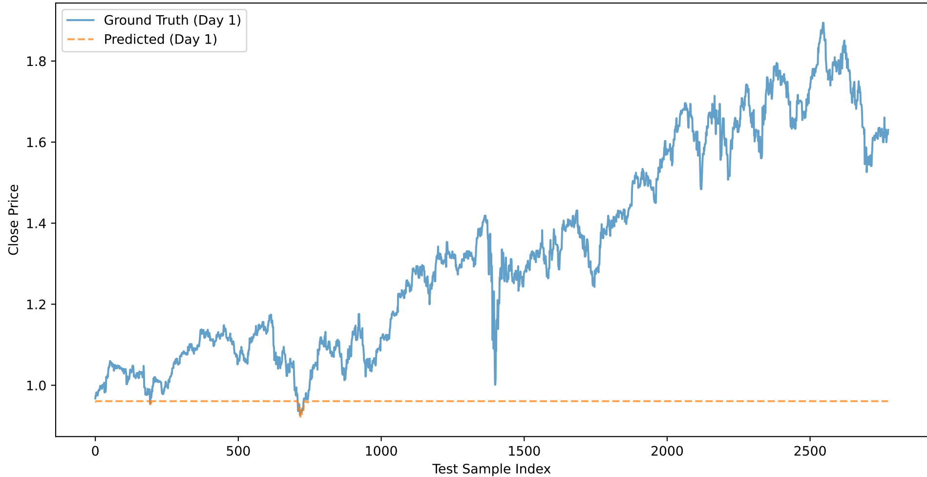
PEP: Close Price Prediction (Day 1) - BASELINE_XGB_CLOSE
