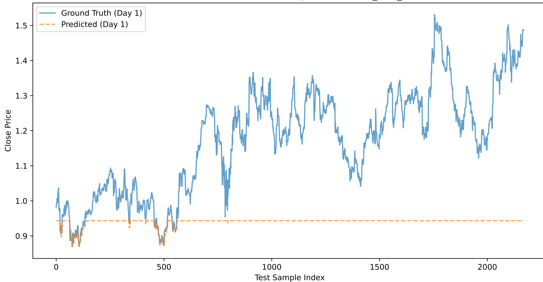
AMGN: Close Price Prediction (Day 1) - BASELINE_XGB_CLOSE
