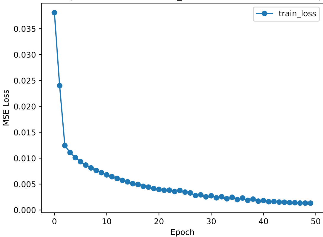
Training Loss (COP, BASELINE_CLOSE, 50 stocks - Close Only)
