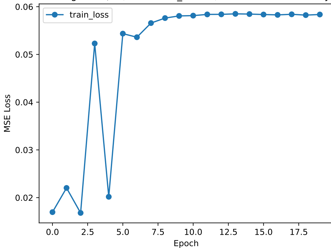
Training Loss (GE, BASELINE_CLOSE, 21 stocks - Close Only)
