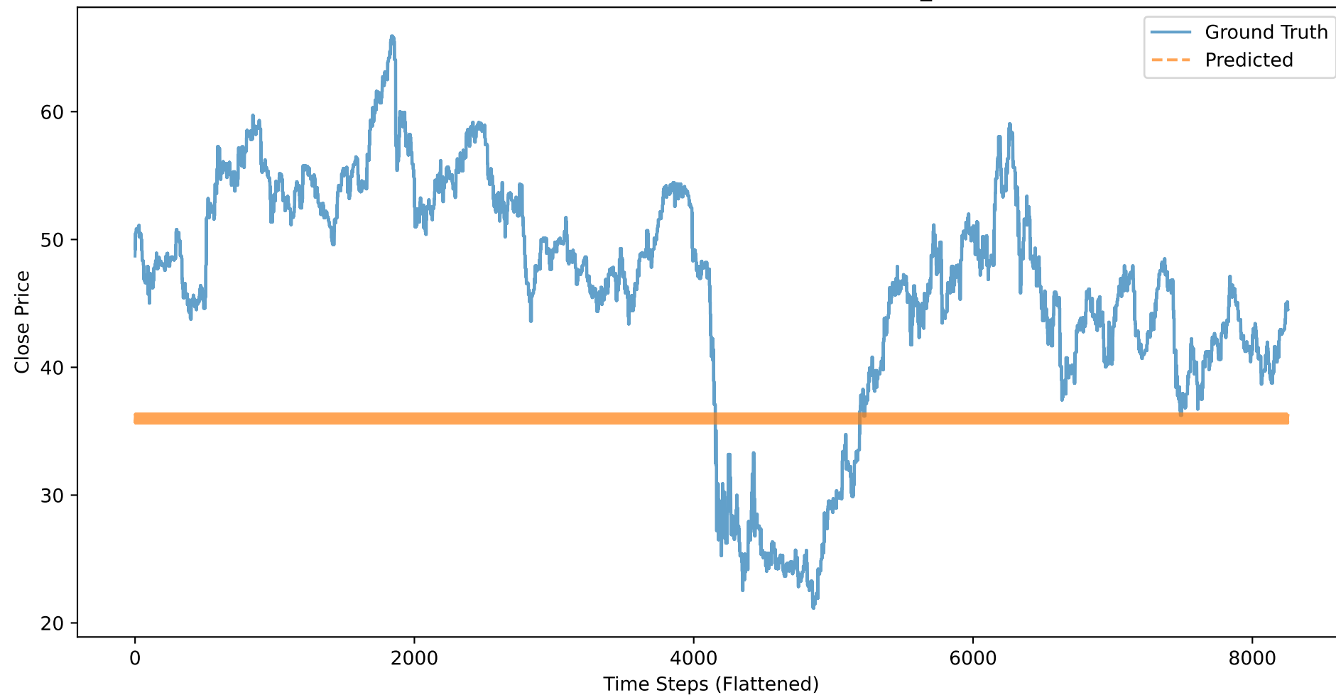
WFC: Close Price - Ground Truth vs Predicted (BASELINE_CLOSE, 21 stocks)
