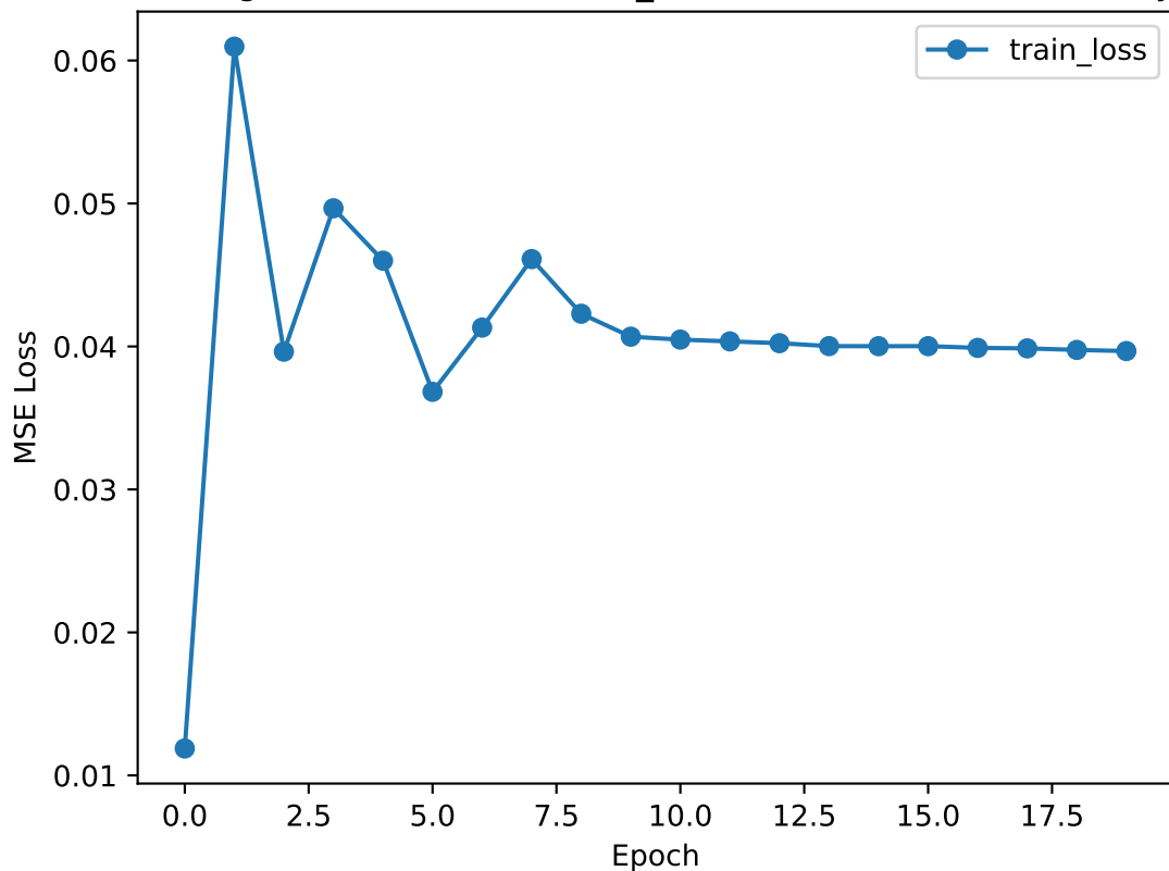
Training Loss (TSM, BASELINE_CLOSE, 21 stocks - Close Only)
