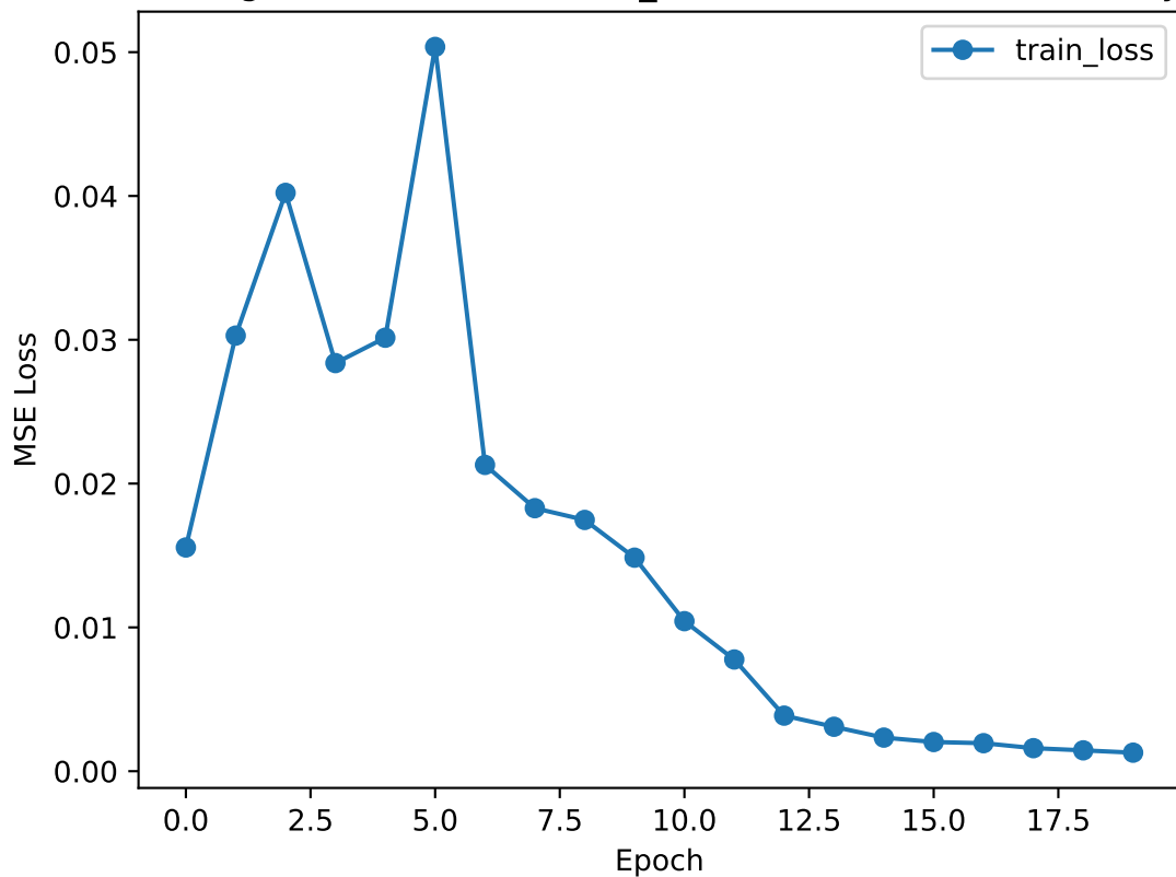
Training Loss (CVX, BASELINE_CLOSE, 21 stocks - Close Only)
