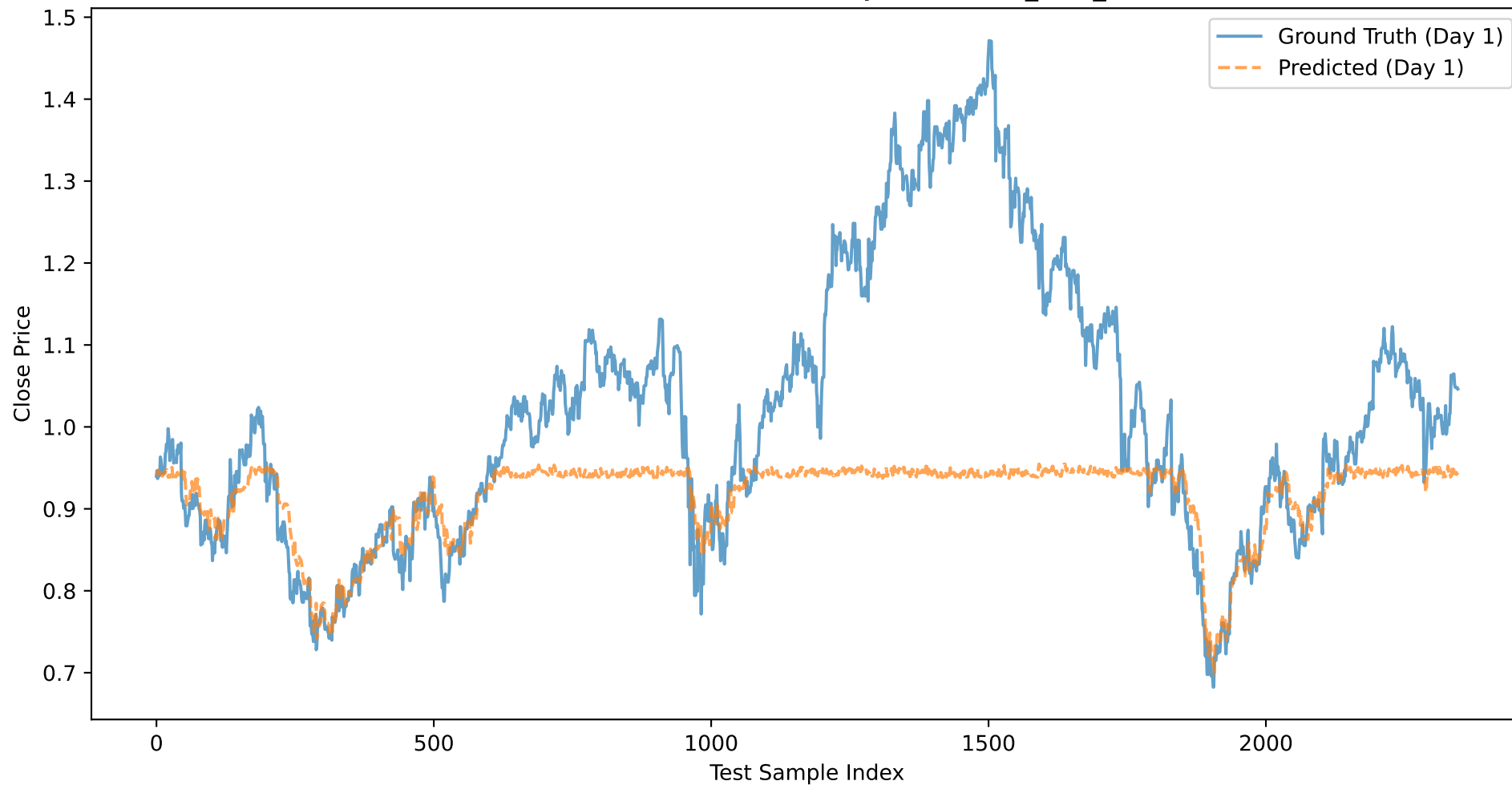
CMCSA: Close Price Prediction (Day 1) - NOVEL_XGB_CLOSE
