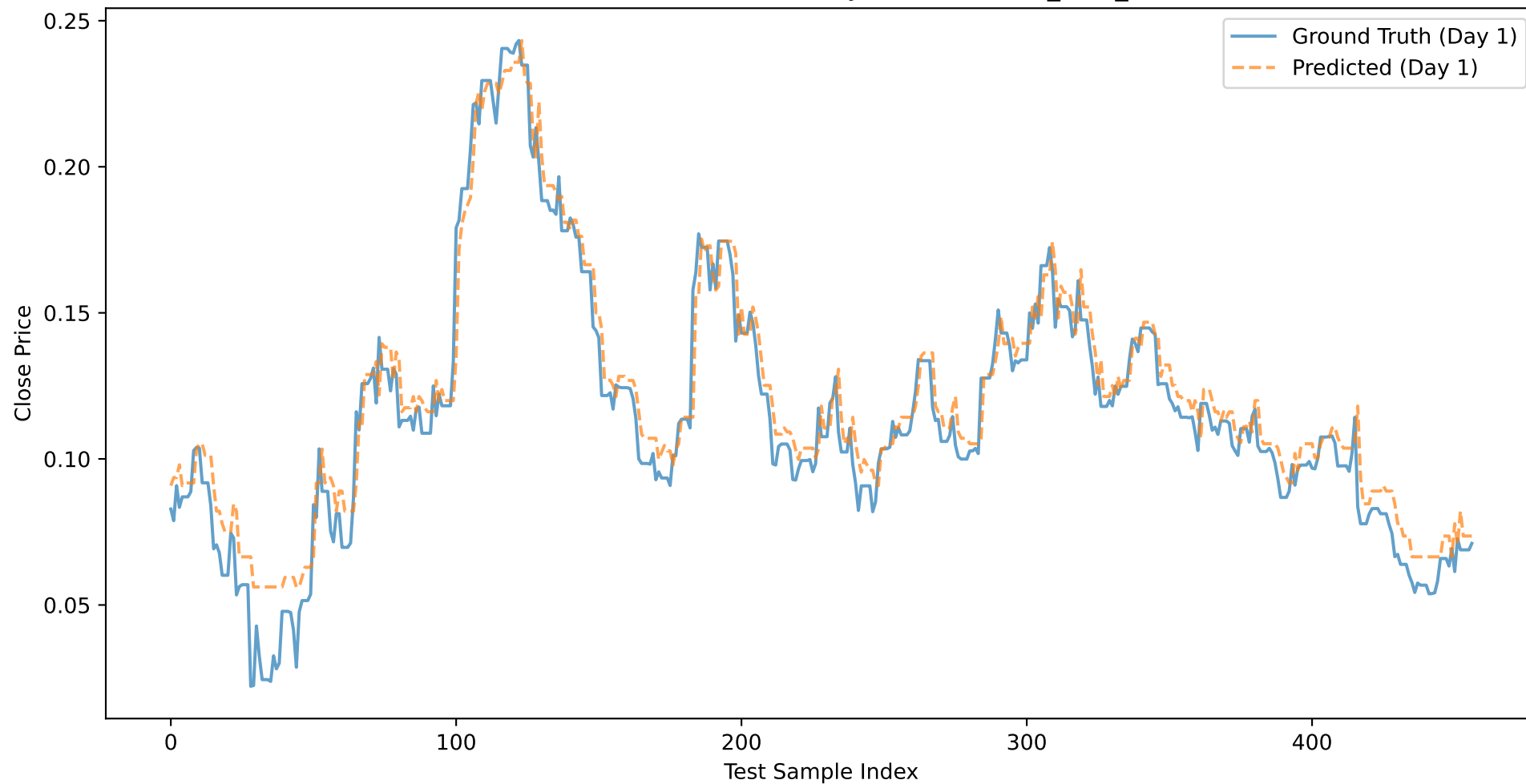
BABA: Close Price Prediction (Day 1) - BASELINE_XGB_CLOSE
