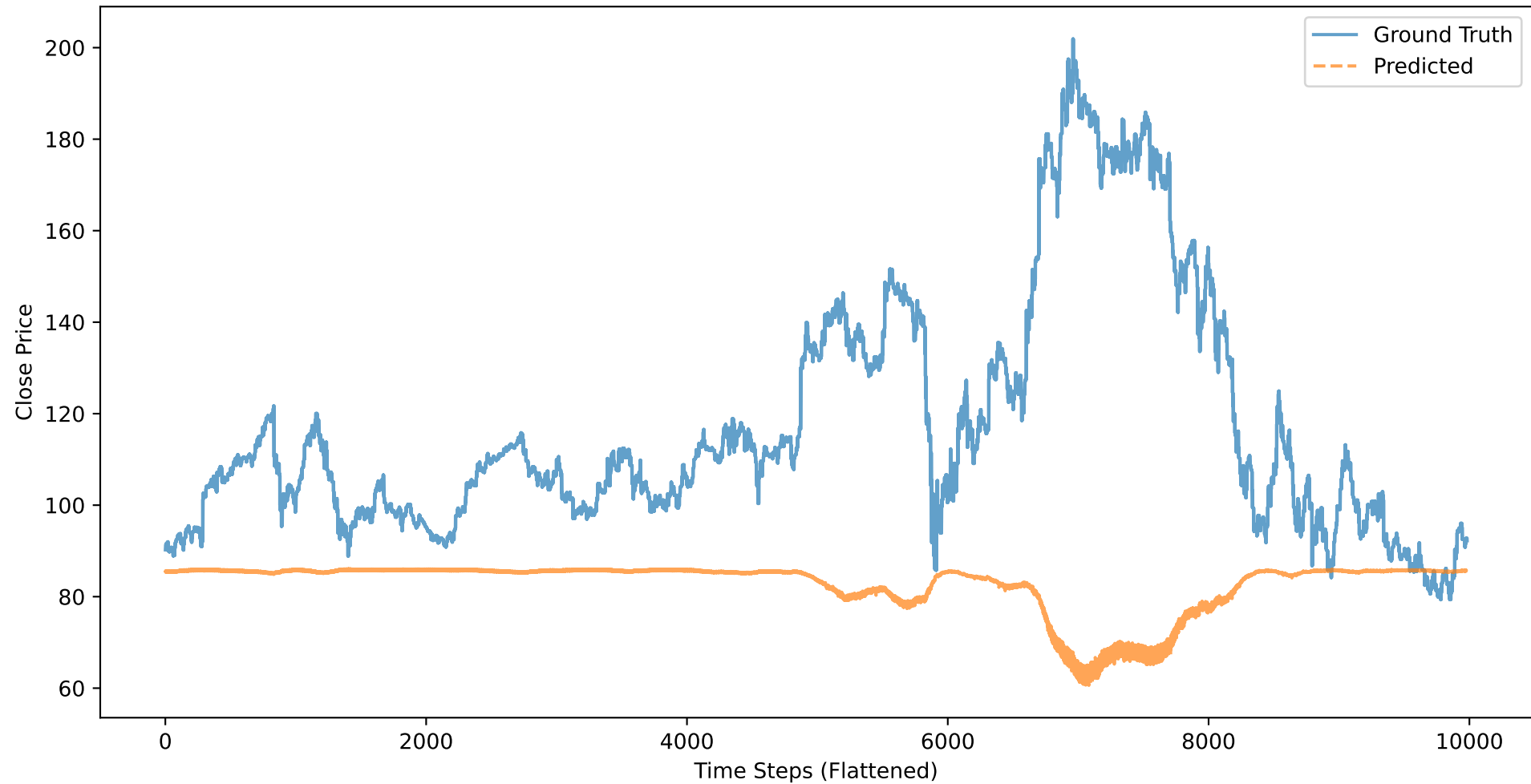
DIS: Close Price - Ground Truth vs Predicted (BASELINE_CLOSE, 50 stocks)
