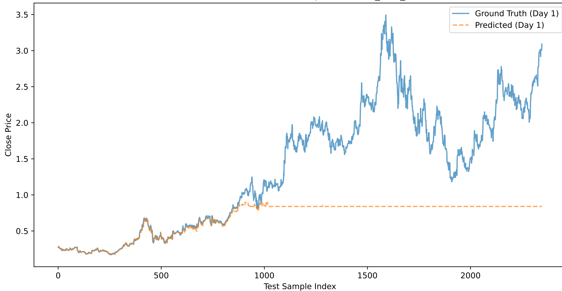
AMD: Close Price Prediction (Day 1) - NOVEL_XGB_CLOSE
