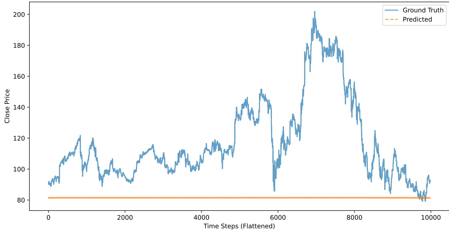
DIS: Close Price - Ground Truth vs Predicted (BASELINE_CLOSE, 21 stocks)
