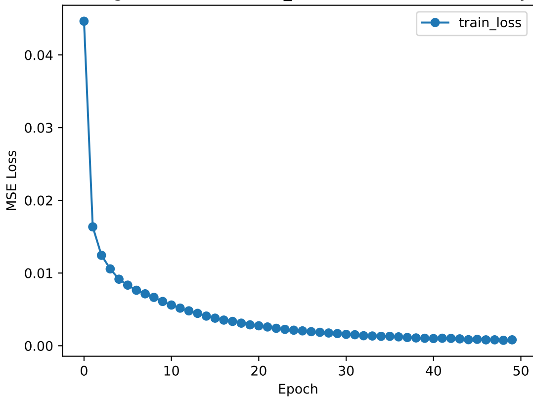
Training Loss (GE, BASELINE_CLOSE, 50 stocks - Close Only)
