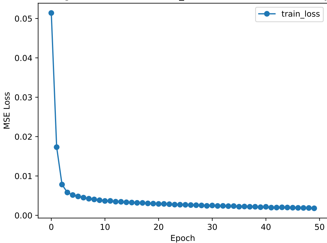
Training Loss (BIDU, BASELINE_CLOSE, 50 stocks - Close Only)
