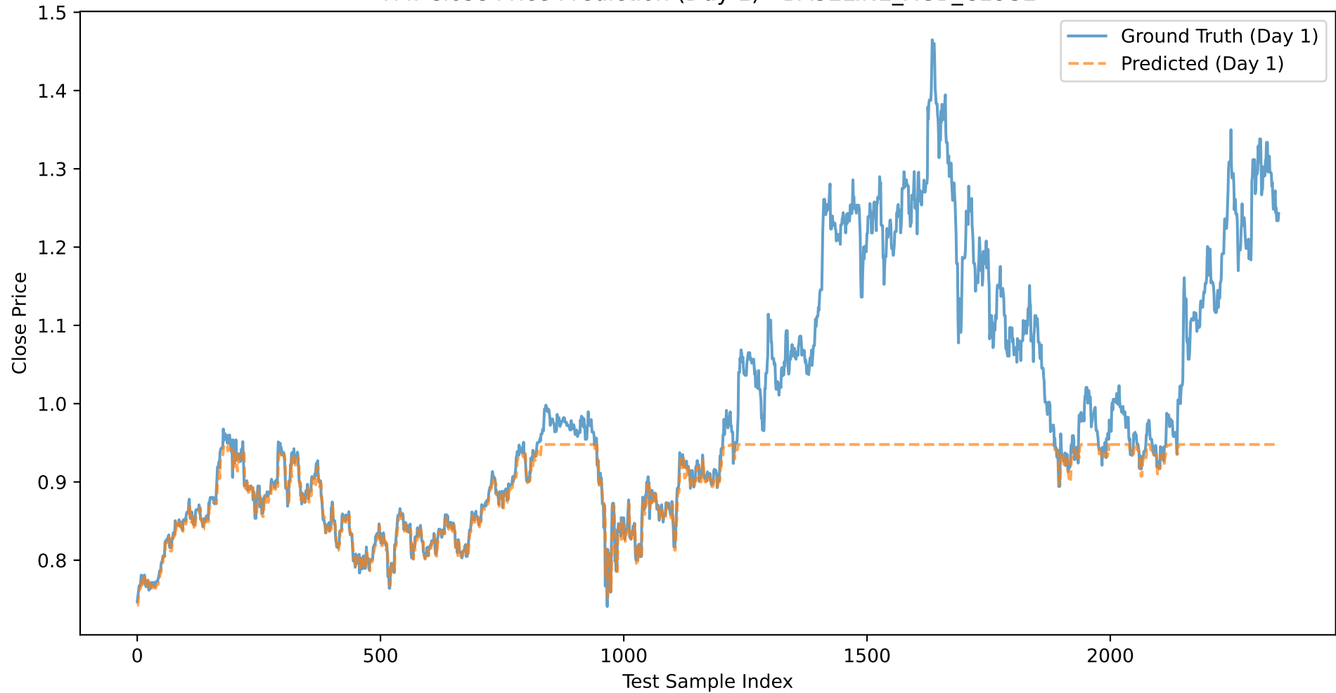
TM: Close Price Prediction (Day 1) - BASELINE_XGB_CLOSE
