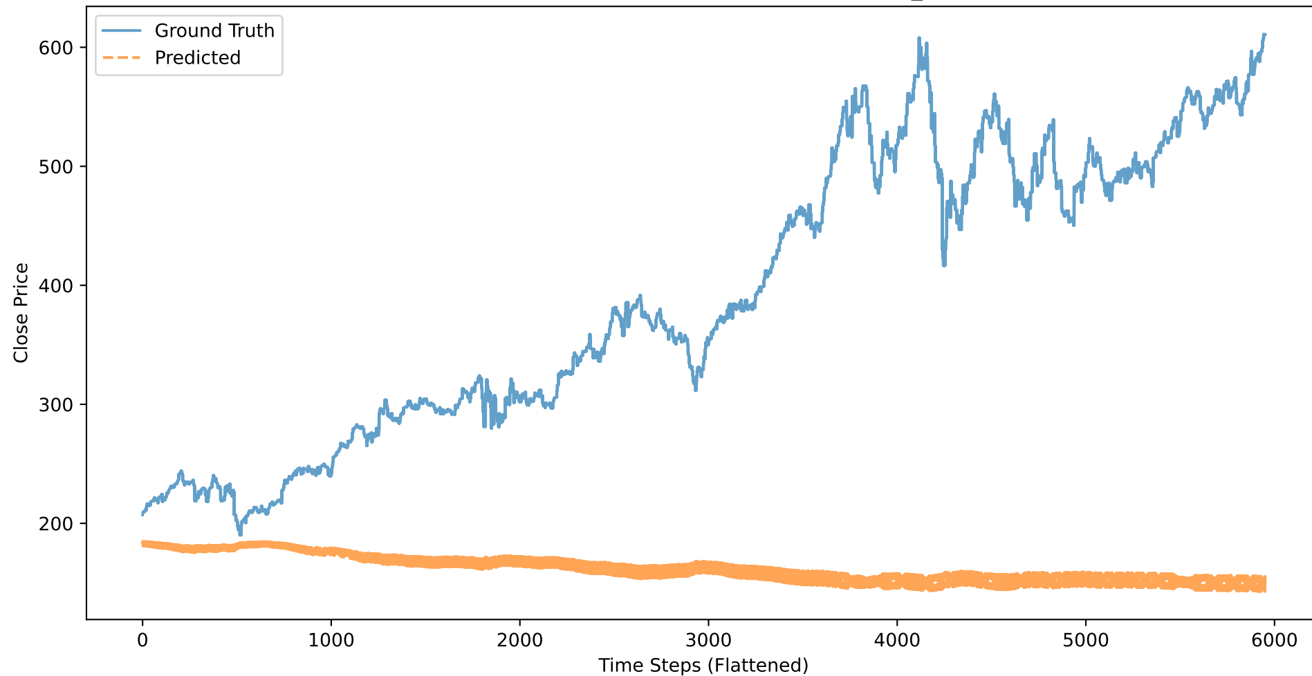
COST: Close Price - Ground Truth vs Predicted (BASELINE_CLOSE, 50 stocks)
