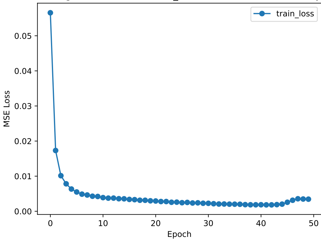
Training Loss (AAL, BASELINE_CLOSE, 50 stocks - Close Only)
