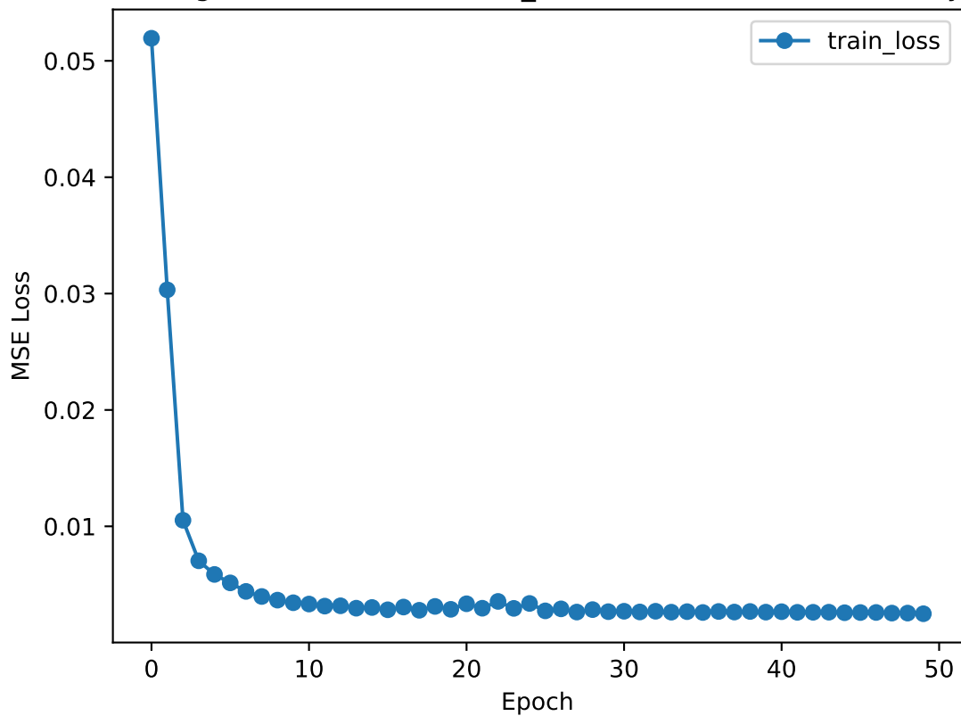
Training Loss (GLD, BASELINE_CLOSE, 50 stocks - Close Only)
