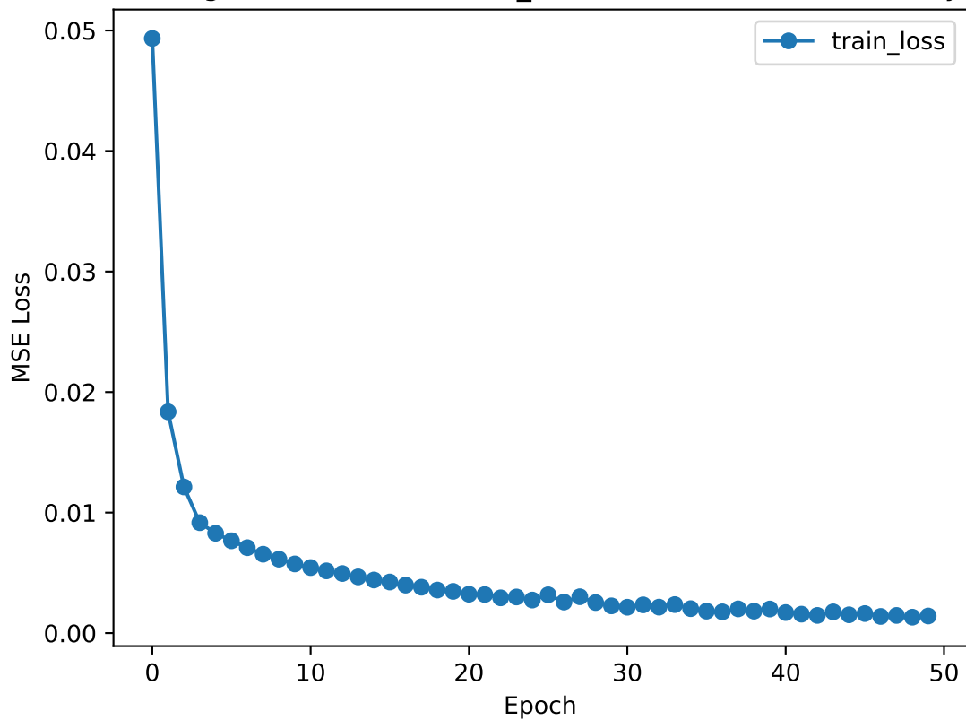
Training Loss (MU, BASELINE_CLOSE, 50 stocks - Close Only)
