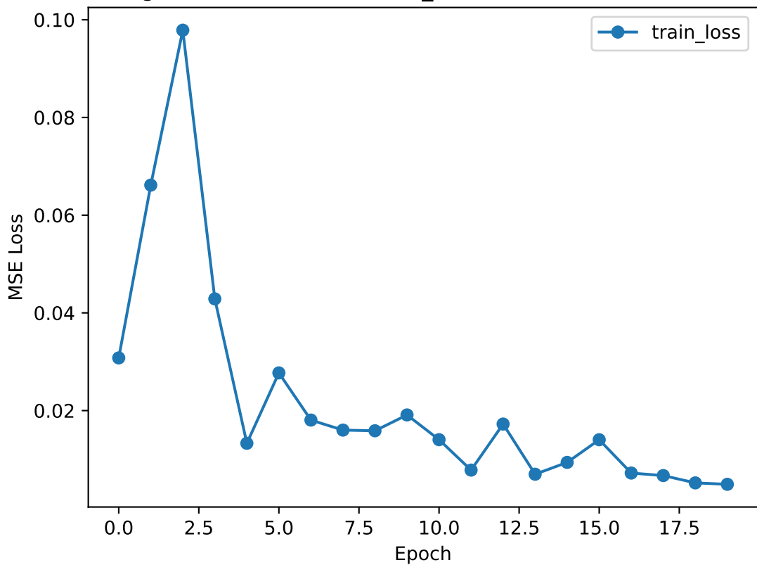
Training Loss (GOOG, BASELINE_CLOSE, 21 stocks - Close Only)
