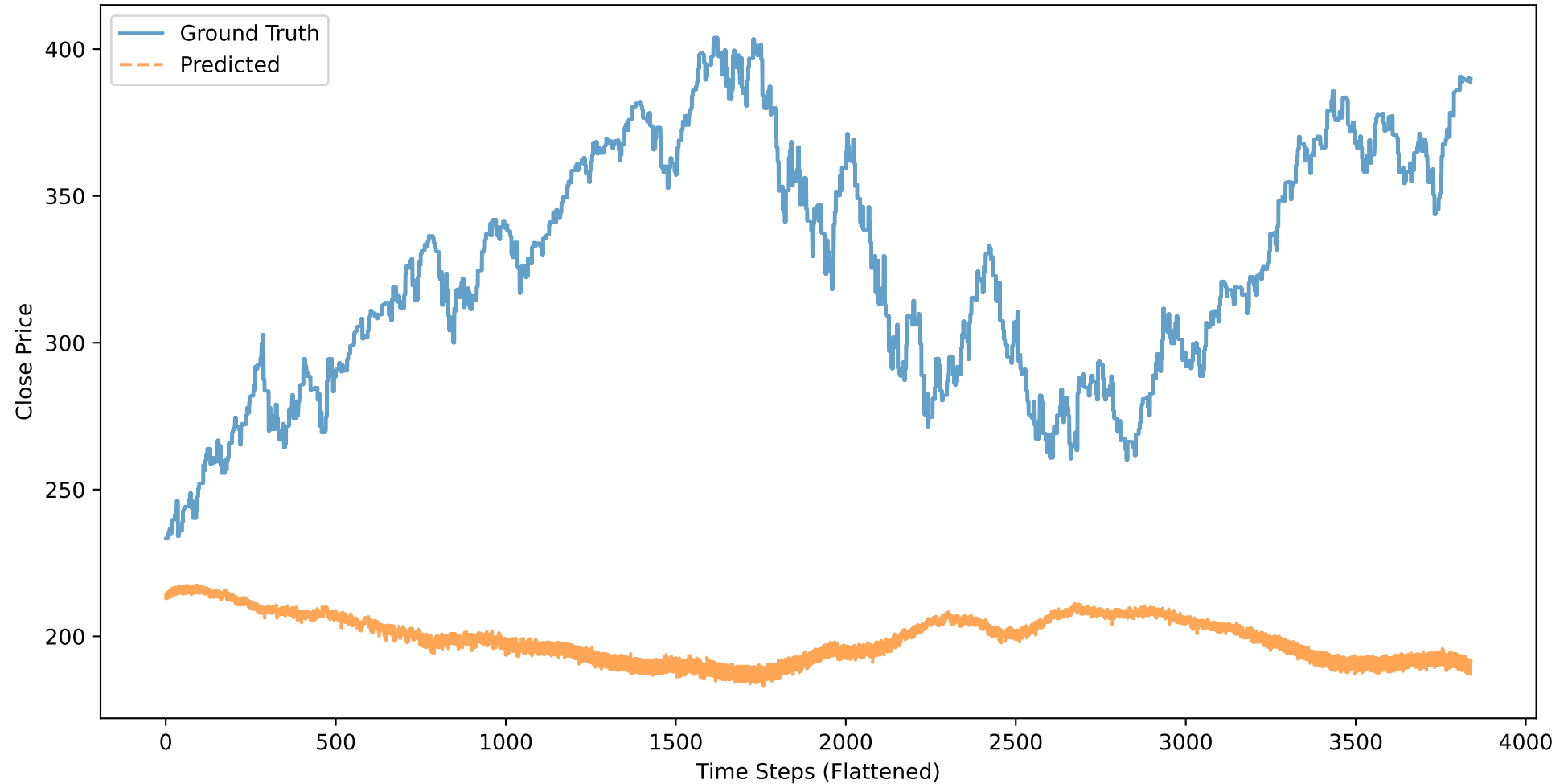
QQQ: Close Price - Ground Truth vs Predicted (BASELINE_CLOSE, 50 stocks)
