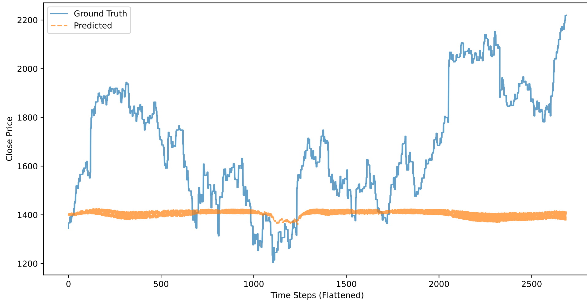
CMG: Close Price - Ground Truth vs Predicted (BASELINE_CLOSE, 50 stocks)
