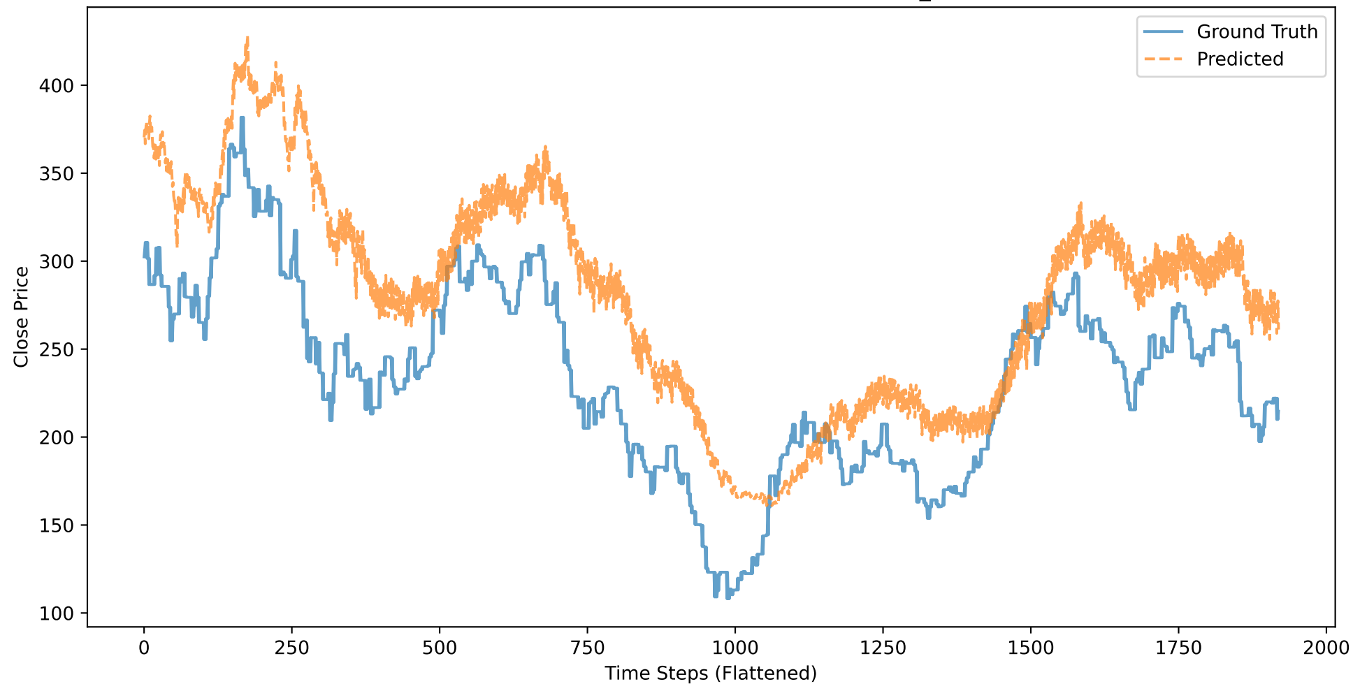
TSLA: Close Price - Ground Truth vs Predicted (BASELINE_CLOSE, 50 stocks)
