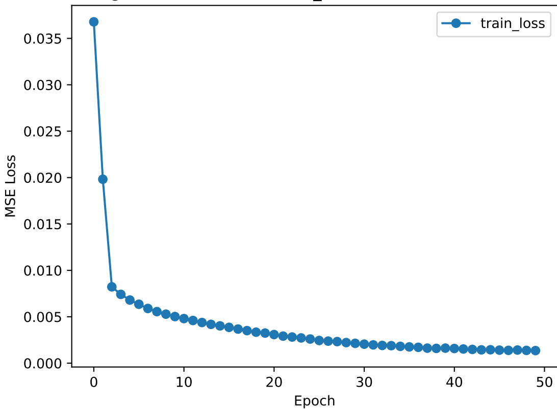
Training Loss (AMGN, BASELINE_CLOSE, 50 stocks - Close Only)
