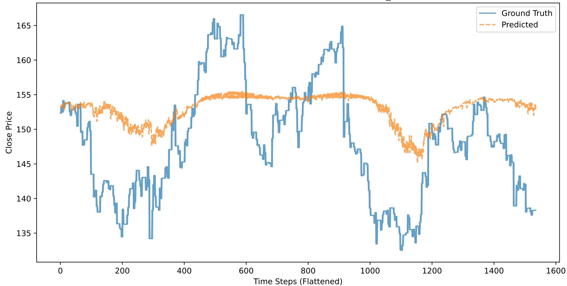
ABBV: Close Price - Ground Truth vs Predicted (BASELINE_CLOSE, 50 stocks)
