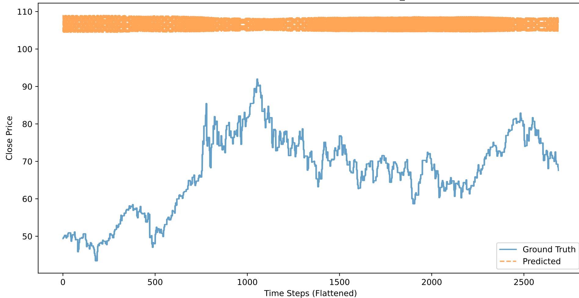
USO: Close Price - Ground Truth vs Predicted (BASELINE_CLOSE, 50 stocks)
