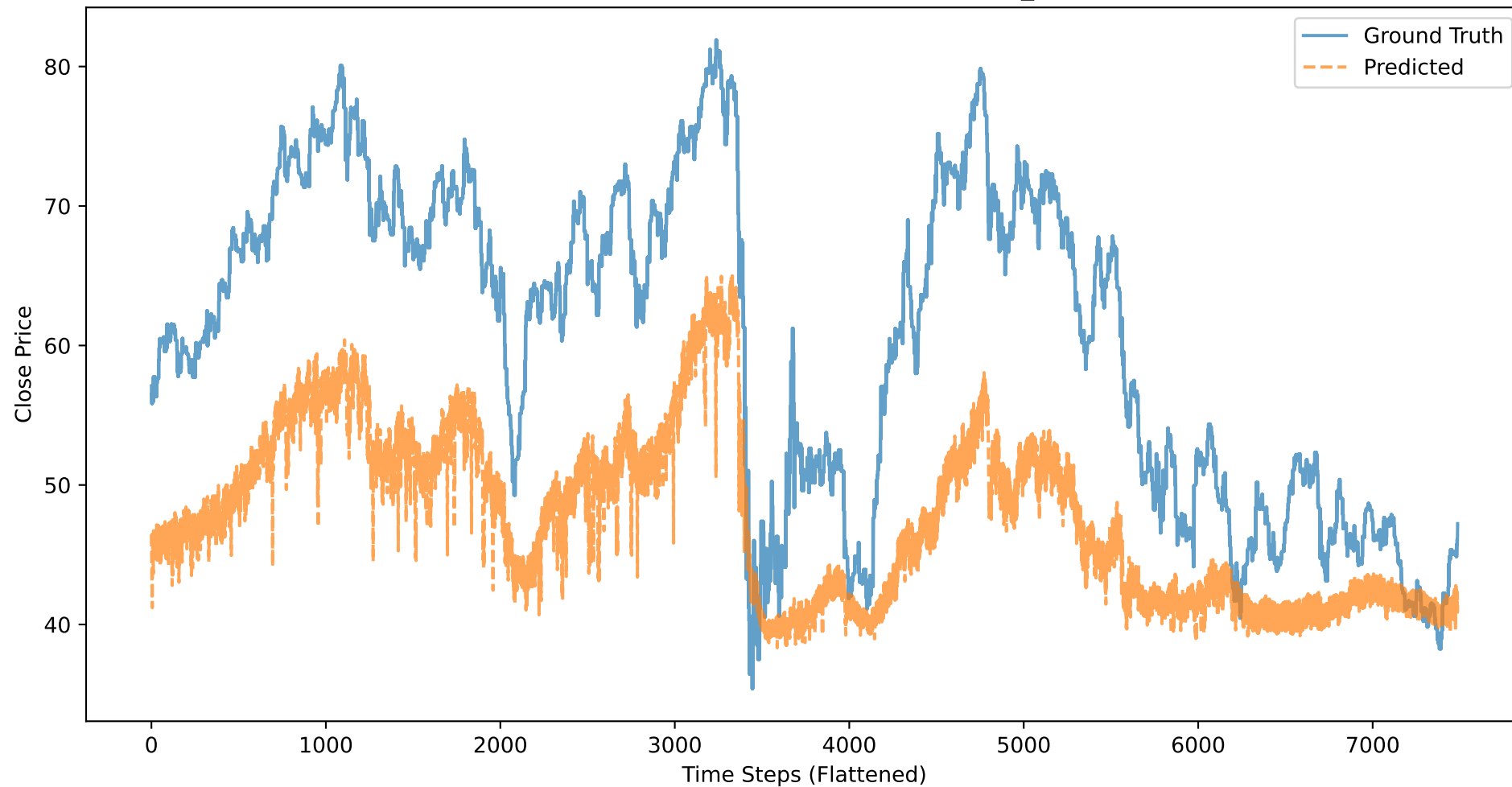
C: Close Price - Ground Truth vs Predicted (BASELINE_CLOSE, 50 stocks)
