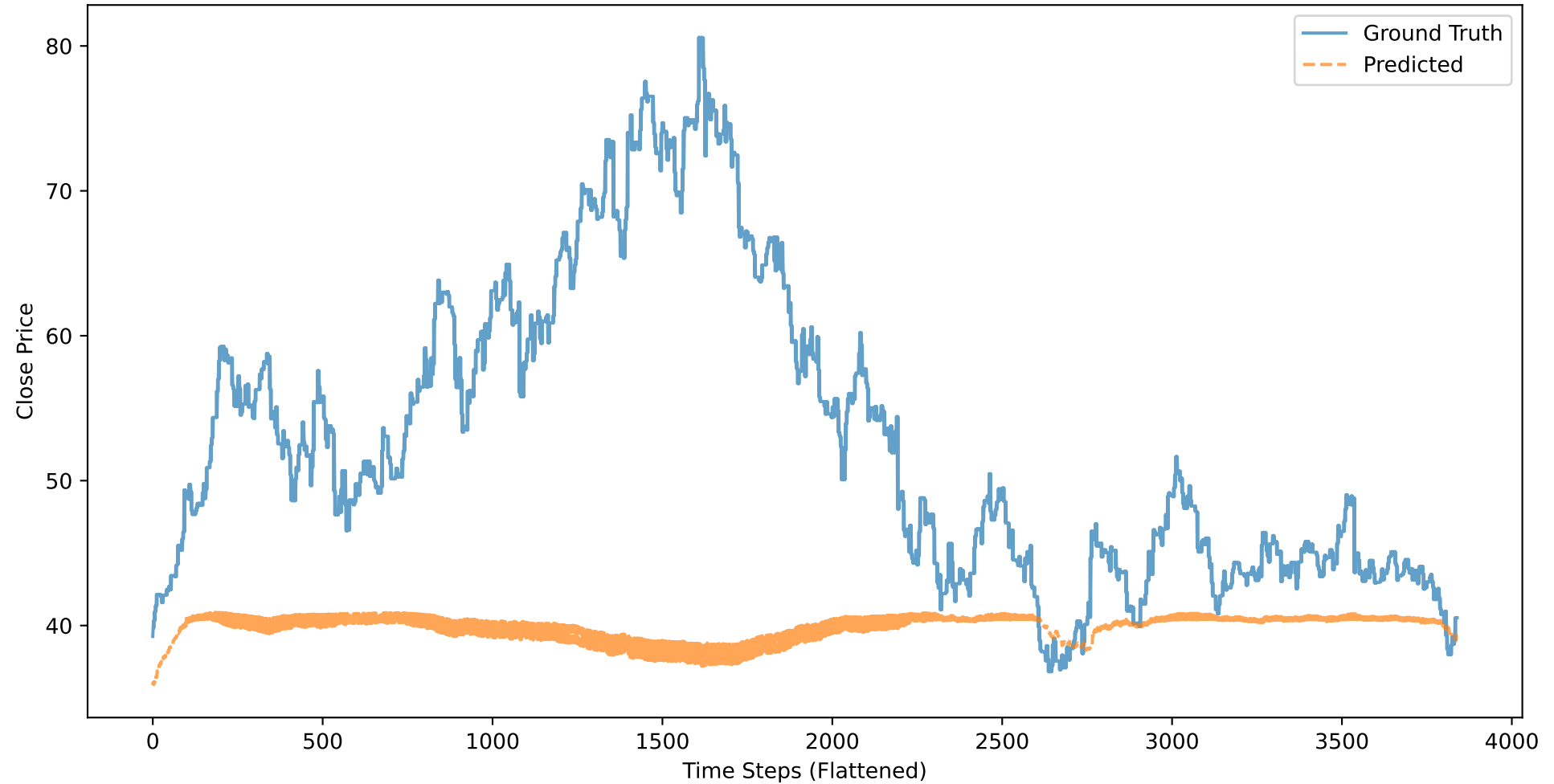
EBAY: Close Price - Ground Truth vs Predicted (BASELINE_CLOSE, 50 stocks)
