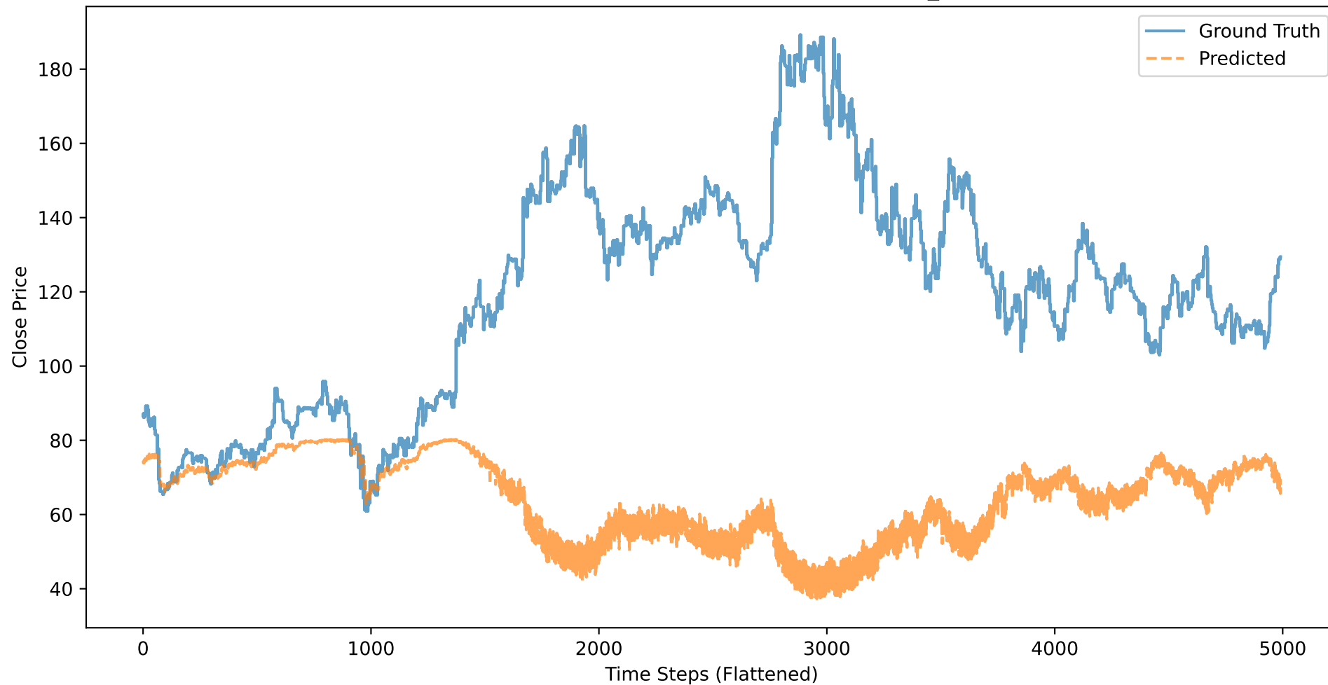
QCOM: Close Price - Ground Truth vs Predicted (BASELINE_CLOSE, 50 stocks)
