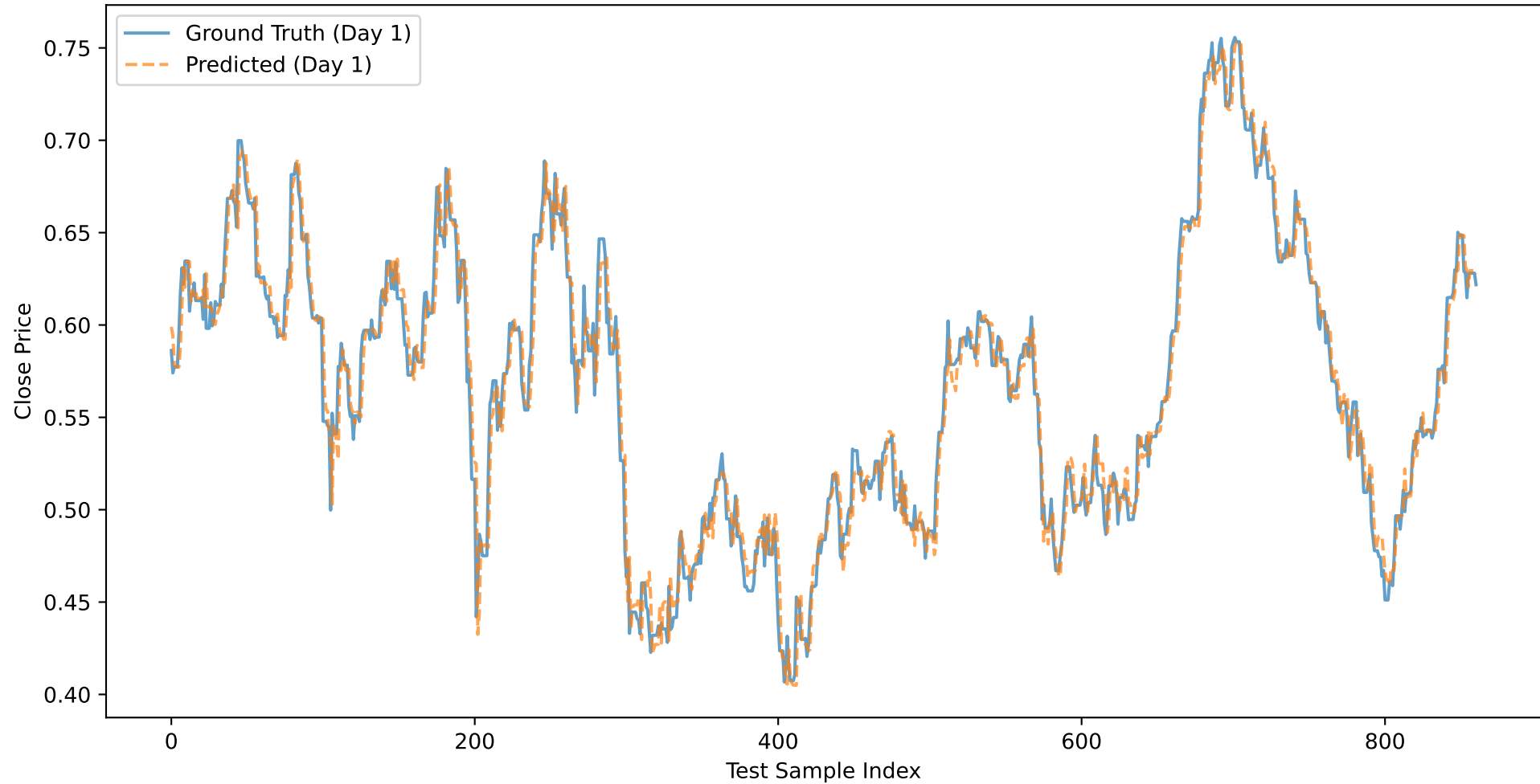
DAL: Close Price Prediction (Day 1) - BASELINE_XGB_CLOSE
