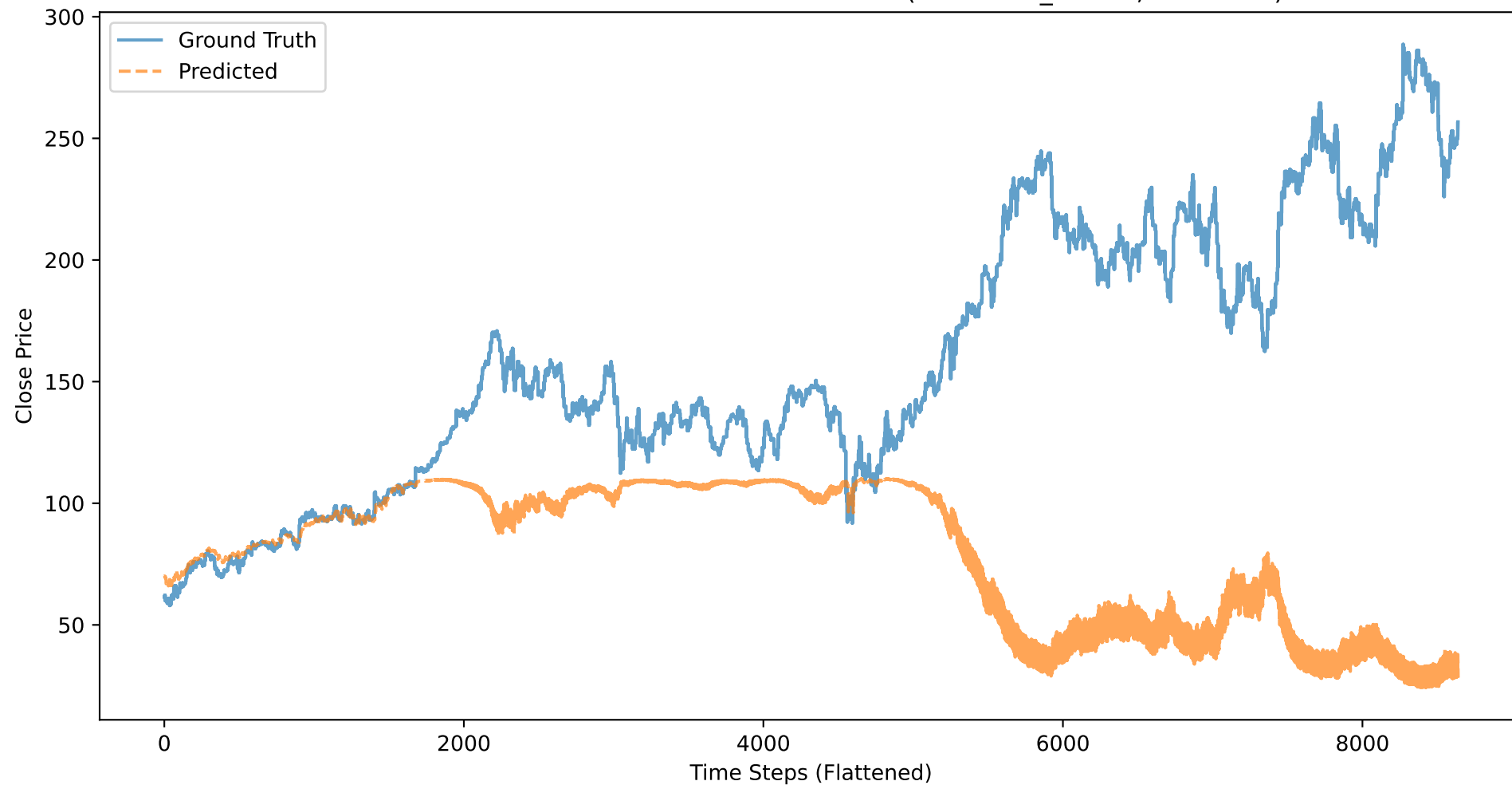
CAT: Close Price - Ground Truth vs Predicted (BASELINE_CLOSE, 50 stocks)
