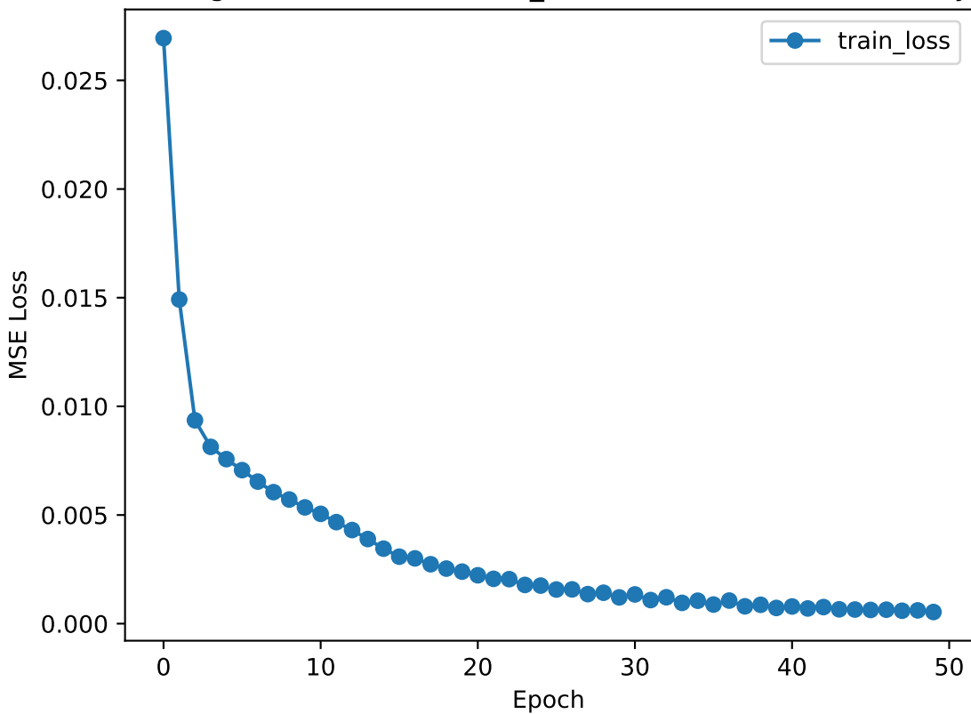
Training Loss (CAT, BASELINE_CLOSE, 50 stocks - Close Only)
