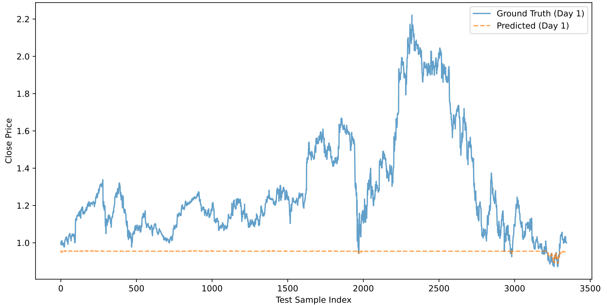
DIS: Close Price Prediction (Day 1) - NOVEL_XGB_CLOSE
