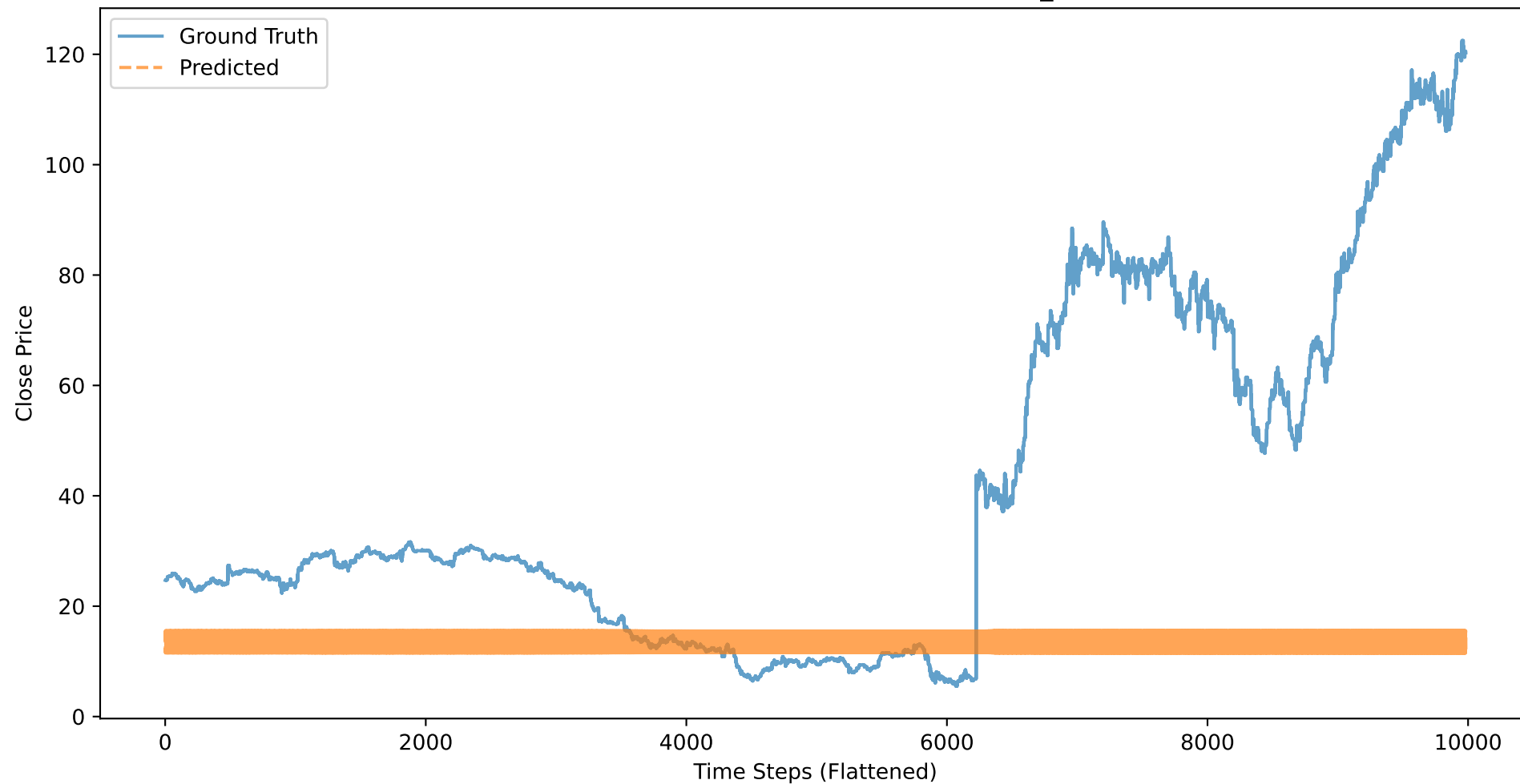
GE: Close Price - Ground Truth vs Predicted (BASELINE_CLOSE, 21 stocks)
