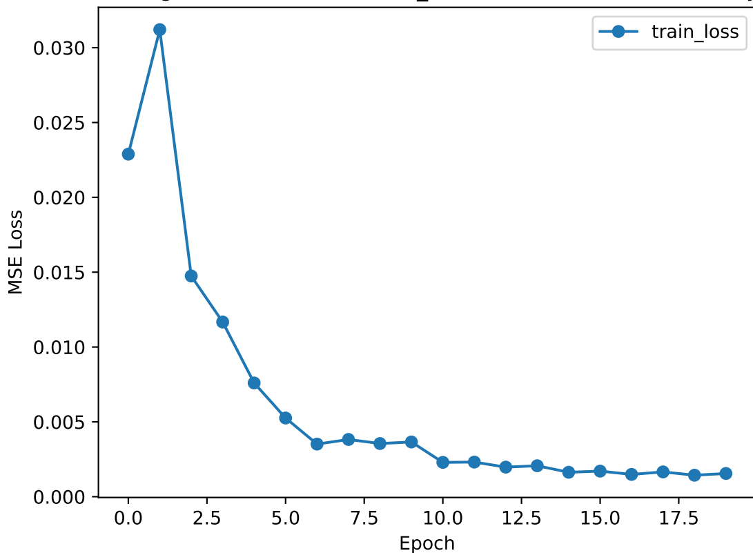
Training Loss (INTC, BASELINE_CLOSE, 21 stocks - Close Only)
