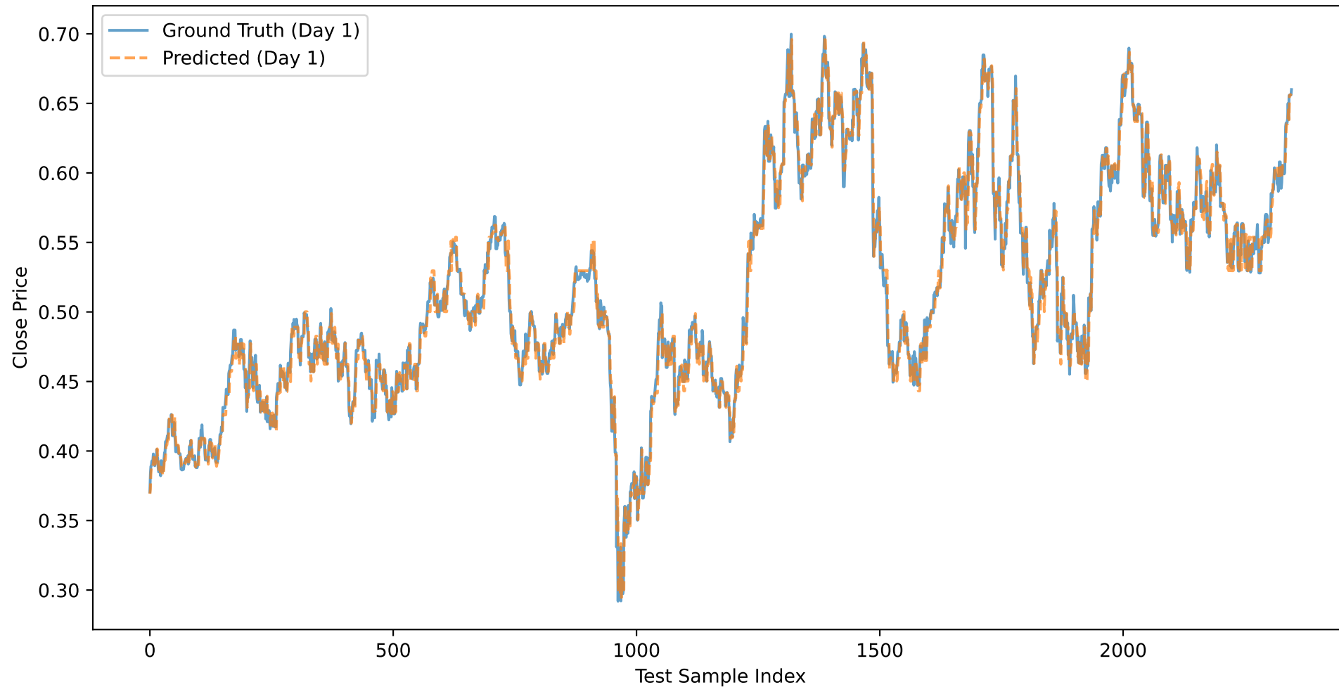
BHP: Close Price Prediction (Day 1) - BASELINE_XGB_CLOSE
