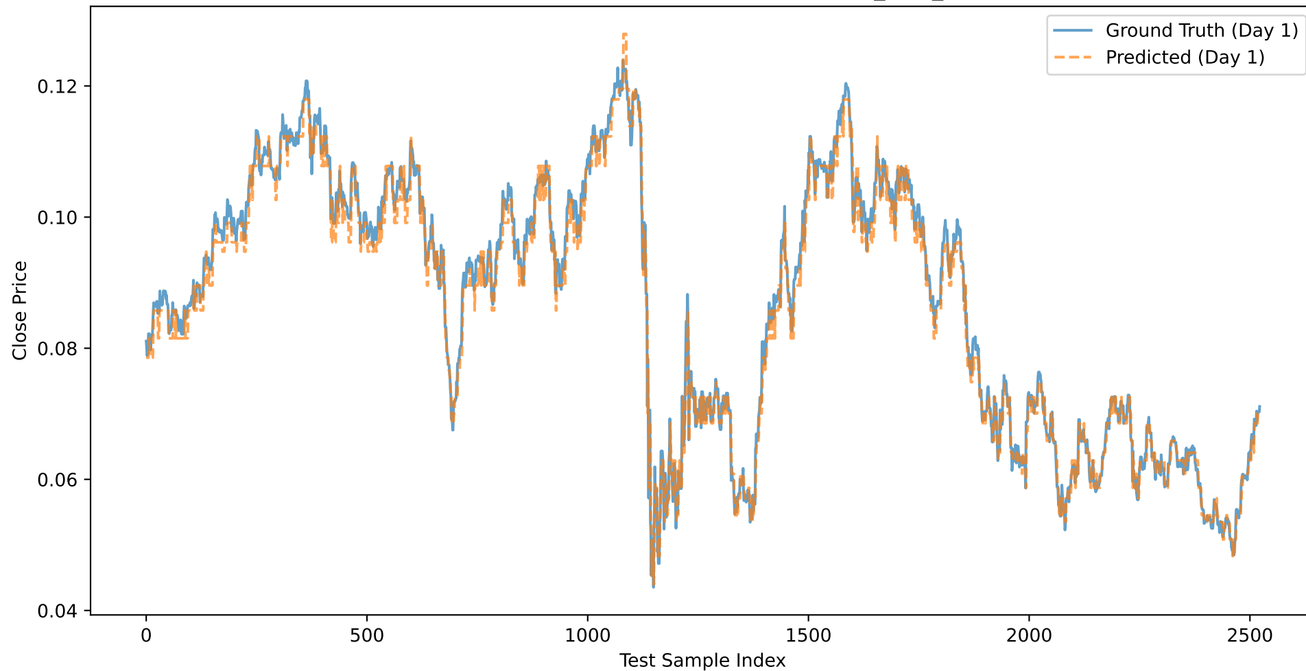
C: Close Price Prediction (Day 1) - BASELINE_XGB_CLOSE
