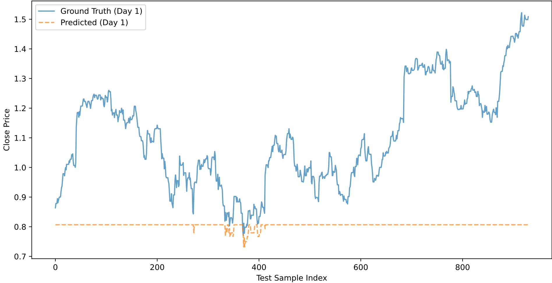
CMG: Close Price Prediction (Day 1) - BASELINE_XGB_CLOSE
