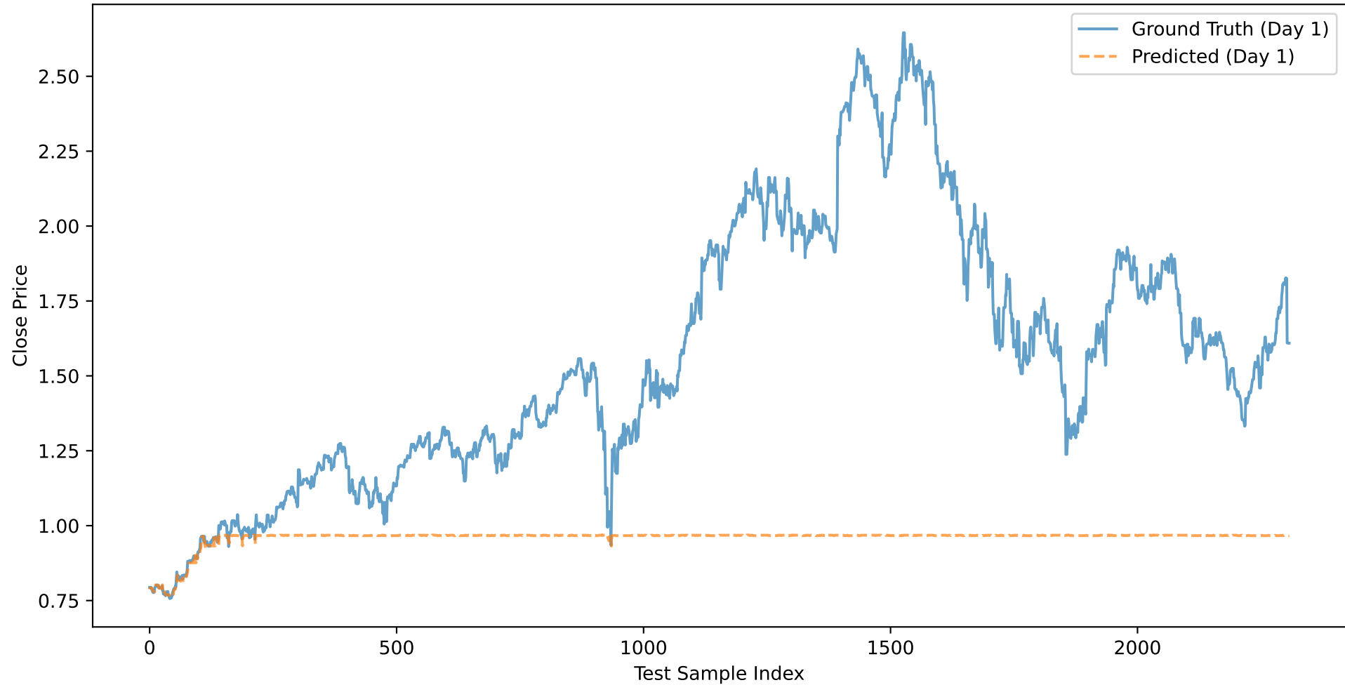
NKE: Close Price Prediction (Day 1) - BASELINE_XGB_CLOSE
