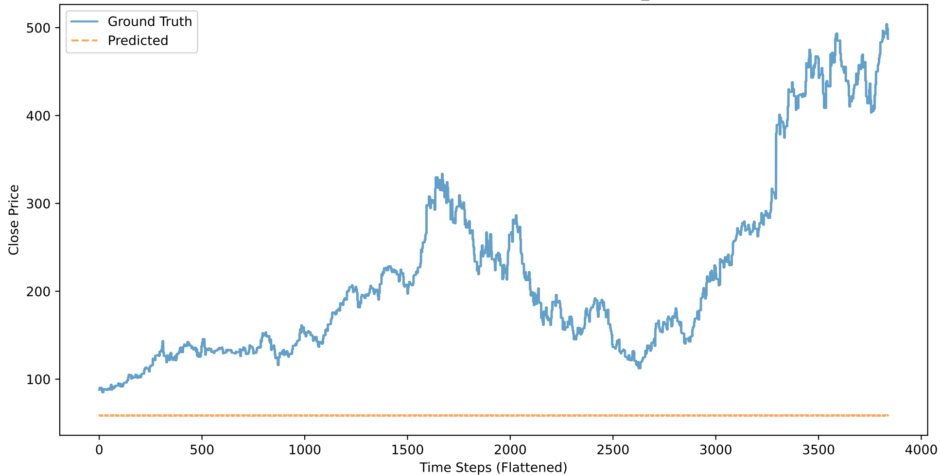
NVDA: Close Price - Ground Truth vs Predicted (BASELINE_CLOSE, 21 stocks)
