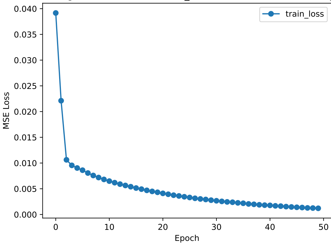
Training Loss (COST, BASELINE_CLOSE, 50 stocks - Close Only)
