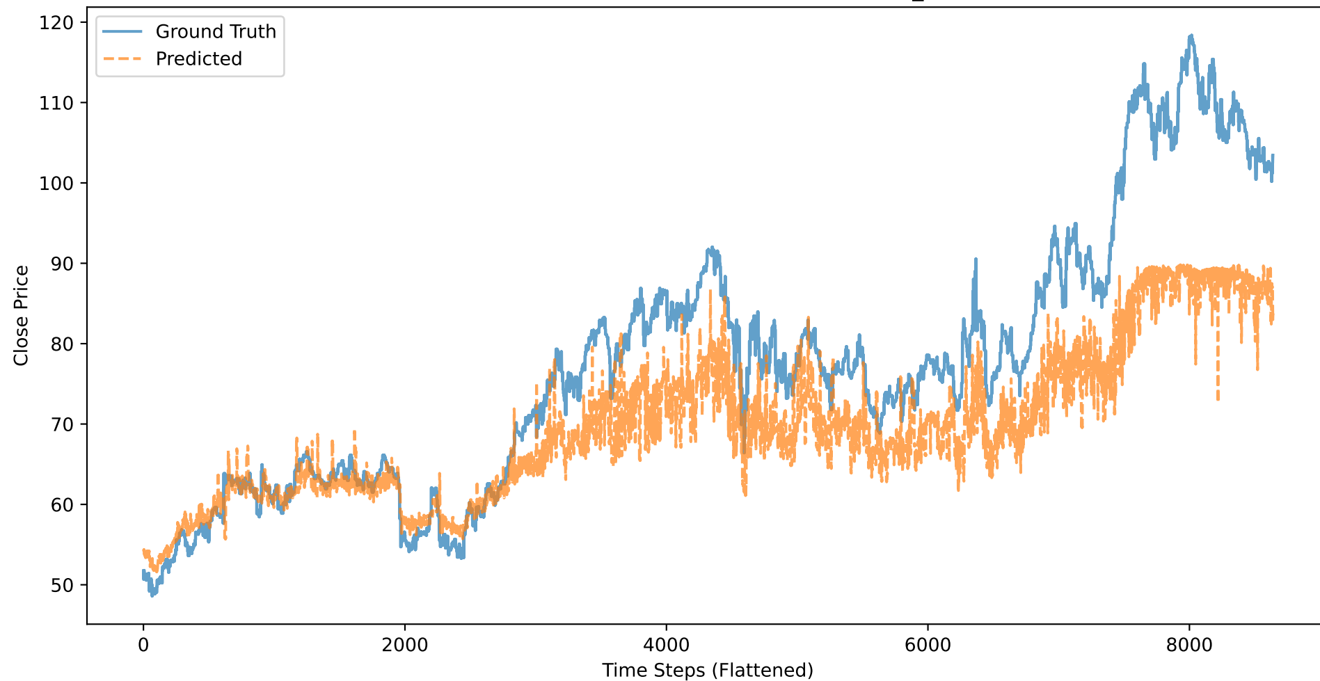
MRK: Close Price - Ground Truth vs Predicted (BASELINE_CLOSE, 50 stocks)
