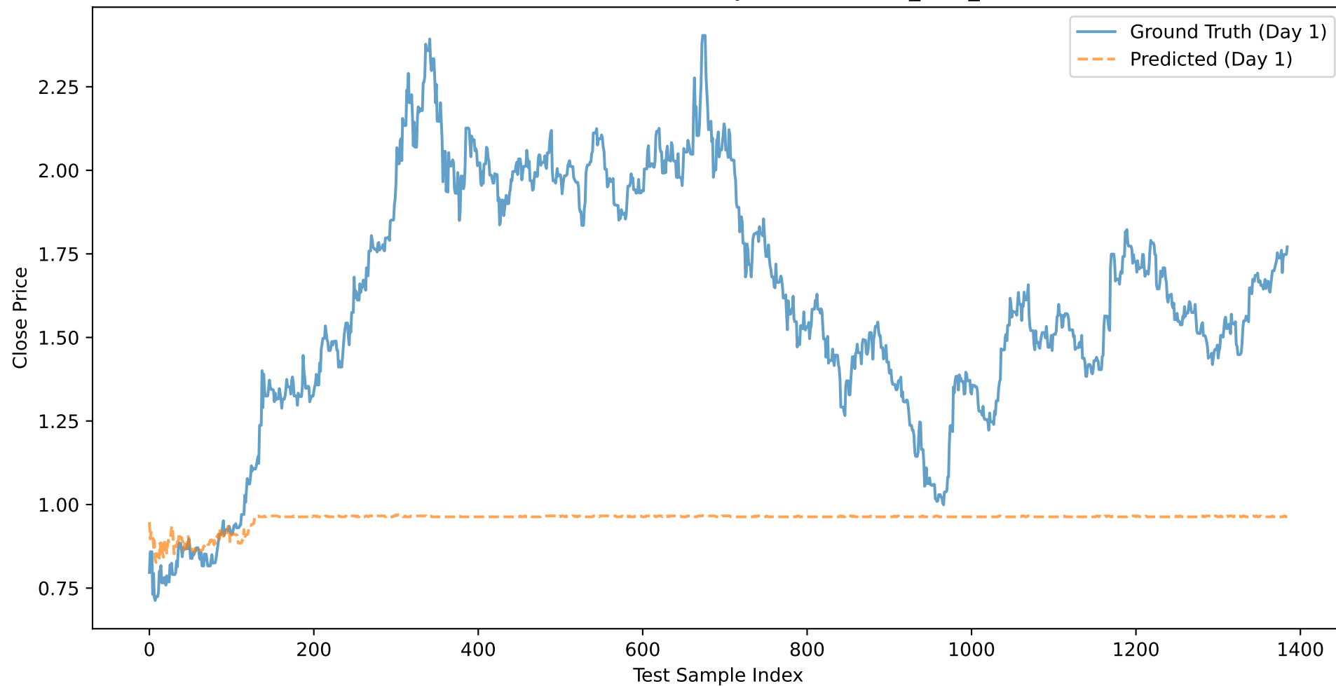
TSM: Close Price Prediction (Day 1) - BASELINE_XGB_CLOSE
