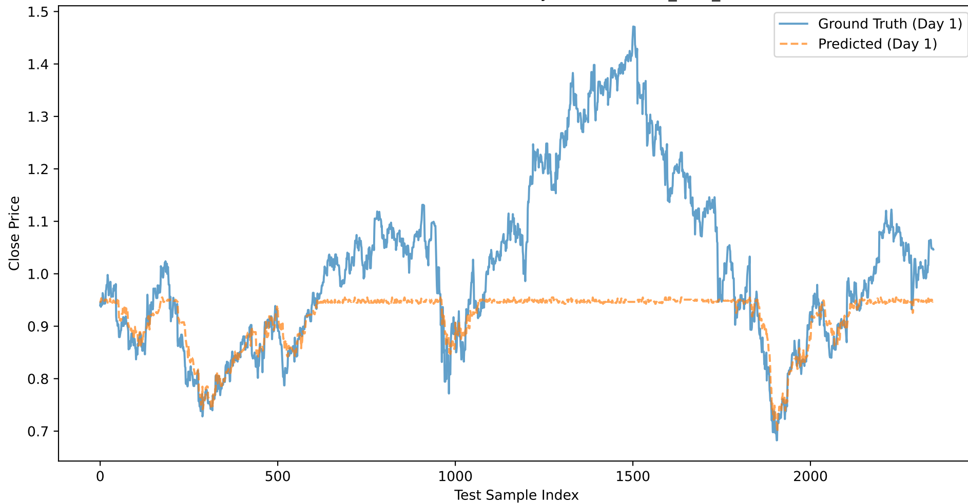
CMCSA: Close Price Prediction (Day 1) - BASELINE_XGB_CLOSE
