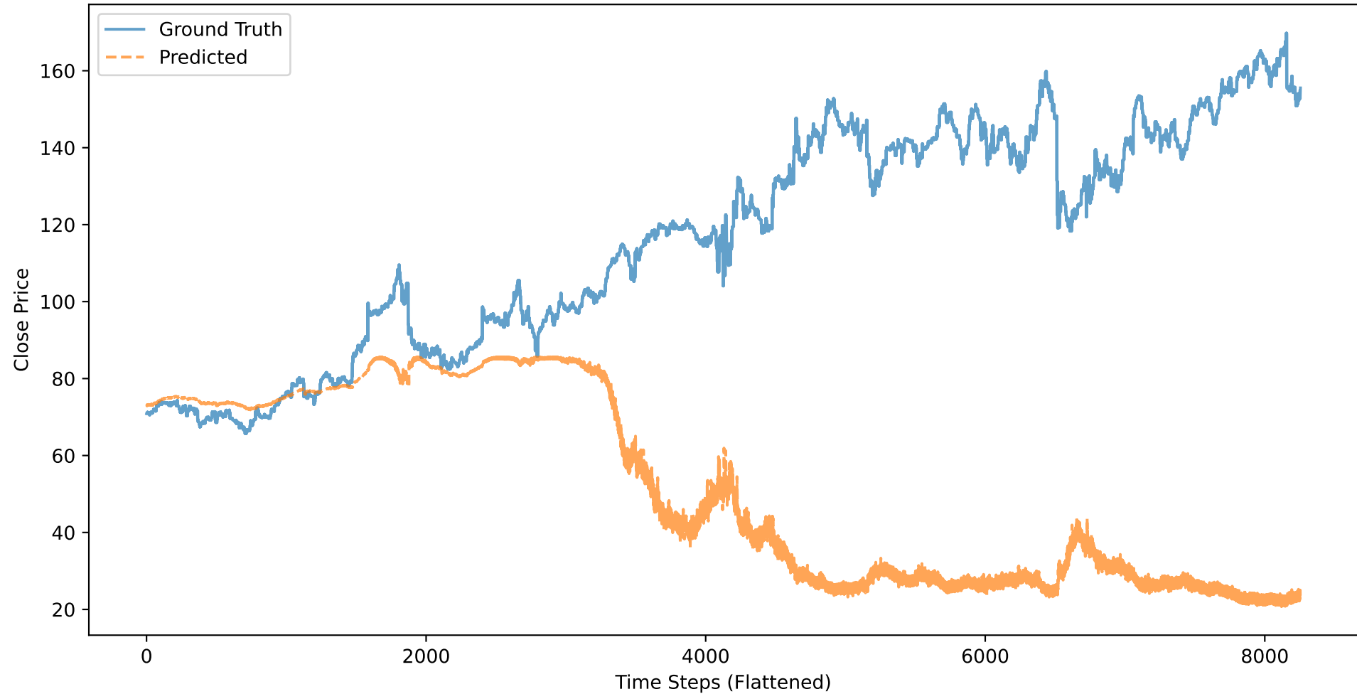
WMT: Close Price - Ground Truth vs Predicted (BASELINE_CLOSE, 50 stocks)
