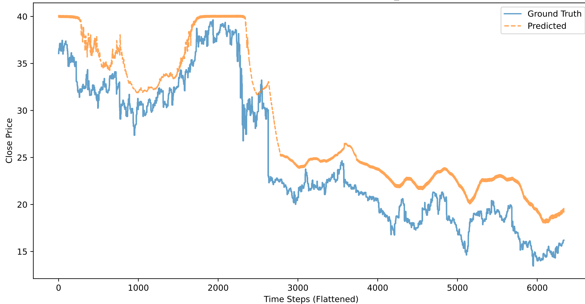
T: Close Price - Ground Truth vs Predicted (BASELINE_CLOSE, 21 stocks)
