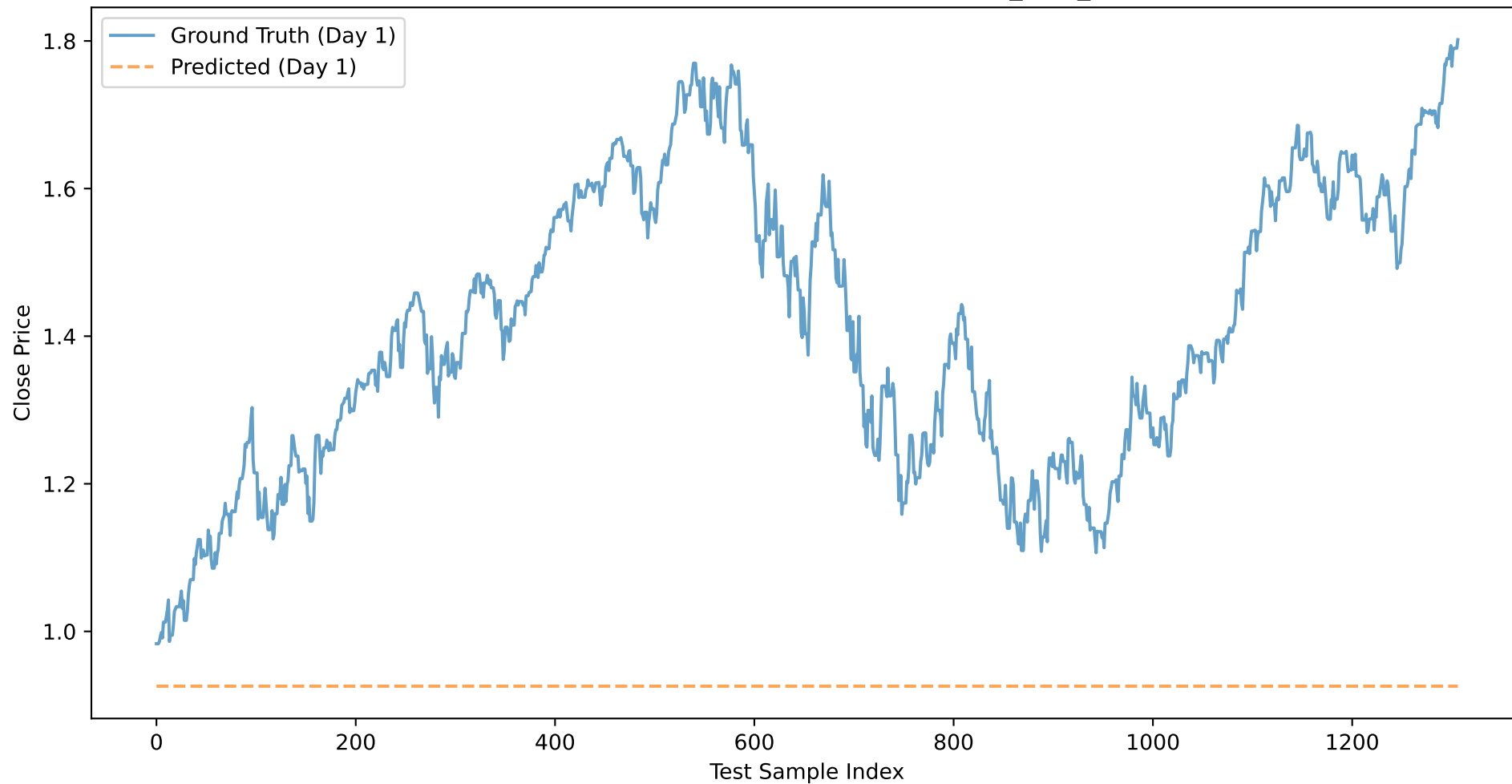
QQQ: Close Price Prediction (Day 1) - NOVEL_XGB_CLOSE
