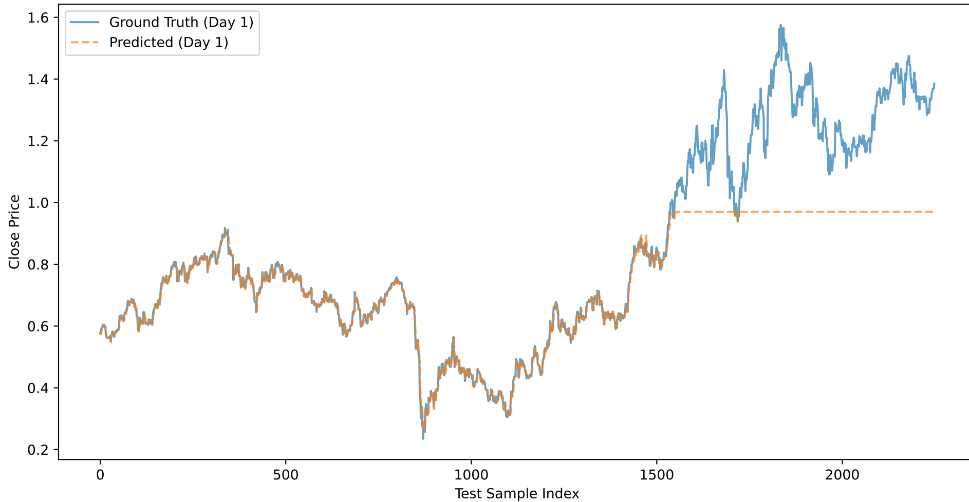
COP: Close Price Prediction (Day 1) - NOVEL_XGB_CLOSE
