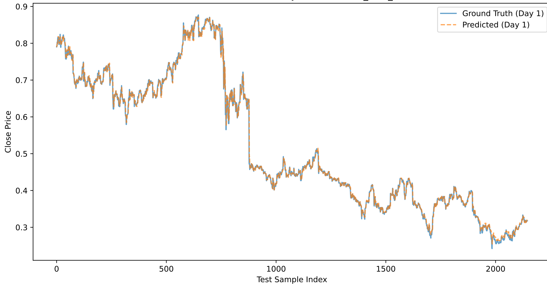
T: Close Price Prediction (Day 1) - BASELINE_XGB_CLOSE
