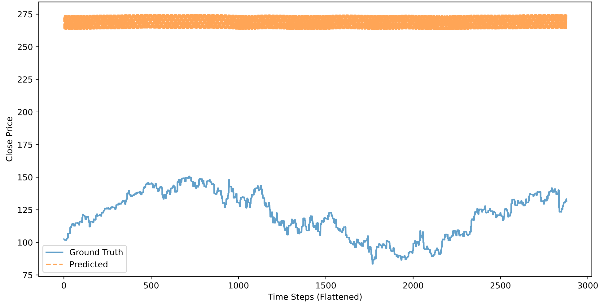
GOOG: Close Price - Ground Truth vs Predicted (BASELINE_CLOSE, 21 stocks)
