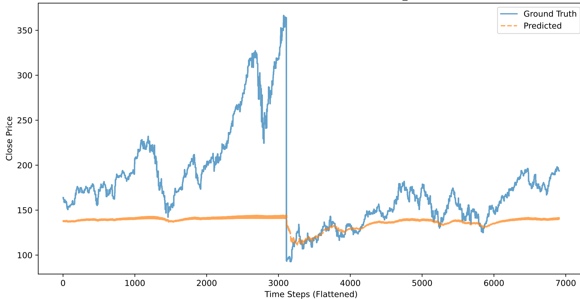
AAPL: Close Price - Ground Truth vs Predicted (BASELINE_CLOSE, 50 stocks)
