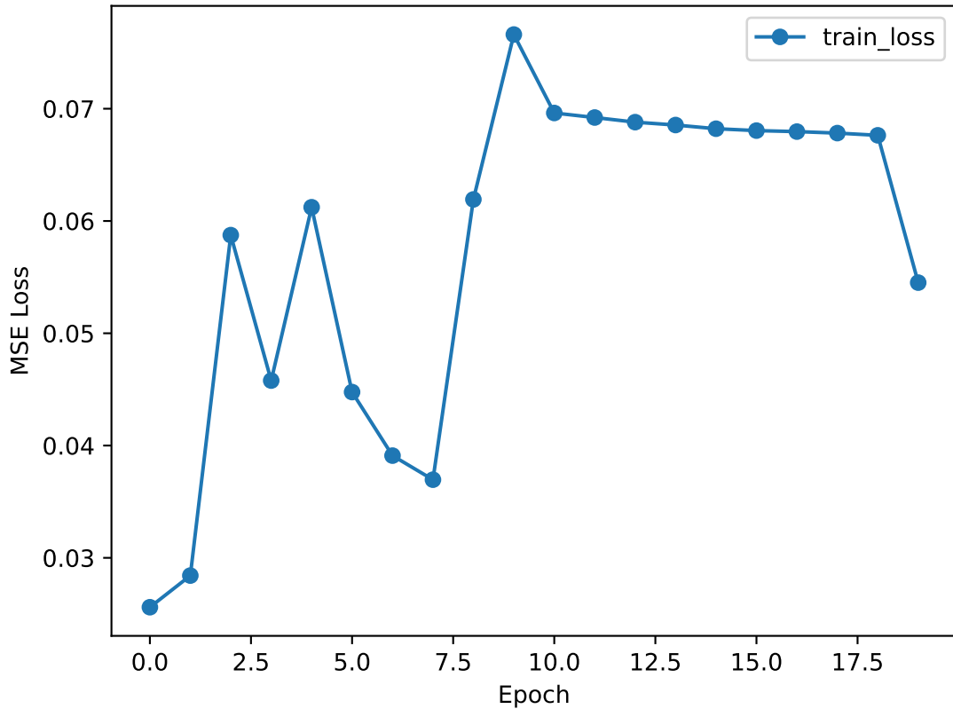
Training Loss (BHP, BASELINE_CLOSE, 21 stocks - Close Only)
