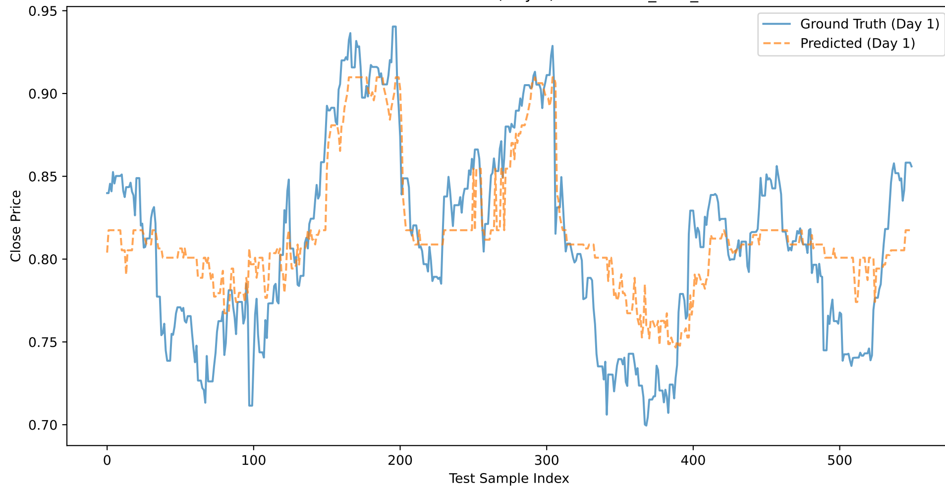
ABBV: Close Price Prediction (Day 1) - BASELINE_XGB_CLOSE
