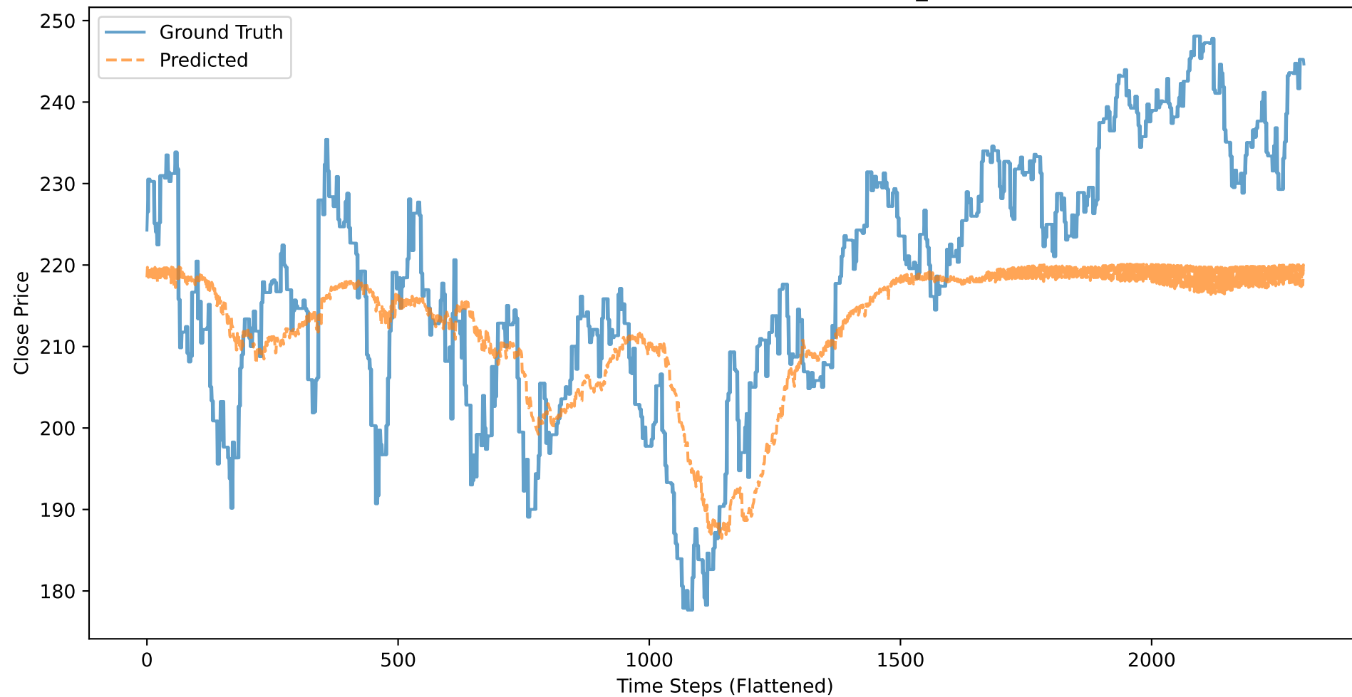
V: Close Price - Ground Truth vs Predicted (BASELINE_CLOSE, 50 stocks)
