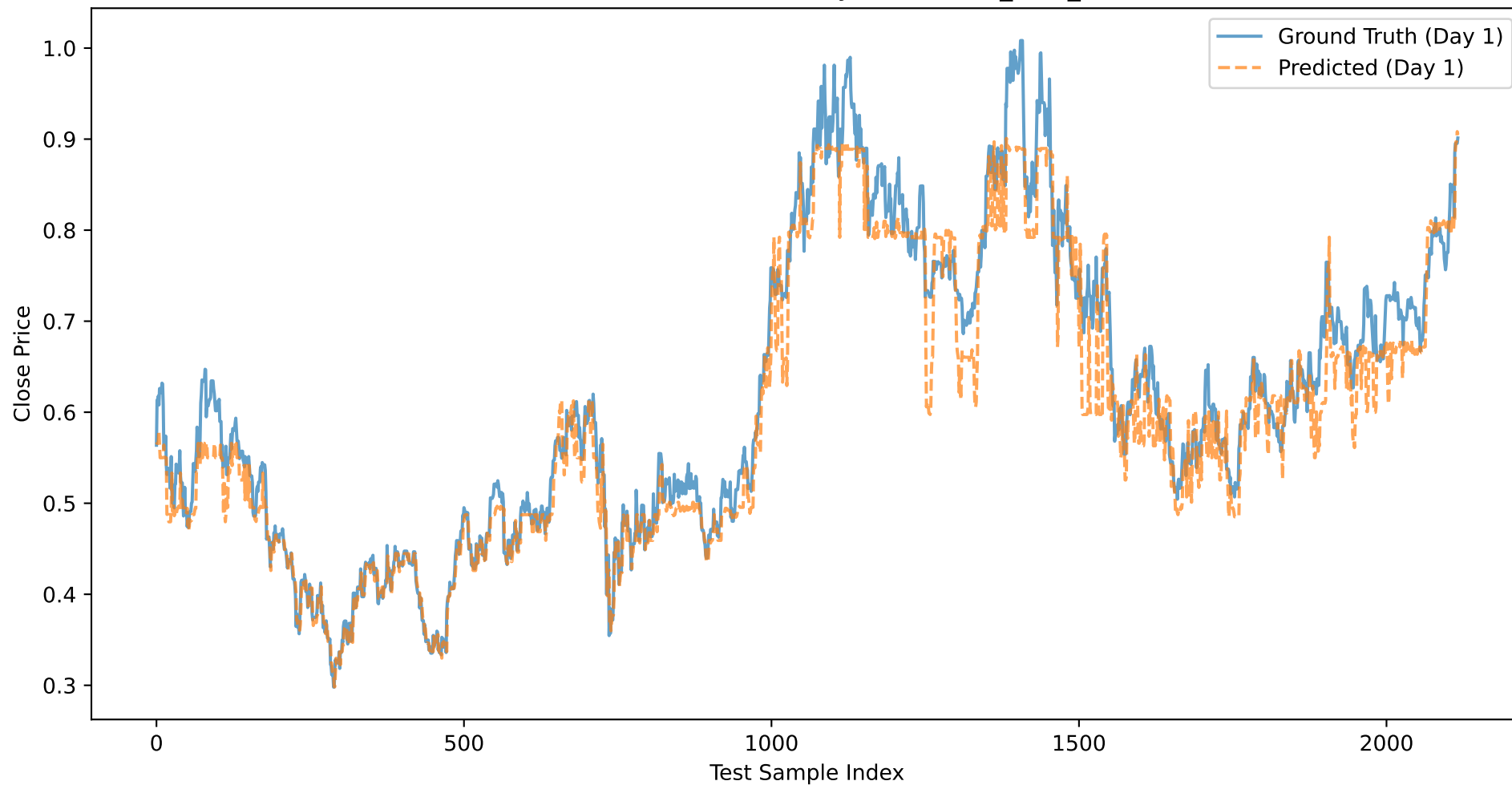
MU: Close Price Prediction (Day 1) - NOVEL_XGB_CLOSE
