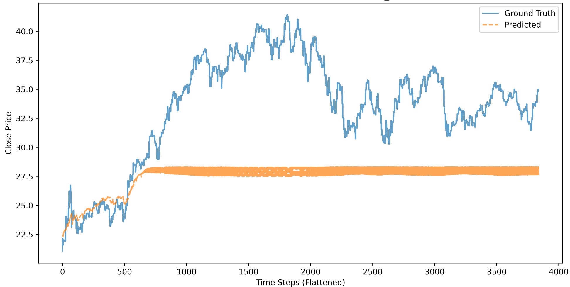
XLF: Close Price - Ground Truth vs Predicted (BASELINE_CLOSE, 50 stocks)
