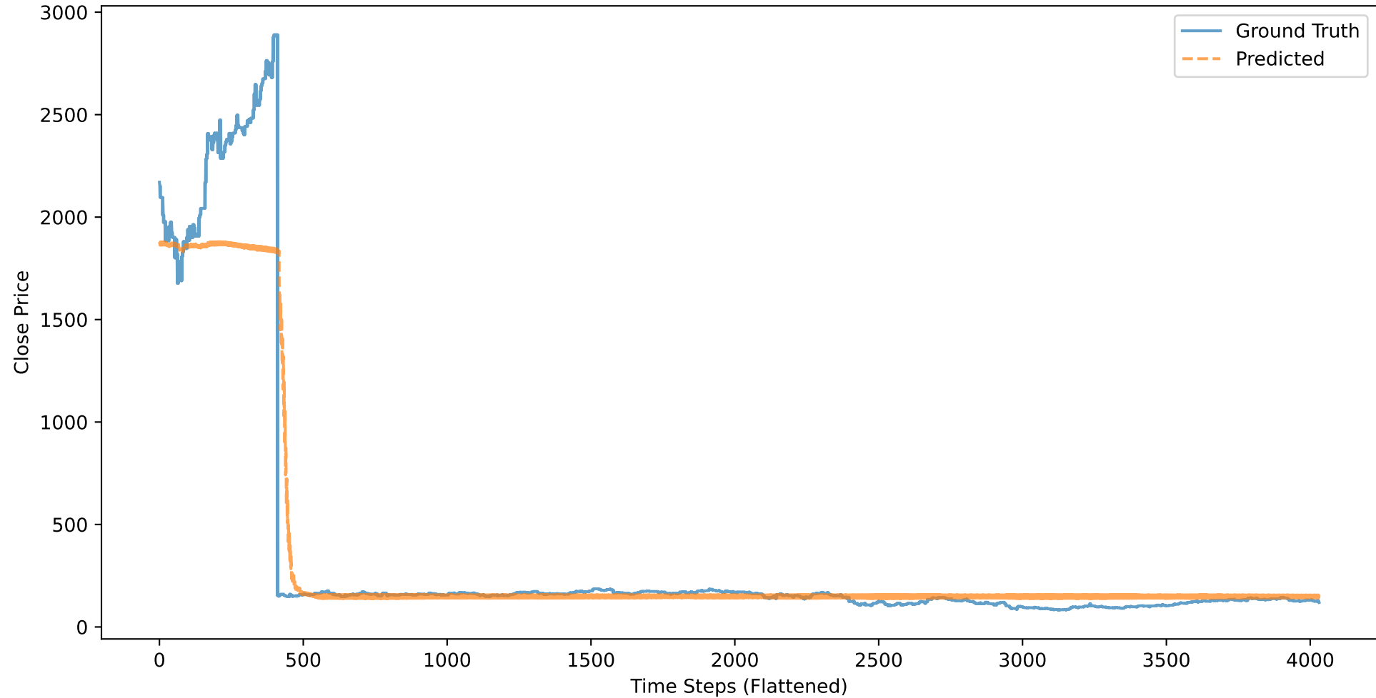
AMZN: Close Price - Ground Truth vs Predicted (BASELINE_CLOSE, 50 stocks)
