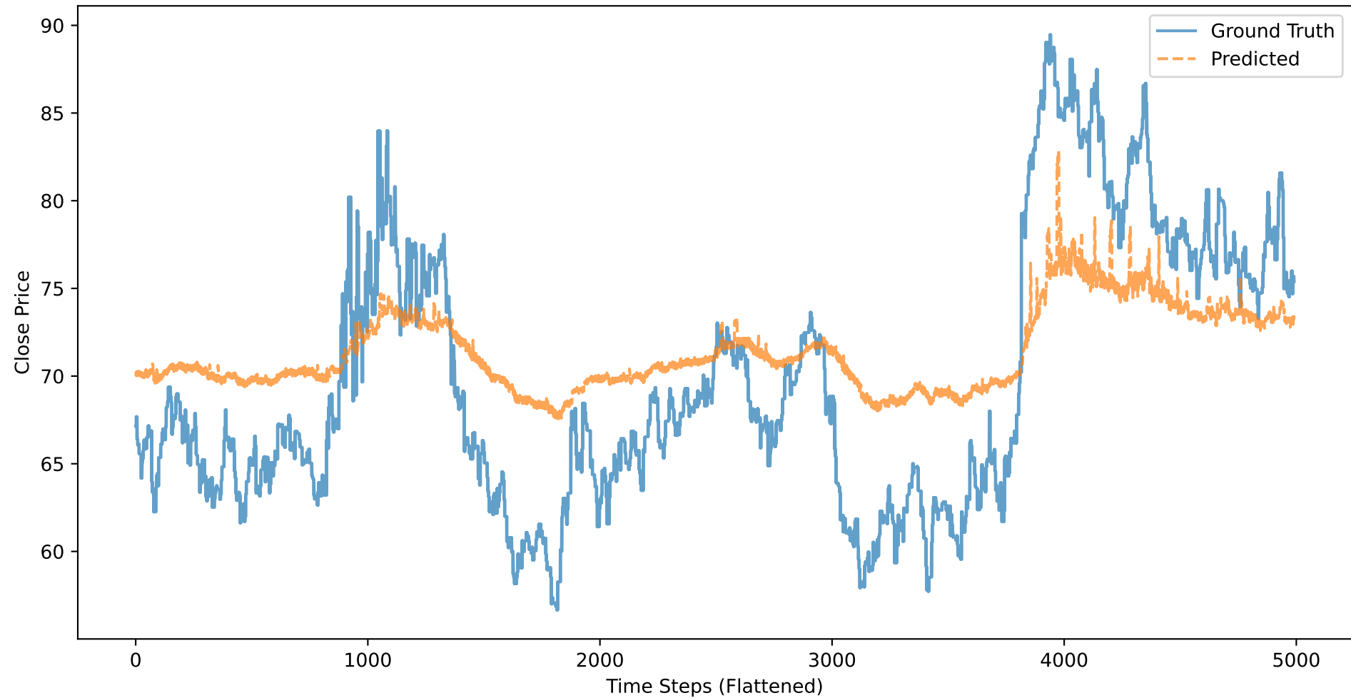
GILD: Close Price - Ground Truth vs Predicted (BASELINE_CLOSE, 50 stocks)
