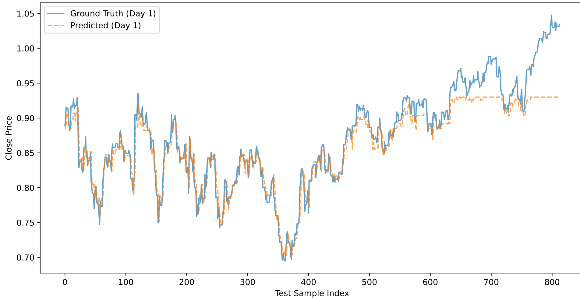
V: Close Price Prediction (Day 1) - BASELINE_XGB_CLOSE
