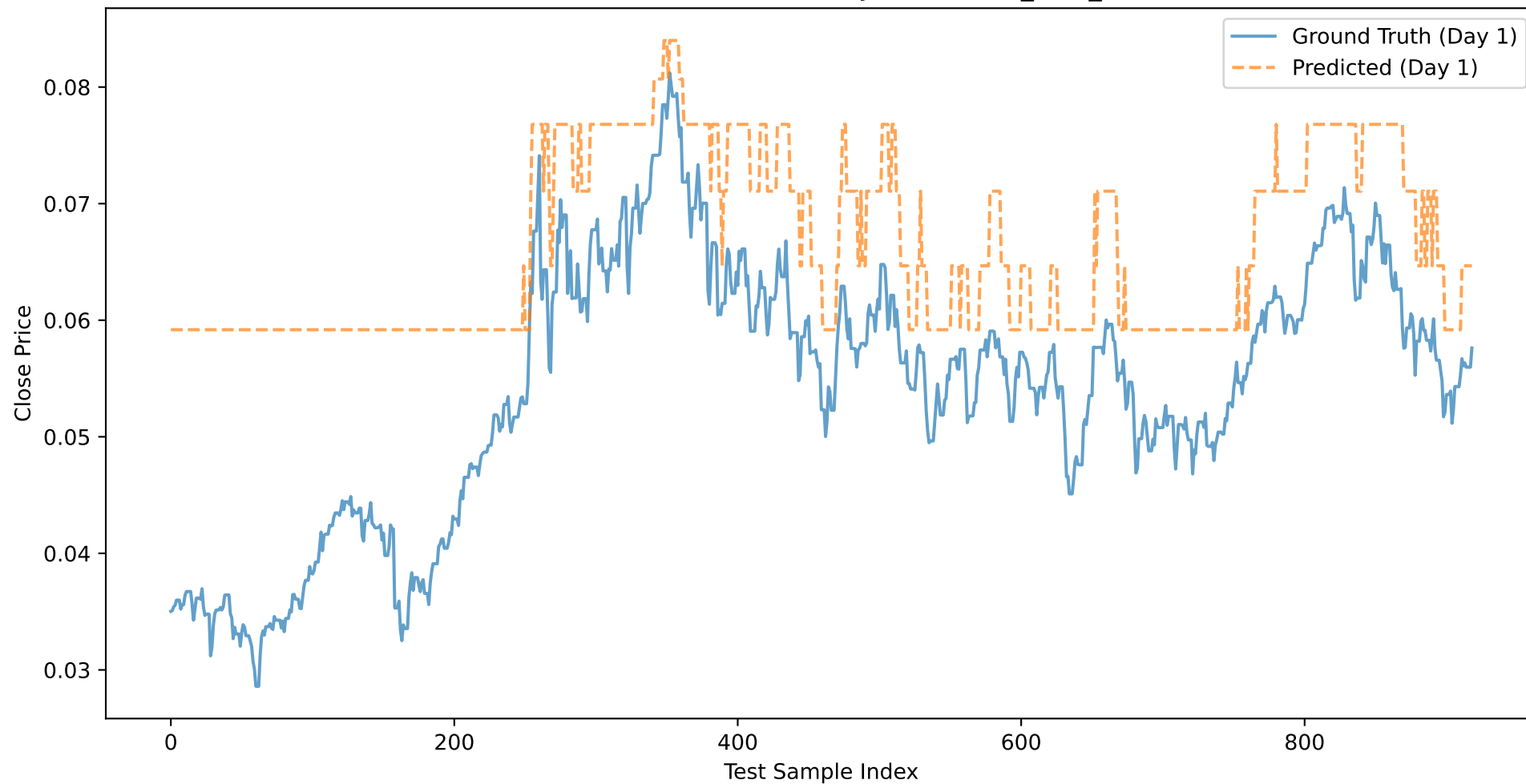
USO: Close Price Prediction (Day 1) - NOVEL_XGB_CLOSE
