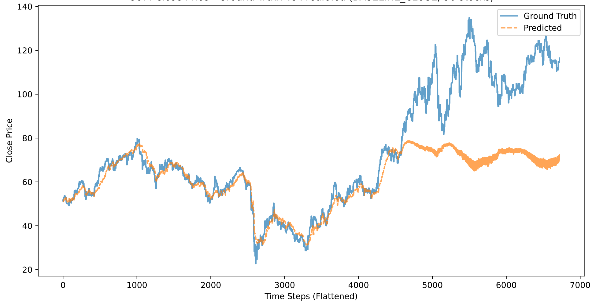
COP: Close Price - Ground Truth vs Predicted (BASELINE_CLOSE, 50 stocks)
