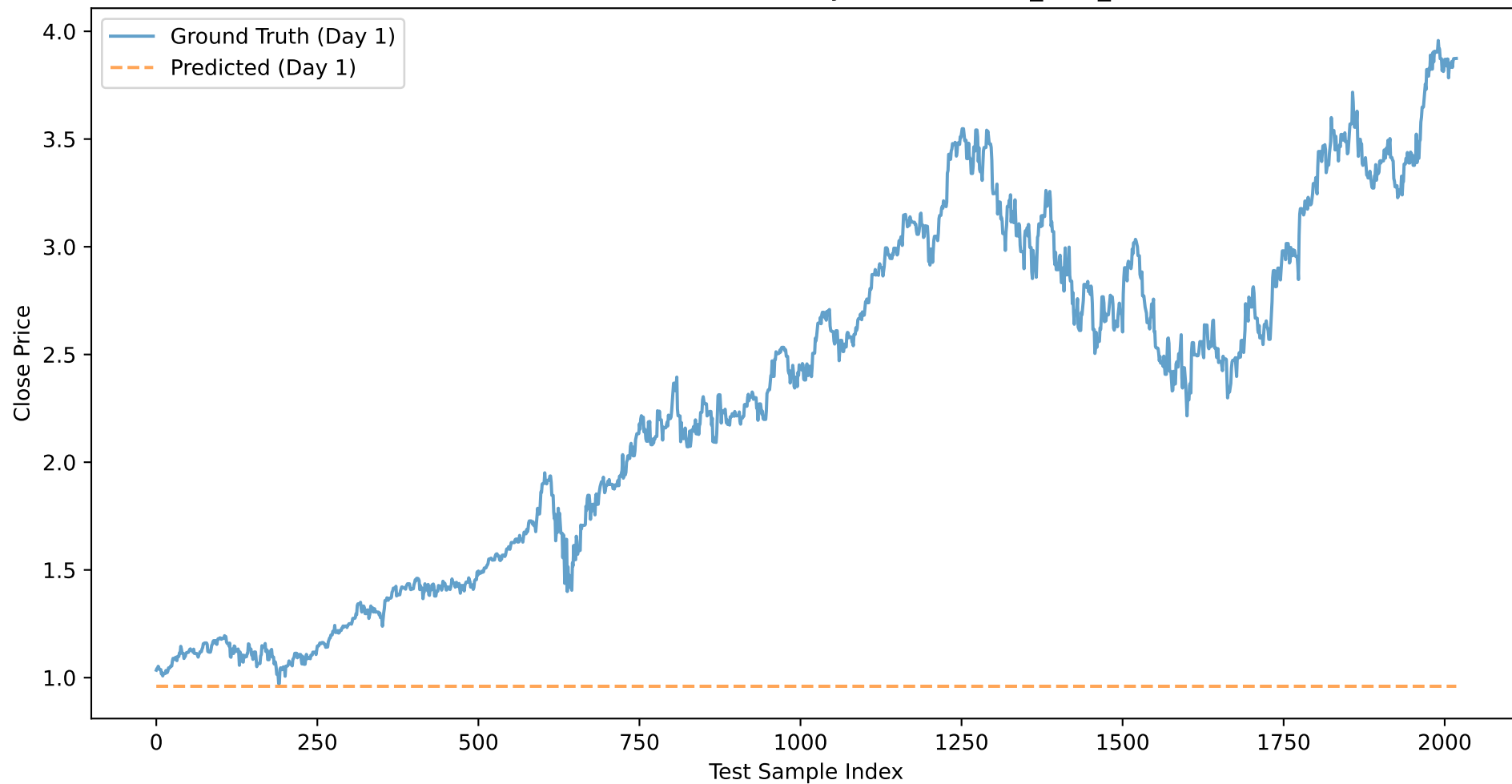
MSFT: Close Price Prediction (Day 1) - BASELINE_XGB_CLOSE
