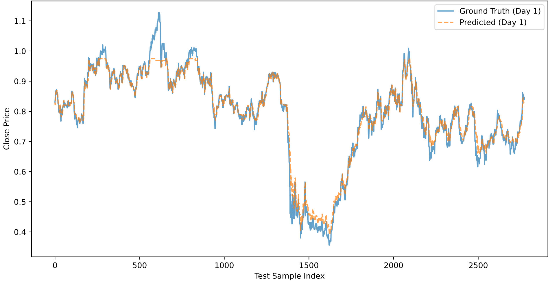
WFC: Close Price Prediction (Day 1) - BASELINE_XGB_CLOSE
