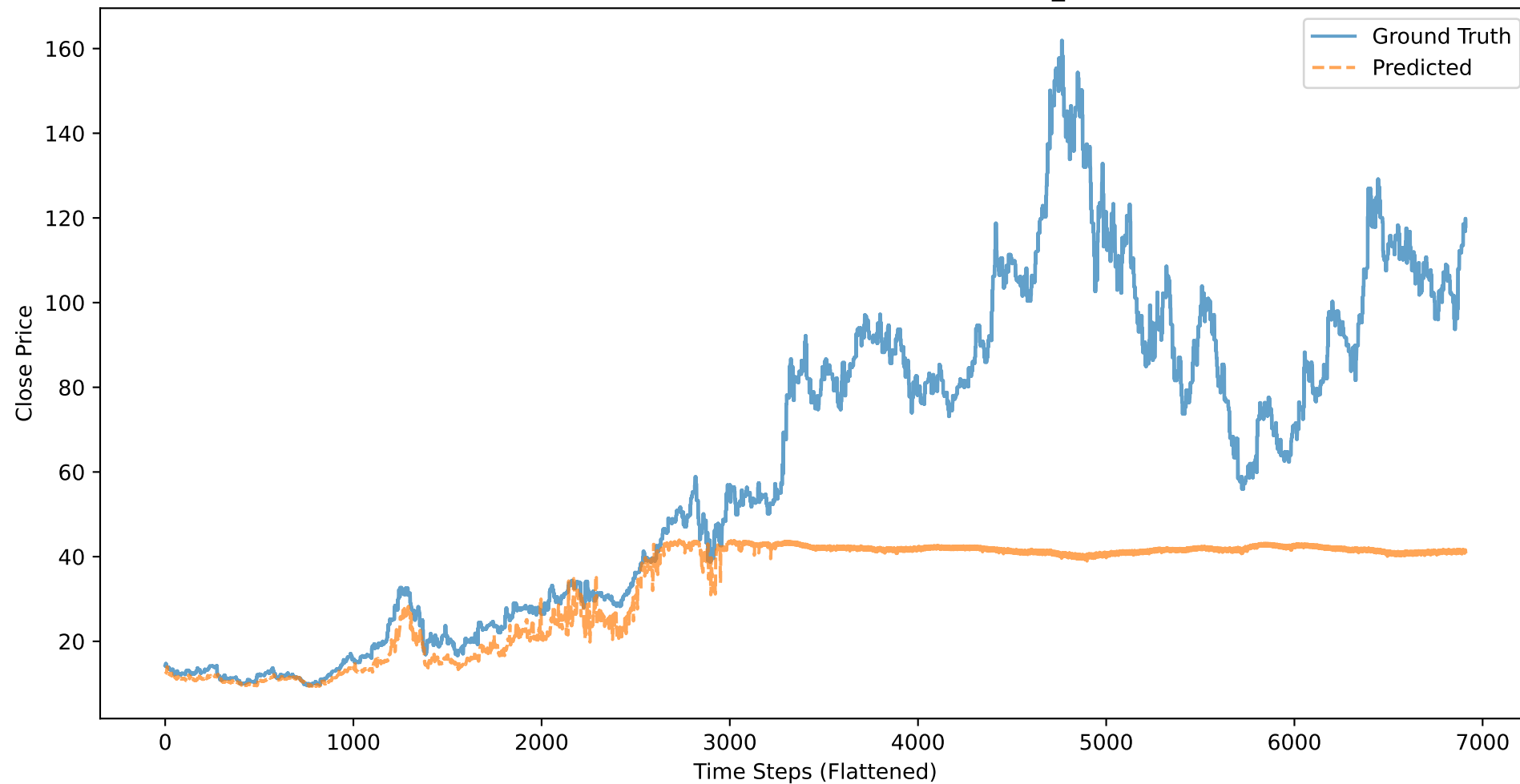
AMD: Close Price - Ground Truth vs Predicted (BASELINE_CLOSE, 50 stocks)
