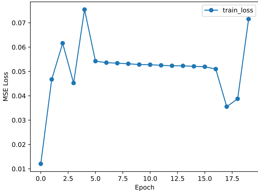
Training Loss (QQQ, BASELINE_CLOSE, 21 stocks - Close Only)
