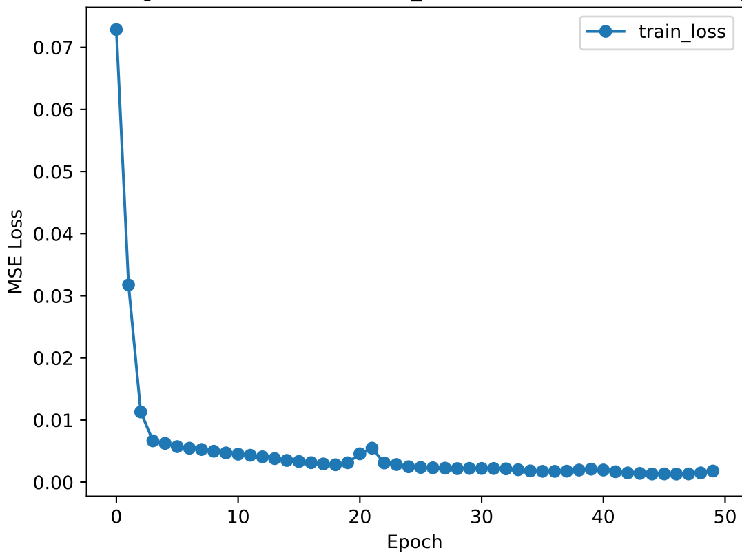
Training Loss (NVDA, BASELINE_CLOSE, 50 stocks - Close Only)
