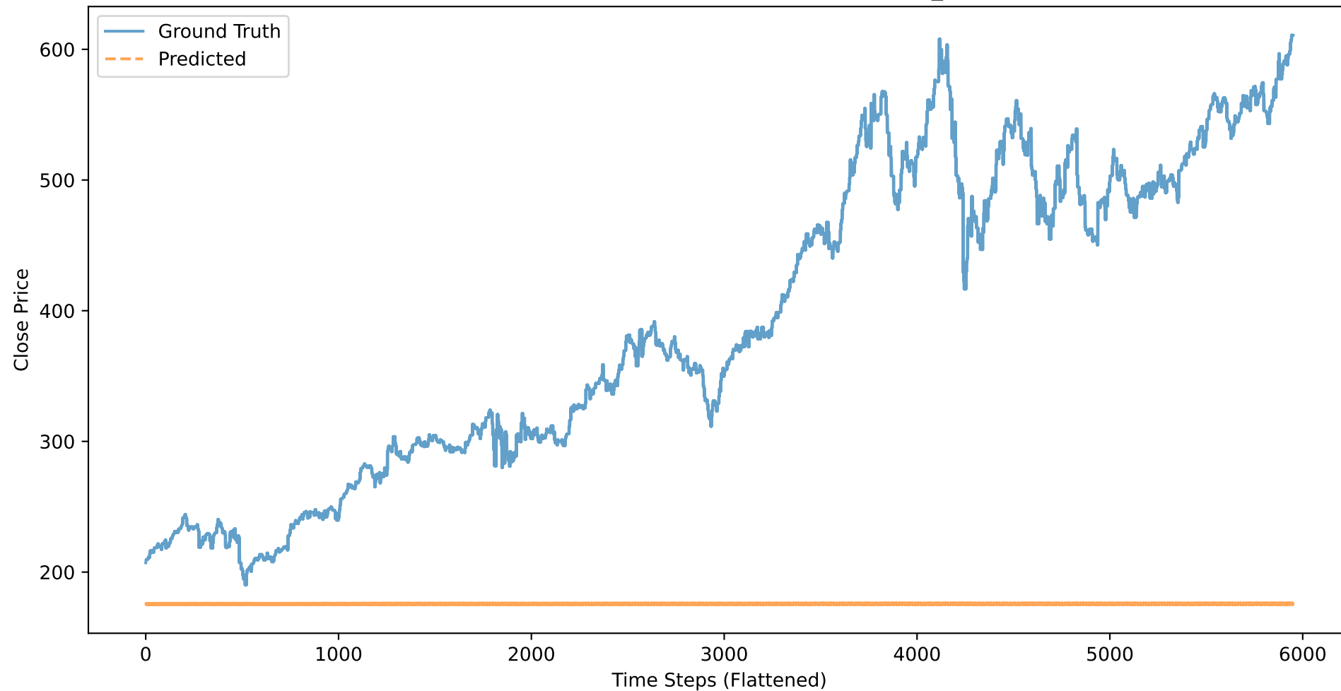
COST: Close Price - Ground Truth vs Predicted (BASELINE_CLOSE, 21 stocks)
