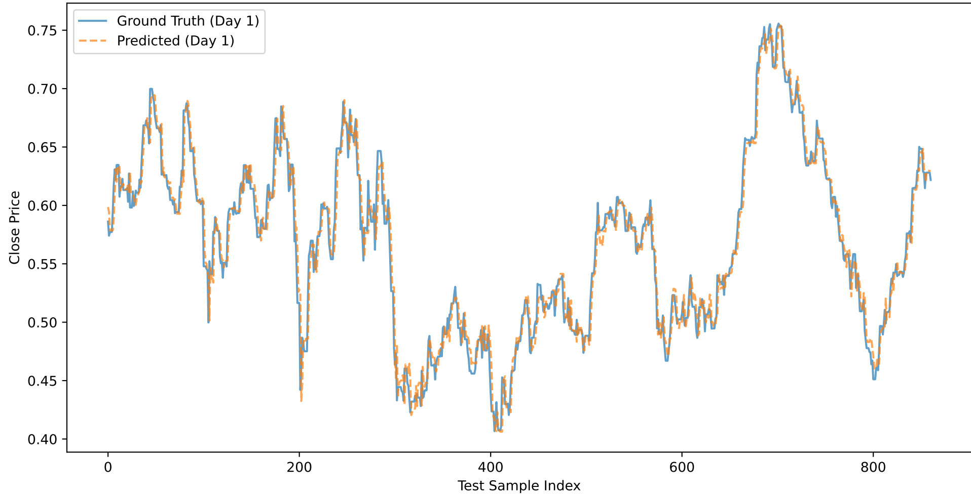
DAL: Close Price Prediction (Day 1) - NOVEL_XGB_CLOSE
