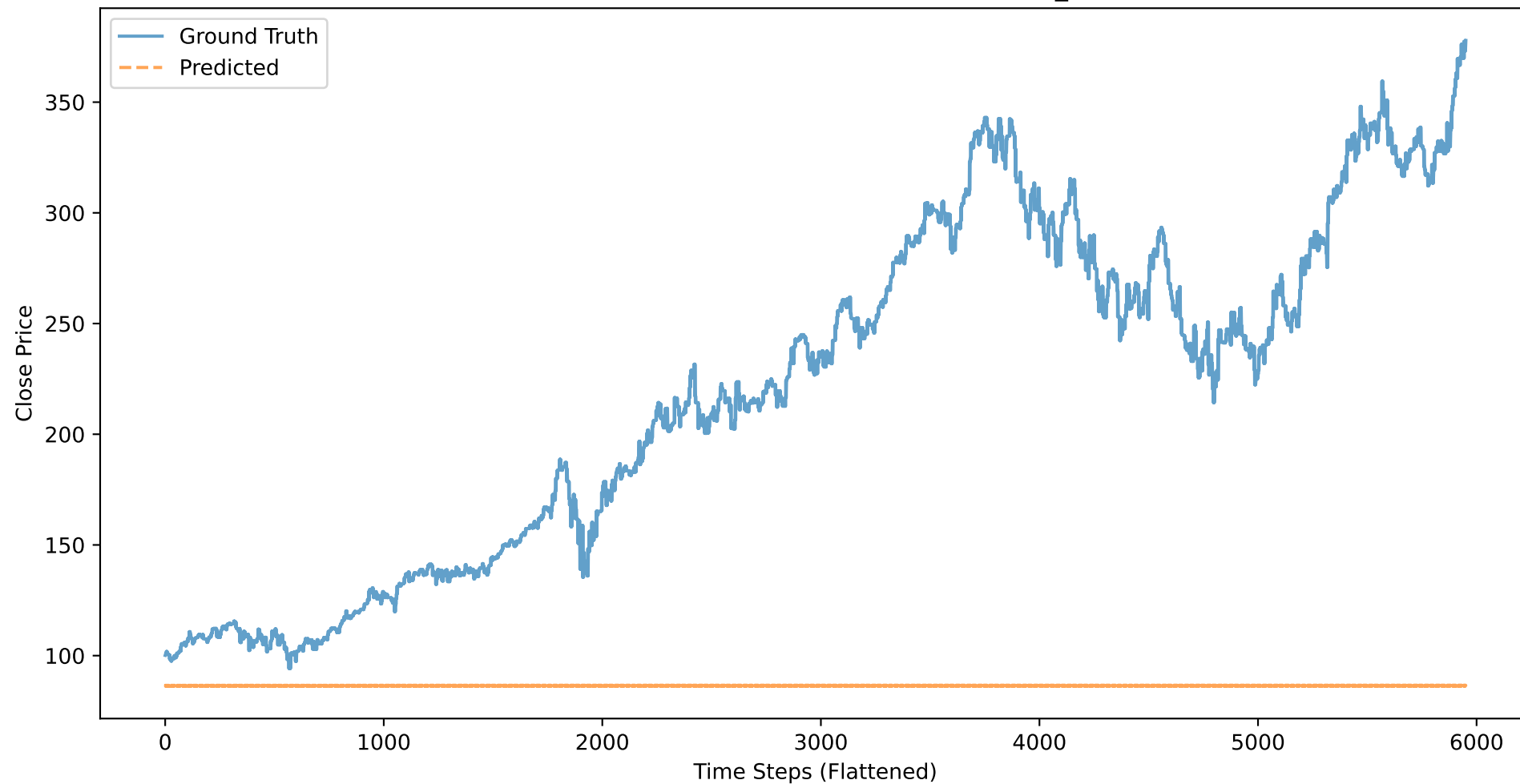
MSFT: Close Price - Ground Truth vs Predicted (BASELINE_CLOSE, 21 stocks)
