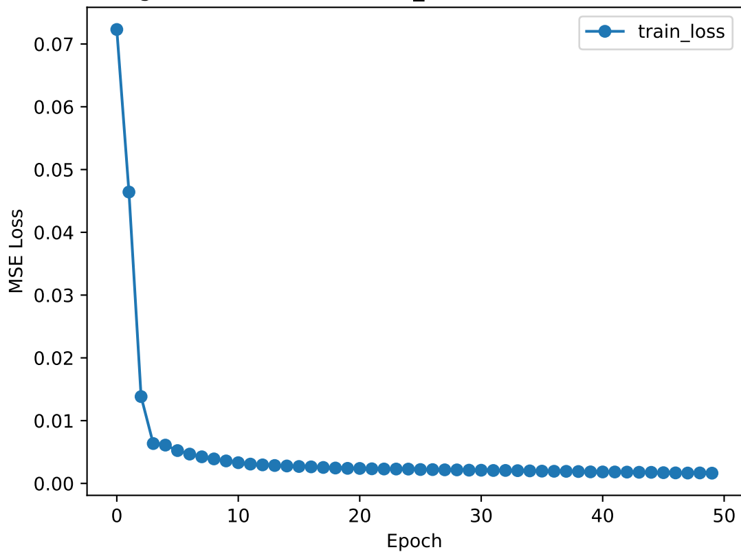
Training Loss (GOOG, BASELINE_CLOSE, 50 stocks - Close Only)
