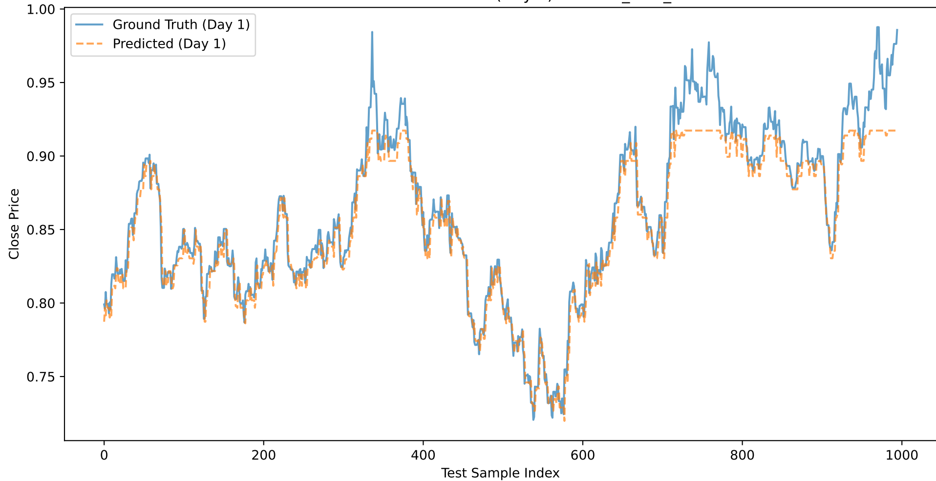
GLD: Close Price Prediction (Day 1) - NOVEL_XGB_CLOSE
