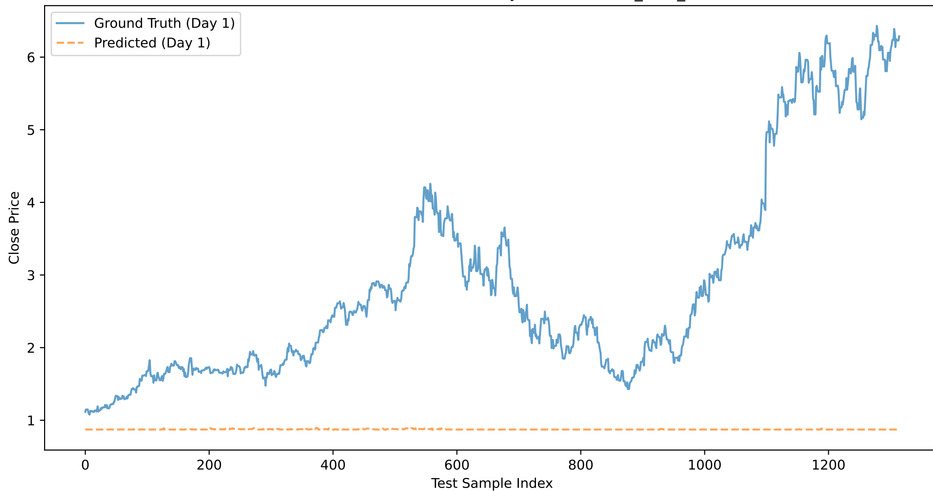
NVDA: Close Price Prediction (Day 1) - BASELINE_XGB_CLOSE
