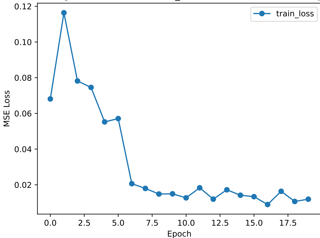
Training Loss (PYPL, BASELINE_CLOSE, 21 stocks - Close Only)
