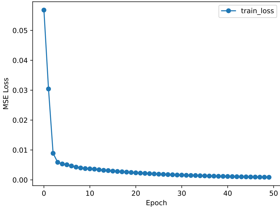
Training Loss (NKE, BASELINE_CLOSE, 50 stocks - Close Only)
