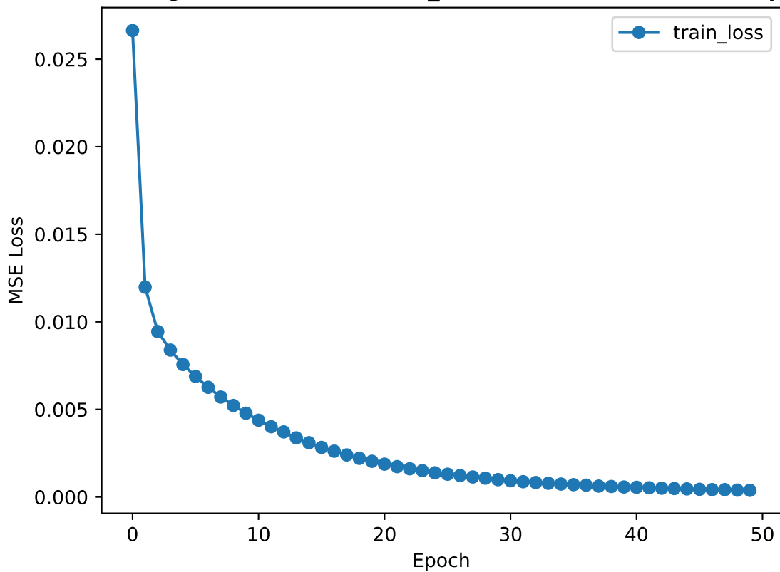
Training Loss (CVX, BASELINE_CLOSE, 50 stocks - Close Only)
