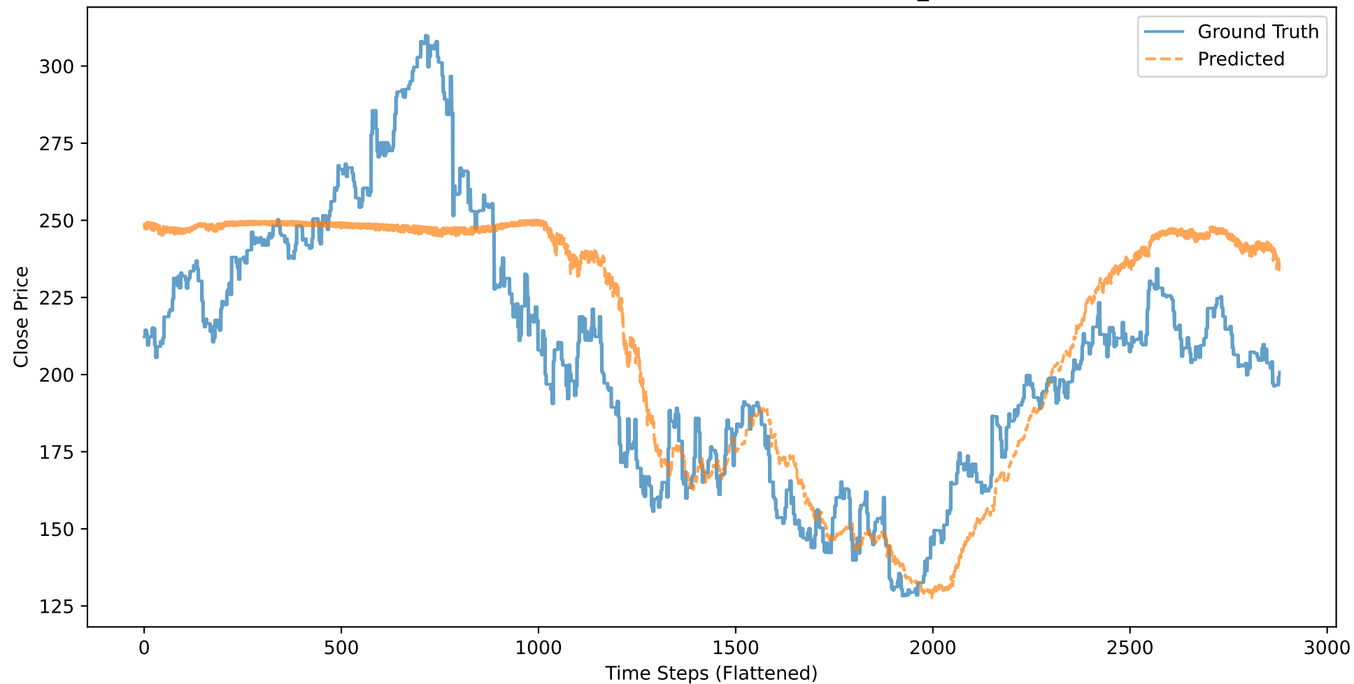
CRM: Close Price - Ground Truth vs Predicted (BASELINE_CLOSE, 50 stocks)
