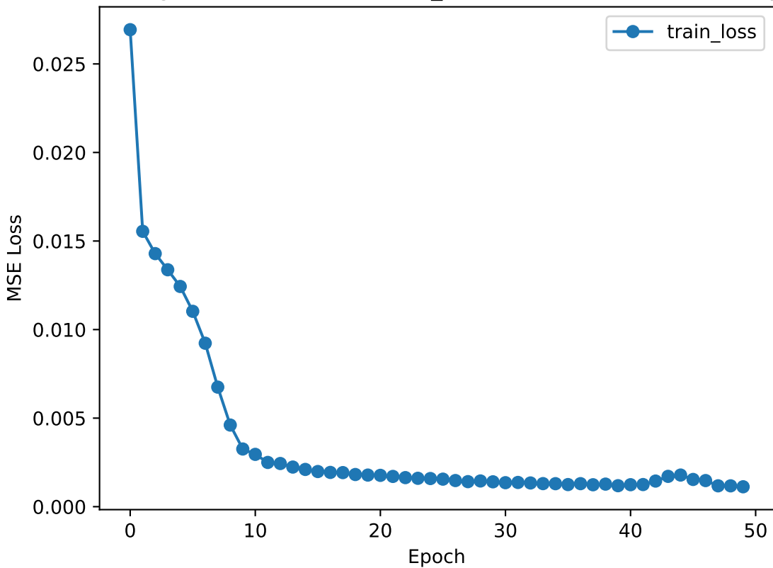
Training Loss (SBUX, BASELINE_CLOSE, 50 stocks - Close Only)
