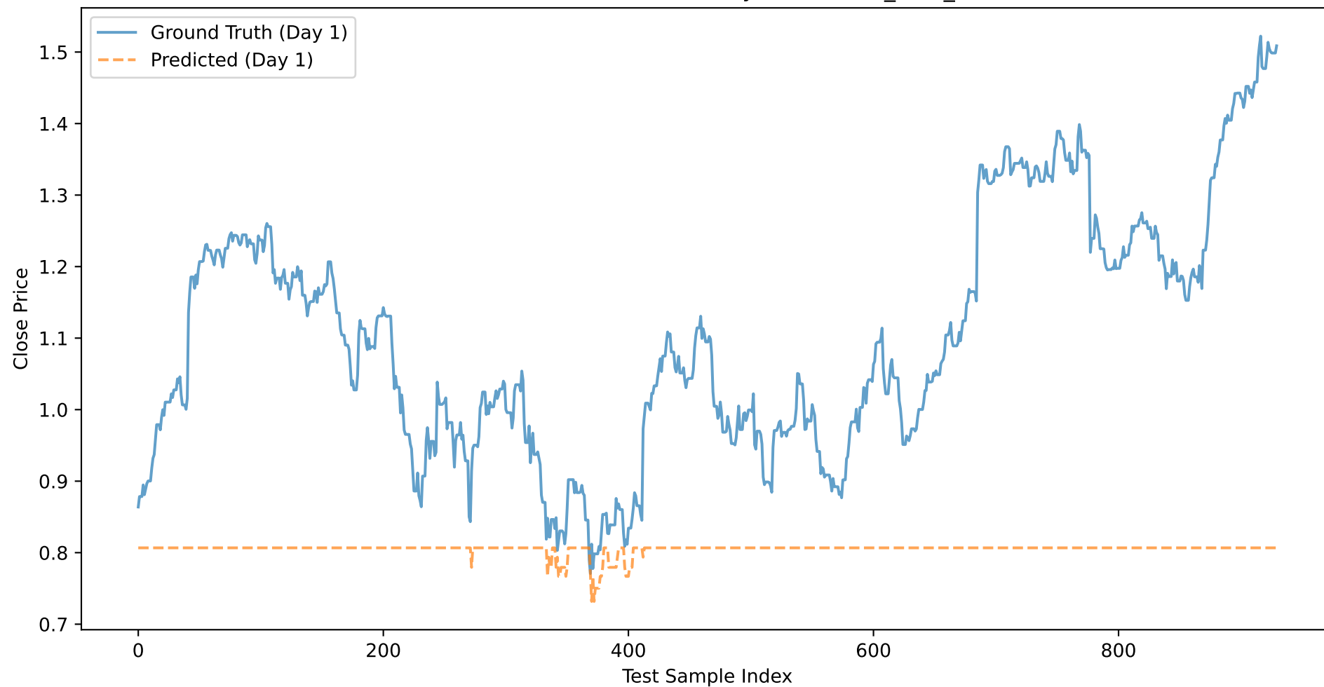
CMG: Close Price Prediction (Day 1) - NOVEL_XGB_CLOSE
