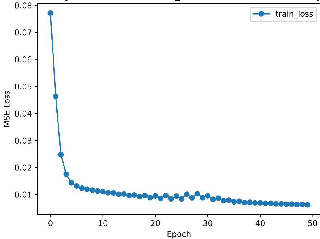
Training Loss (PYPL, BASELINE_CLOSE, 50 stocks - Close Only)
