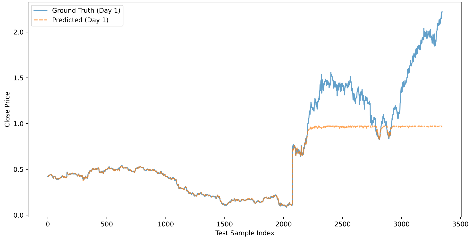
GE: Close Price Prediction (Day 1) - BASELINE_XGB_CLOSE
