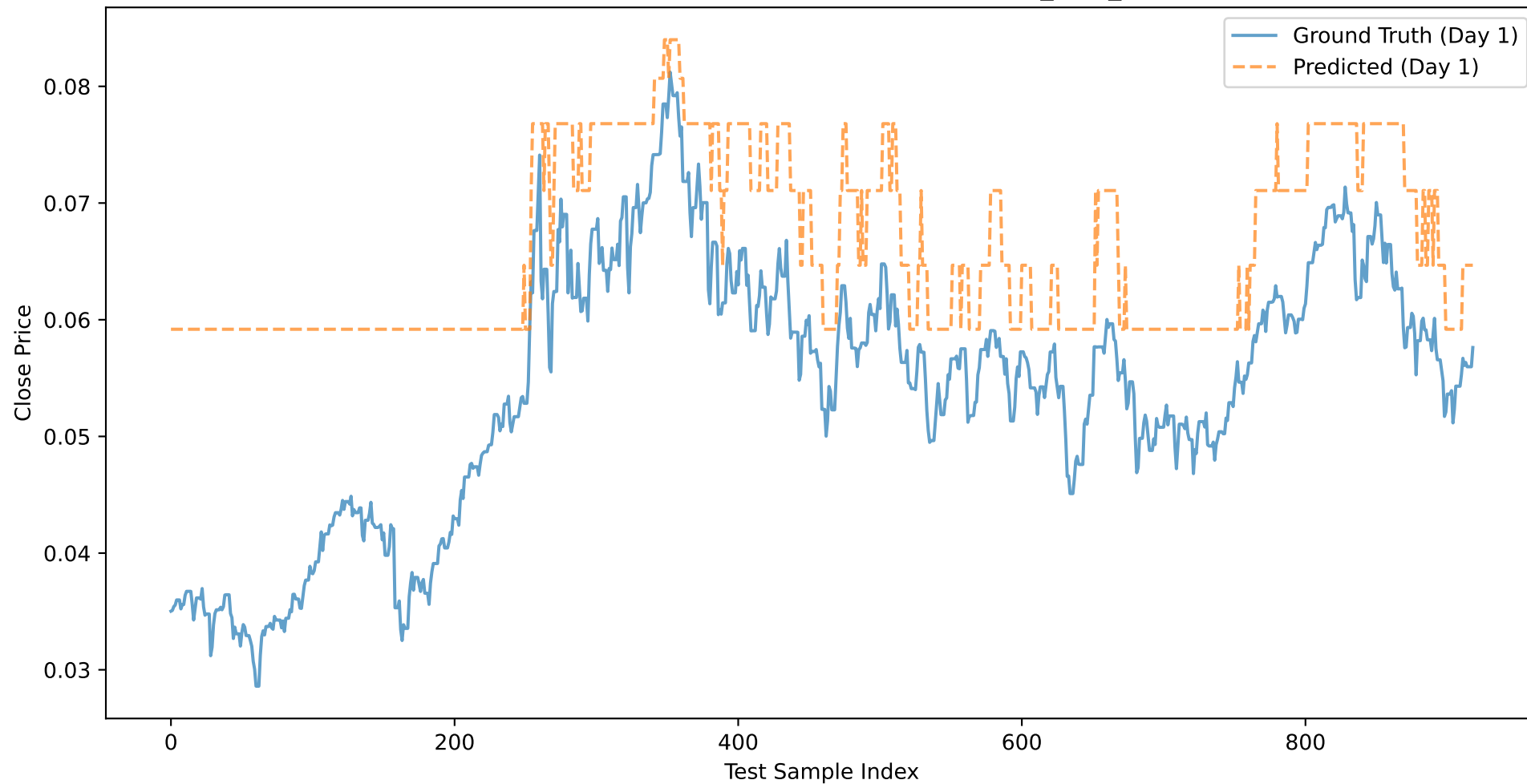
USO: Close Price Prediction (Day 1) - BASELINE_XGB_CLOSE
