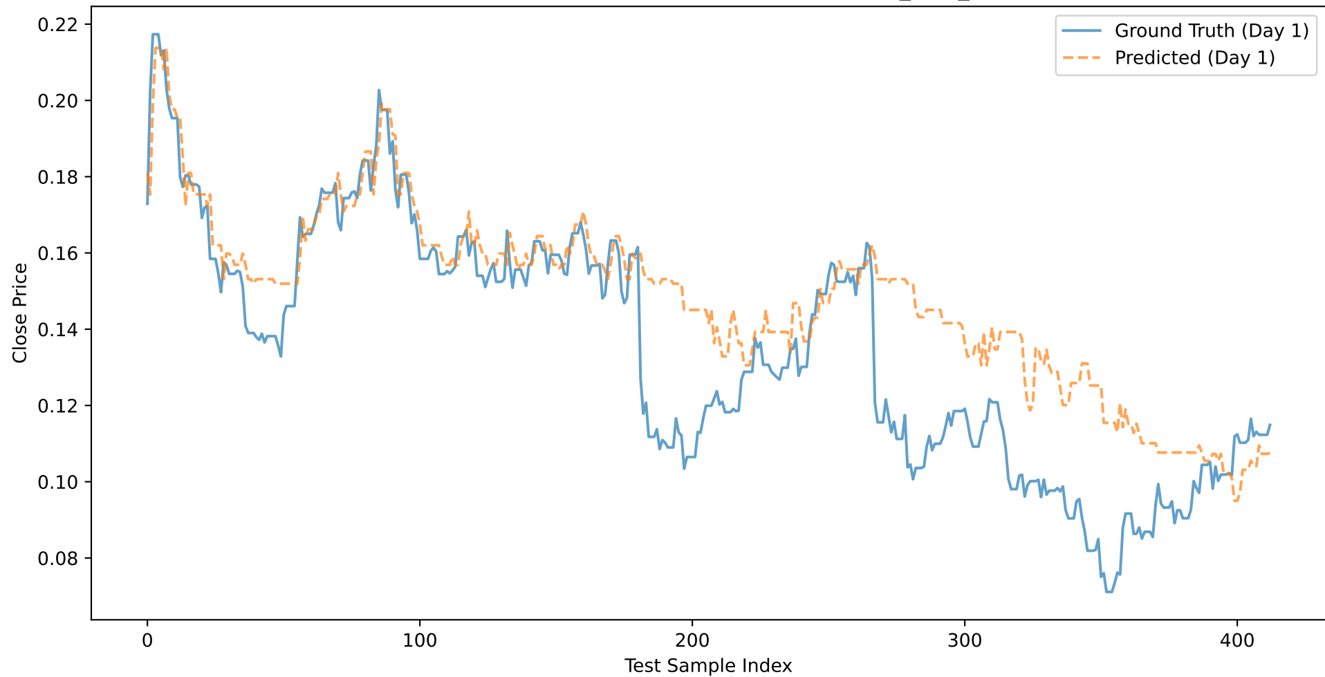
PYPL: Close Price Prediction (Day 1) - BASELINE_XGB_CLOSE
