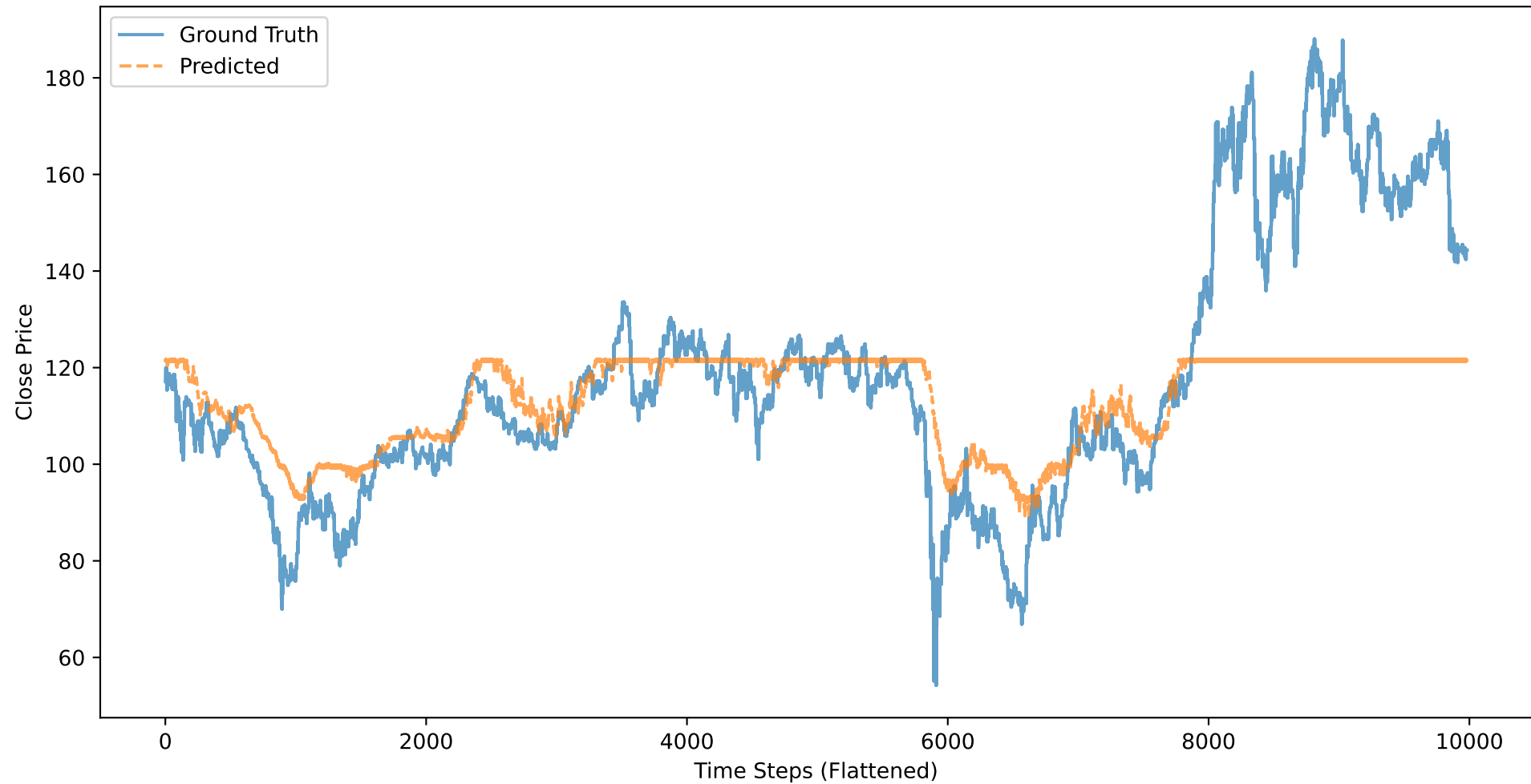
CVX: Close Price - Ground Truth vs Predicted (BASELINE_CLOSE, 21 stocks)
