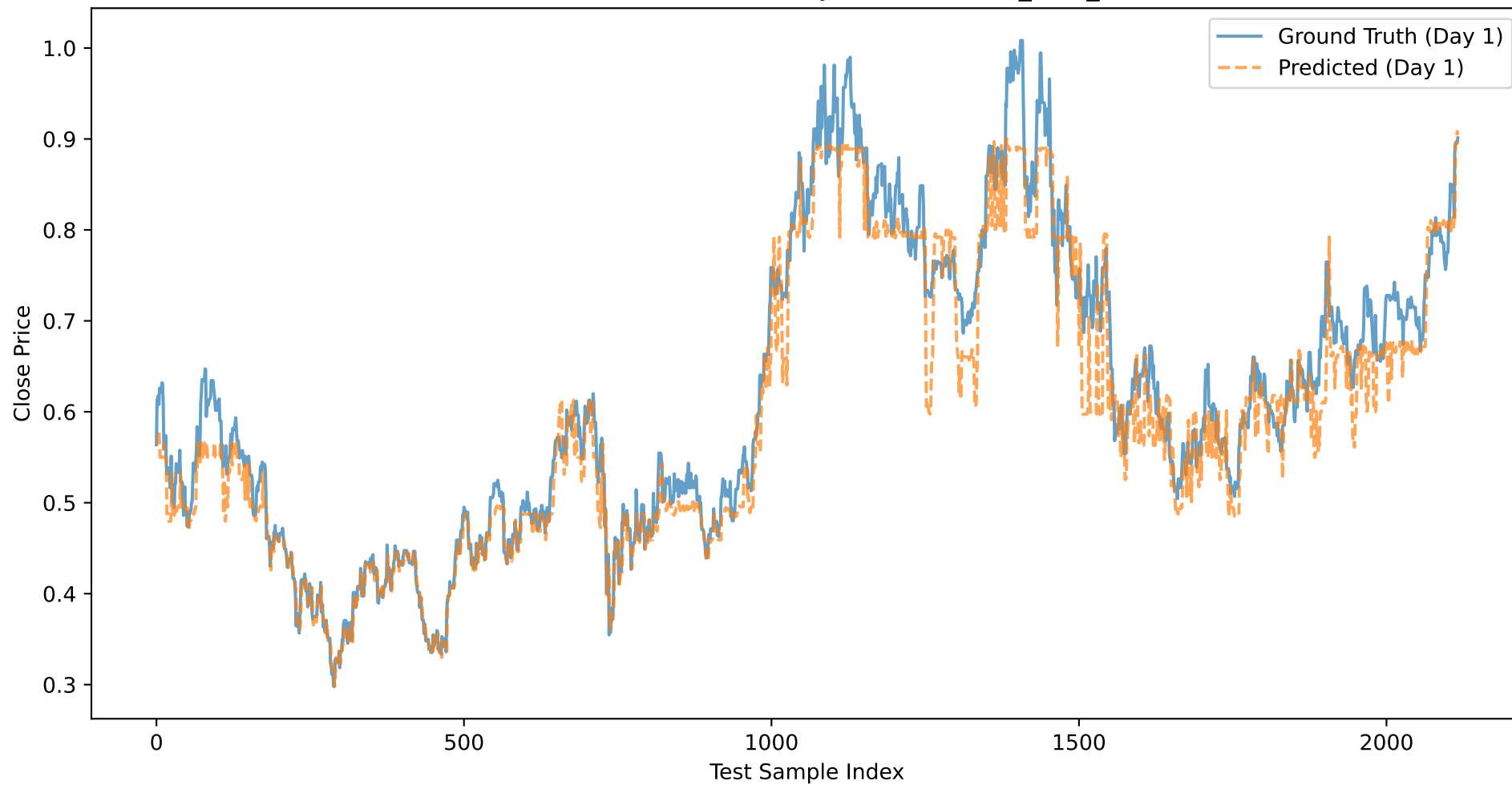
MU: Close Price Prediction (Day 1) - BASELINE_XGB_CLOSE
