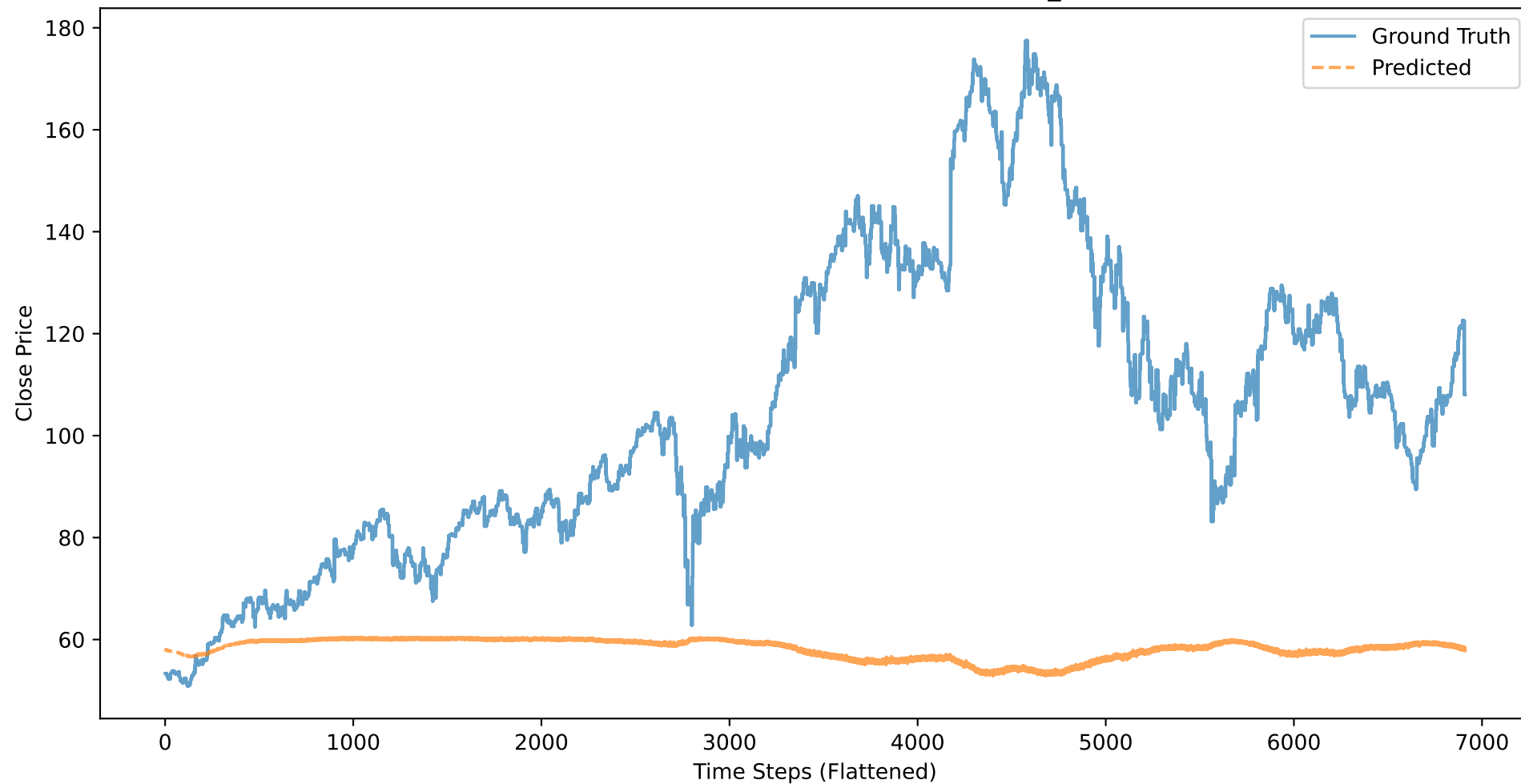
NKE: Close Price - Ground Truth vs Predicted (BASELINE_CLOSE, 50 stocks)
