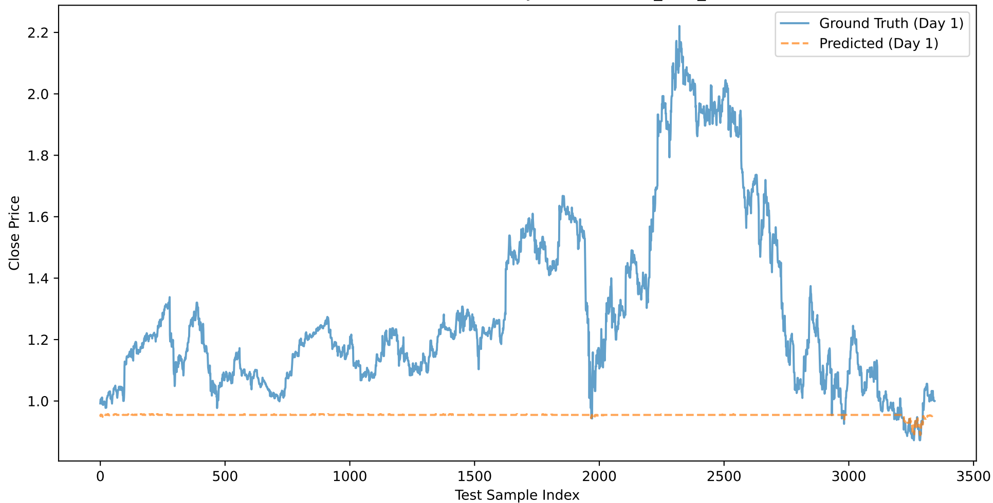
DIS: Close Price Prediction (Day 1) - BASELINE_XGB_CLOSE
