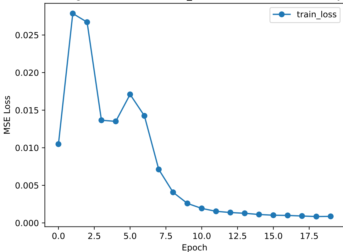
Training Loss (DIS, BASELINE_CLOSE, 21 stocks - Close Only)
