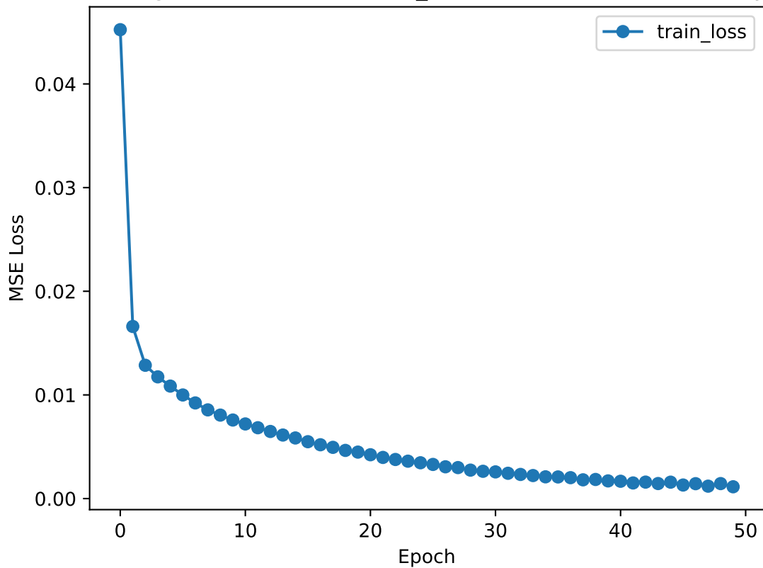
Training Loss (INTC, BASELINE_CLOSE, 50 stocks - Close Only)
