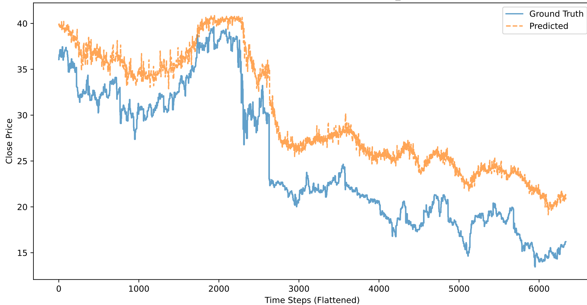
T: Close Price - Ground Truth vs Predicted (BASELINE_CLOSE, 50 stocks)
