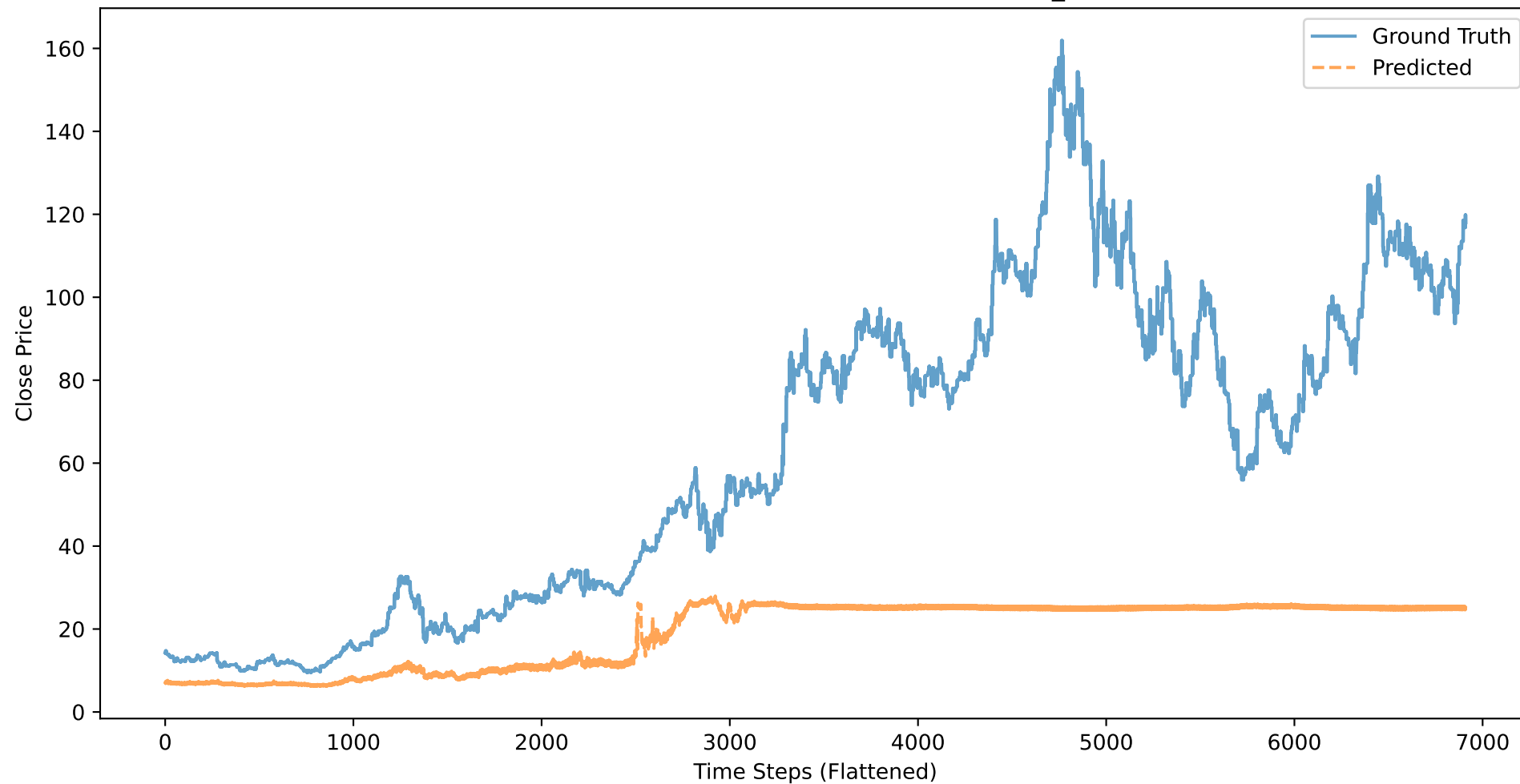
AMD: Close Price - Ground Truth vs Predicted (BASELINE_CLOSE, 21 stocks)
