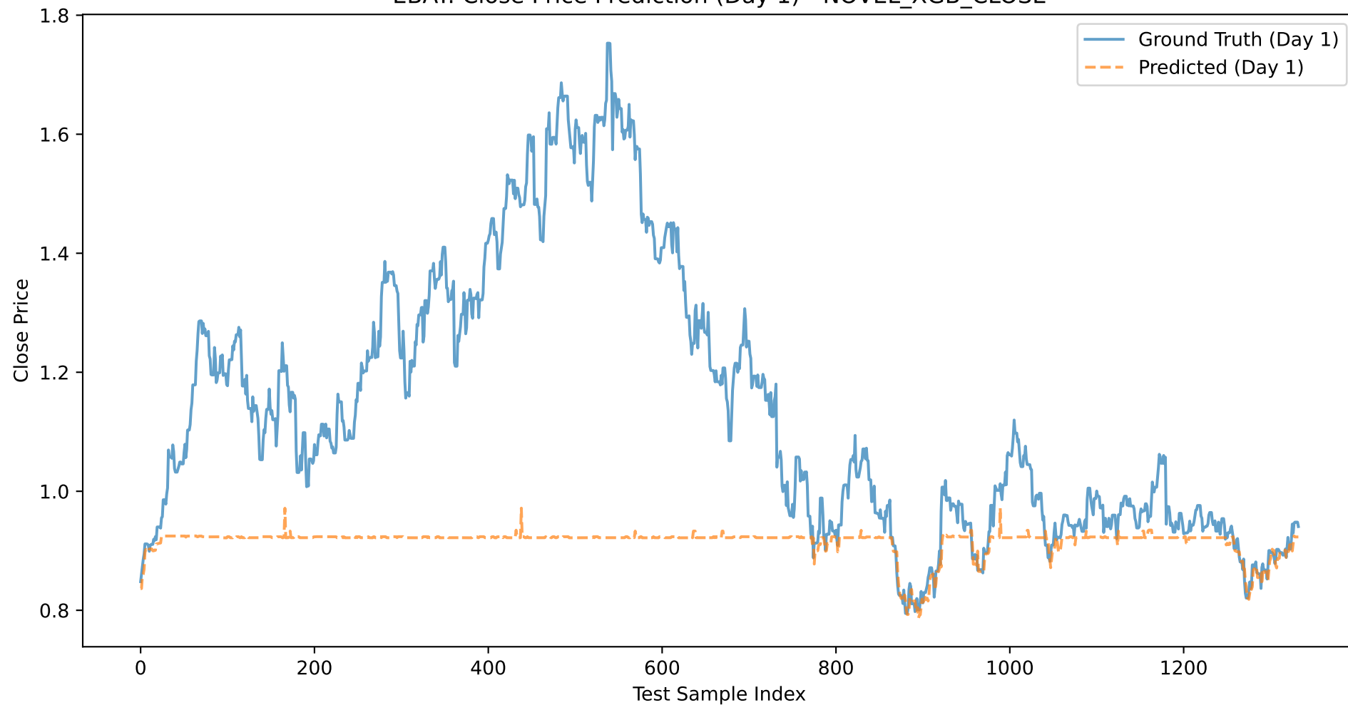
EBAY: Close Price Prediction (Day 1) - NOVEL_XGB_CLOSE
