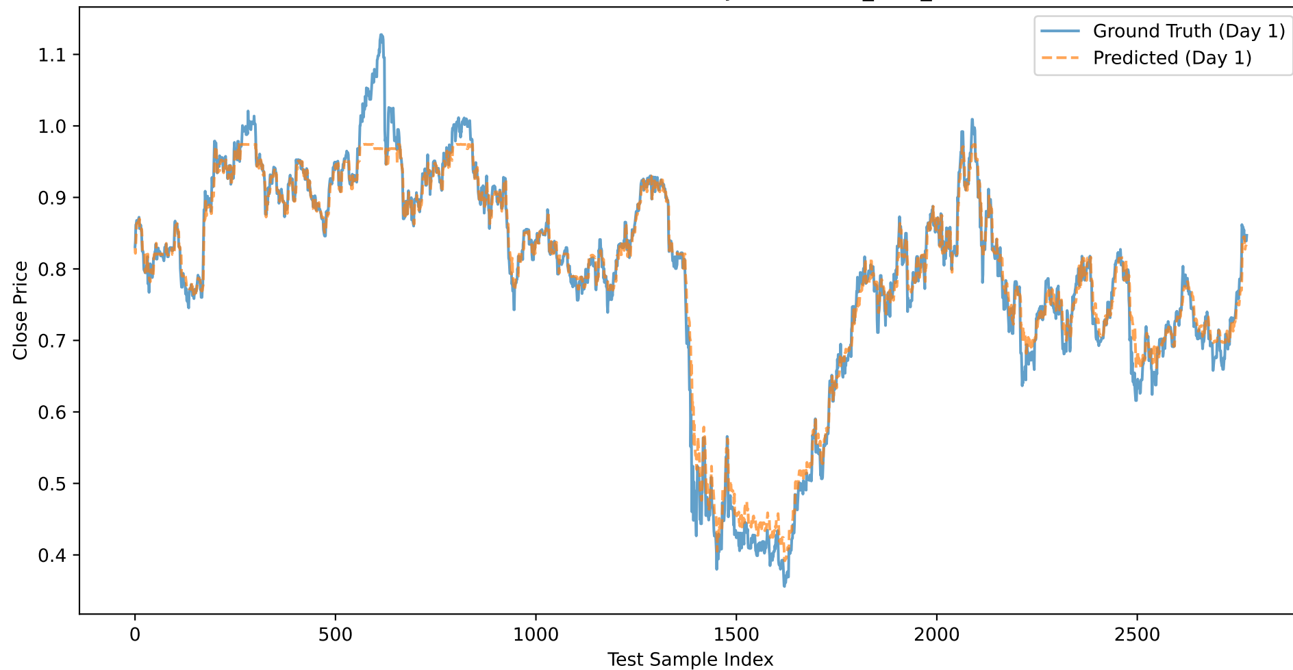
WFC: Close Price Prediction (Day 1) - NOVEL_XGB_CLOSE
