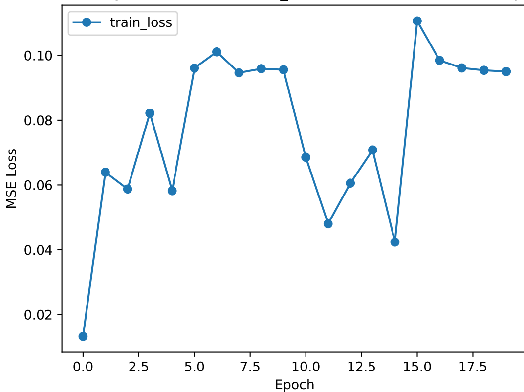
Training Loss (KO, BASELINE_CLOSE, 21 stocks - Close Only)
