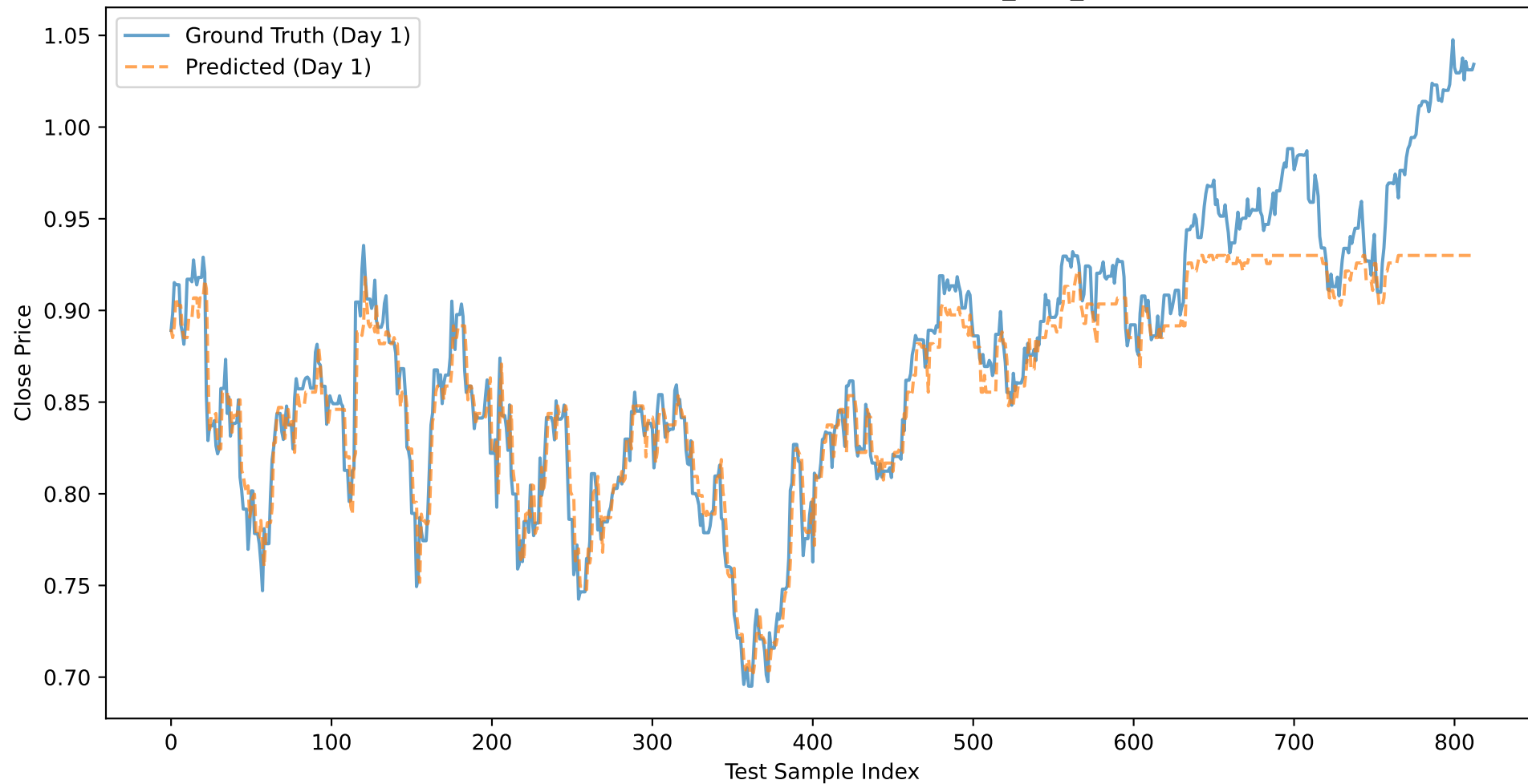
V: Close Price Prediction (Day 1) - NOVEL_XGB_CLOSE
