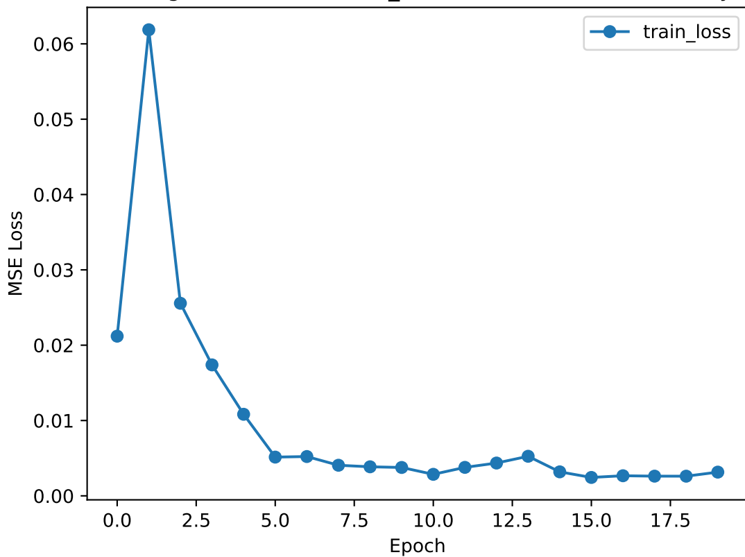
Training Loss (T, BASELINE_CLOSE, 21 stocks - Close Only)
