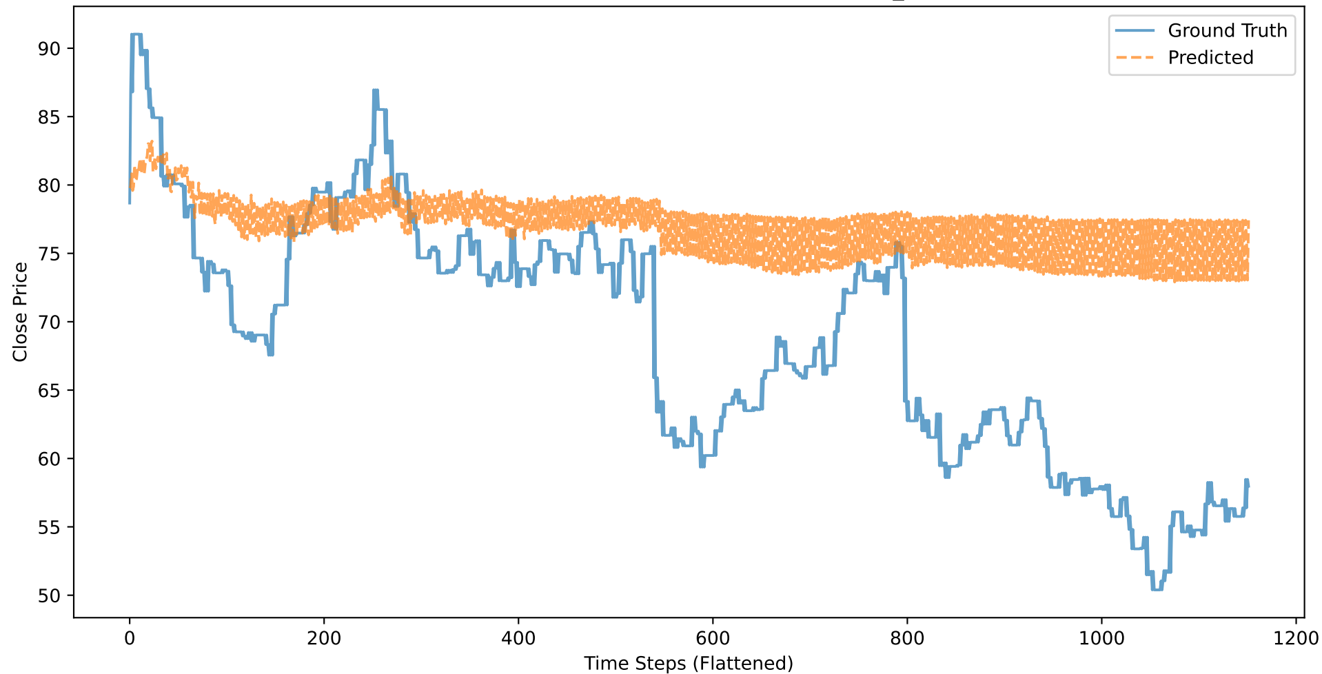
PYPL: Close Price - Ground Truth vs Predicted (BASELINE_CLOSE, 50 stocks)
