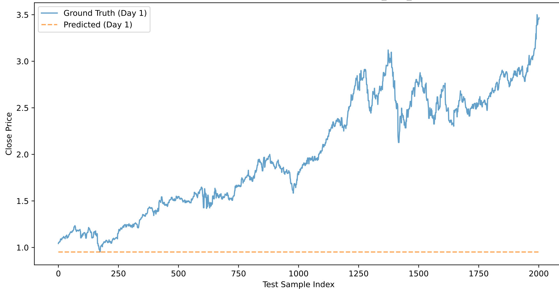
COST: Close Price Prediction (Day 1) - BASELINE_XGB_CLOSE
