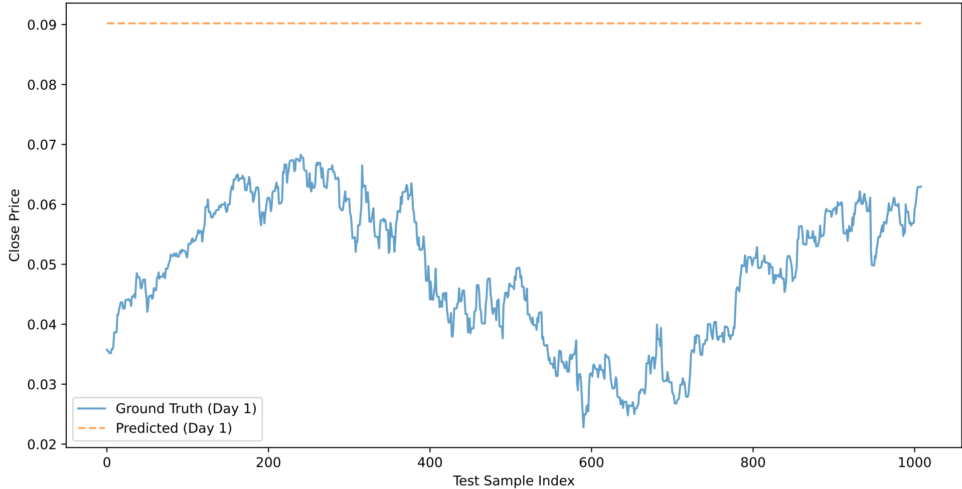
GOOG: Close Price Prediction (Day 1) - NOVEL_XGB_CLOSE
