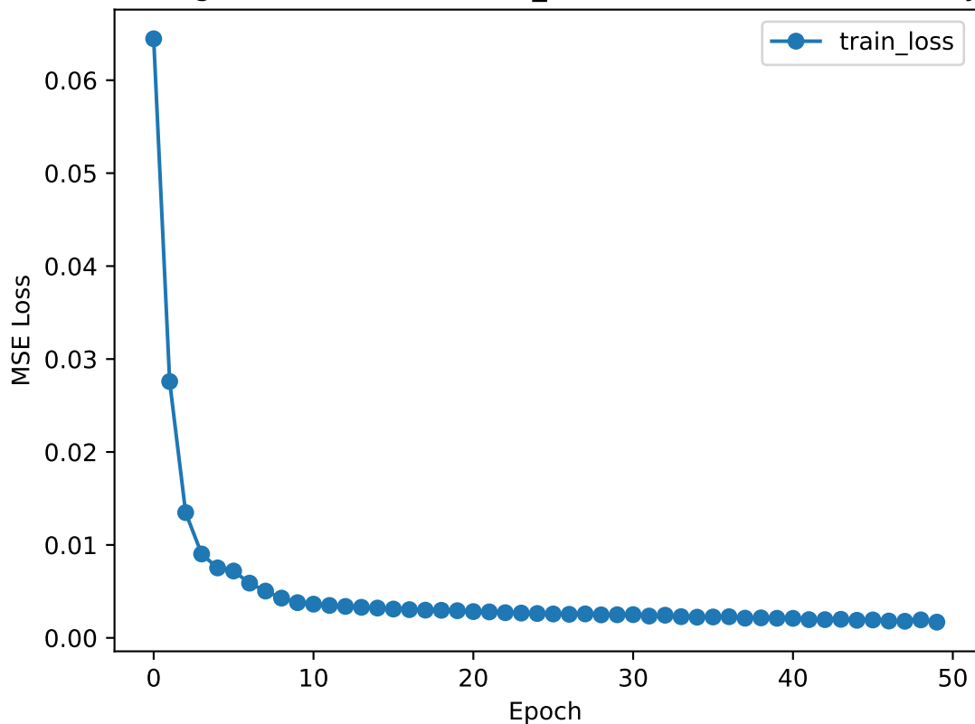
Training Loss (CMG, BASELINE_CLOSE, 50 stocks - Close Only)
