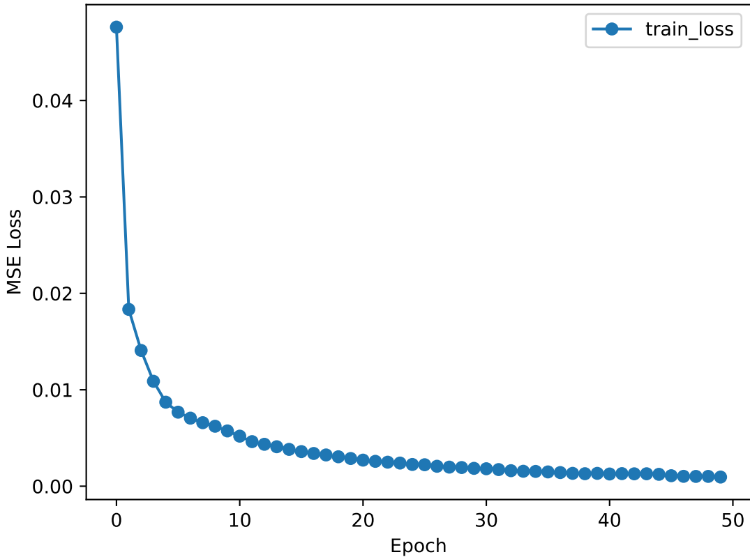
Training Loss (BHP, BASELINE_CLOSE, 50 stocks - Close Only)
