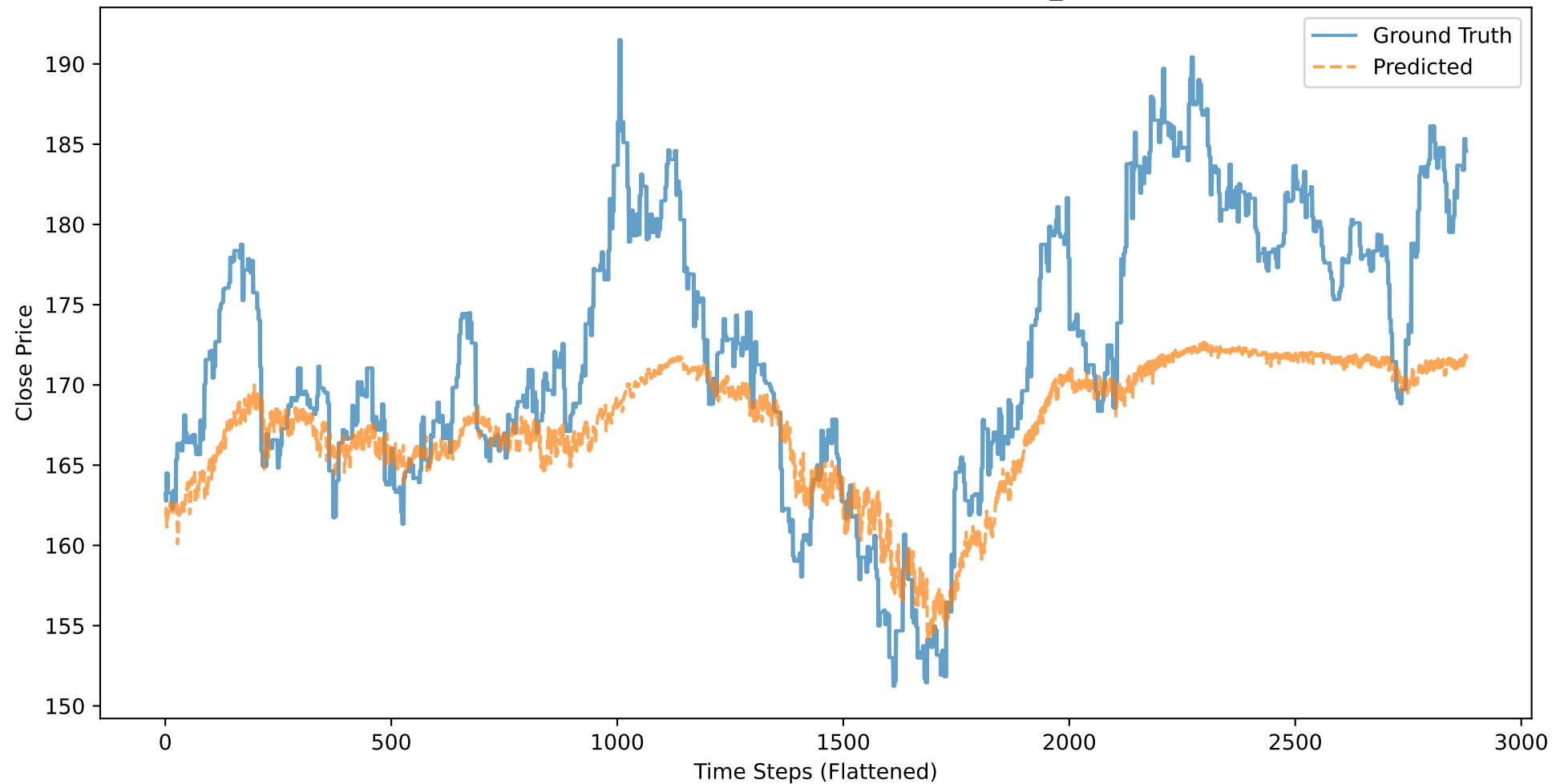
GLD: Close Price - Ground Truth vs Predicted (BASELINE_CLOSE, 50 stocks)
