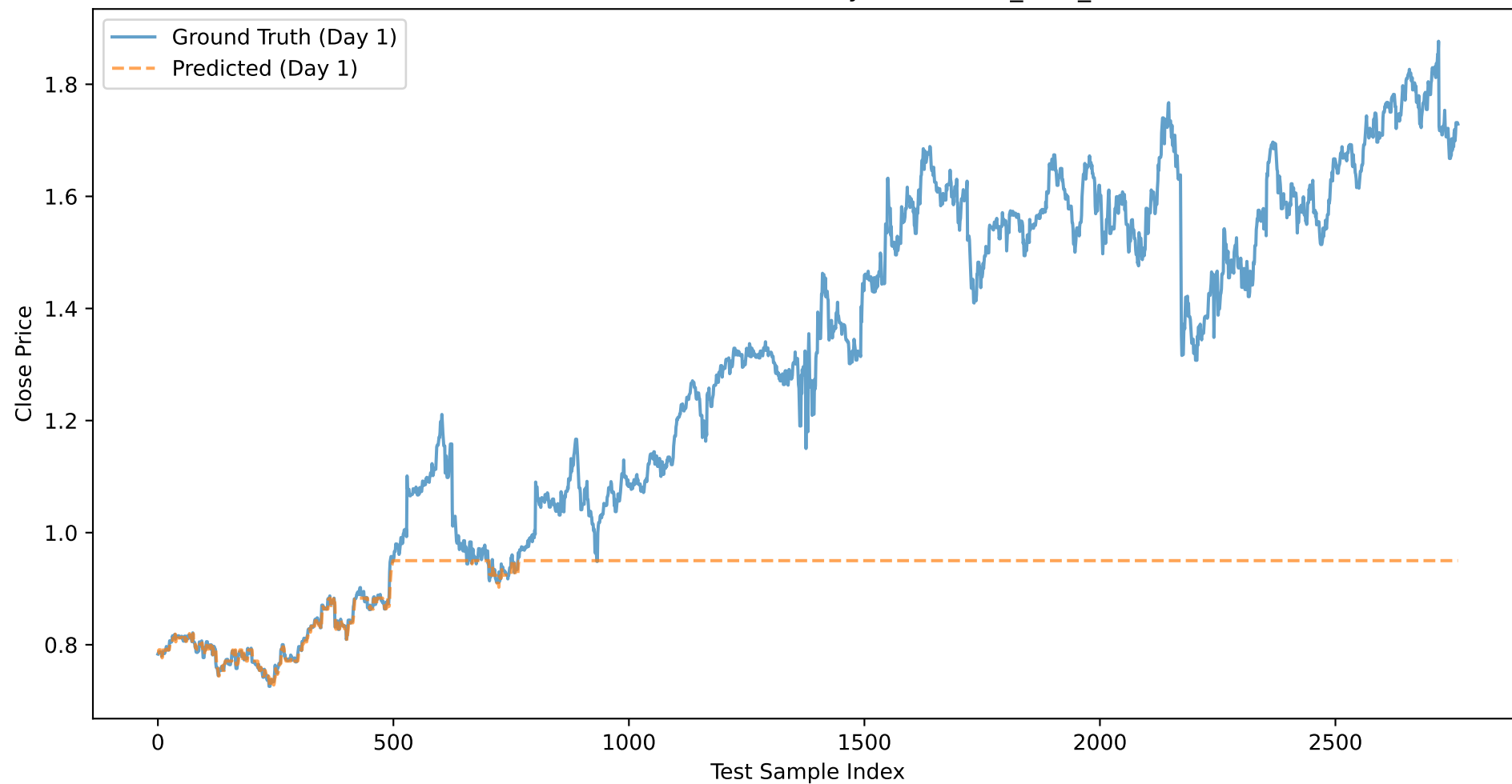
WMT: Close Price Prediction (Day 1) - NOVEL_XGB_CLOSE
