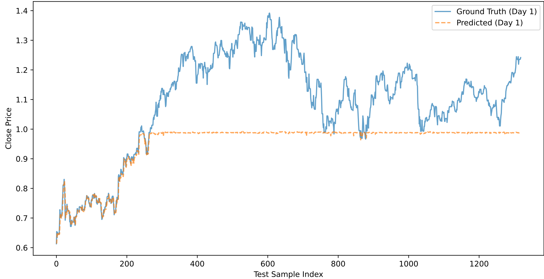
XLF: Close Price Prediction (Day 1) - BASELINE_XGB_CLOSE
