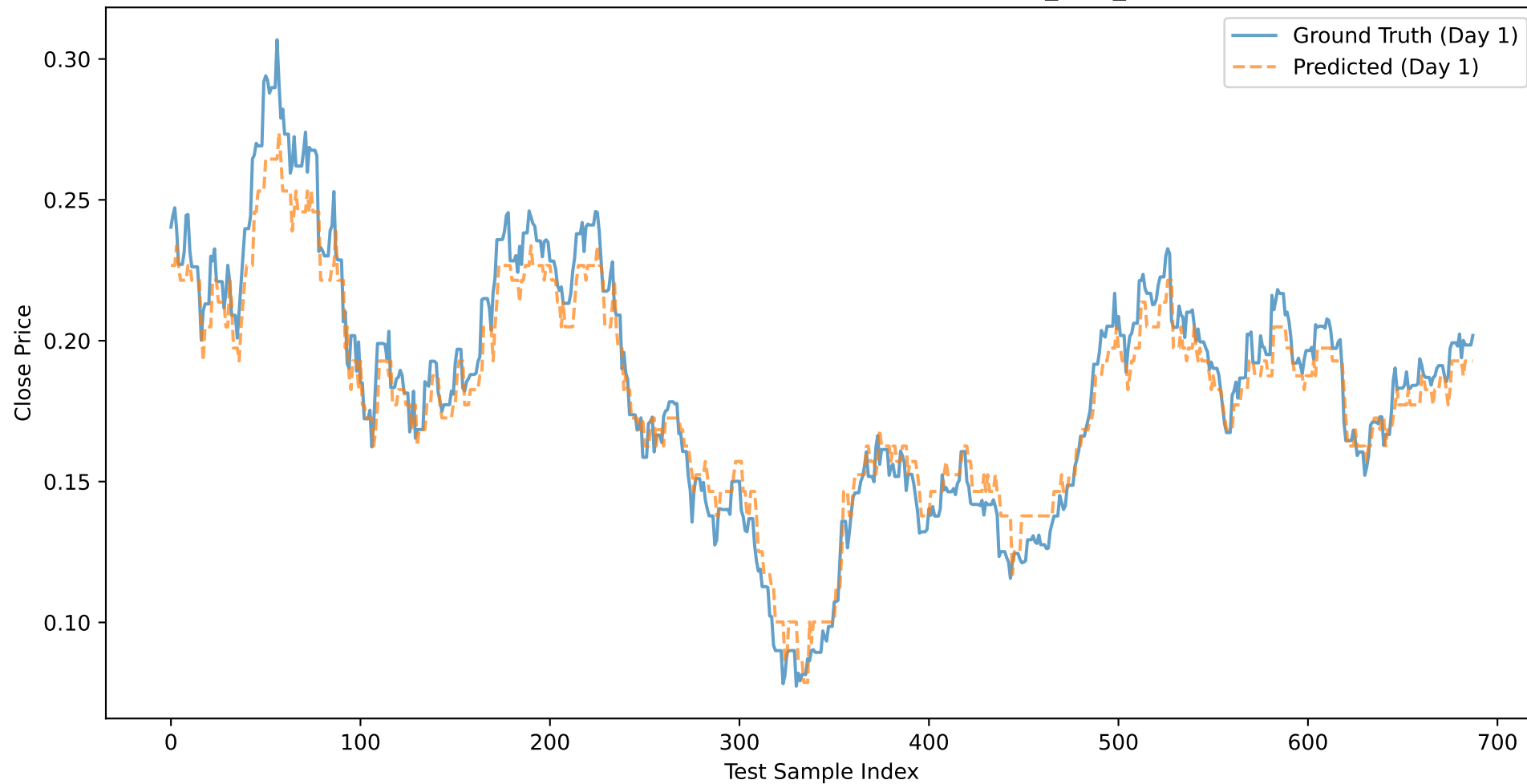
TSLA: Close Price Prediction (Day 1) - BASELINE_XGB_CLOSE
