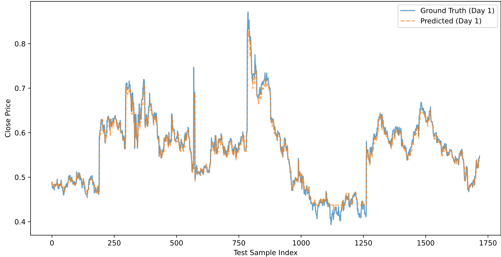
BIIB: Close Price Prediction (Day 1) - NOVEL_XGB_CLOSE
