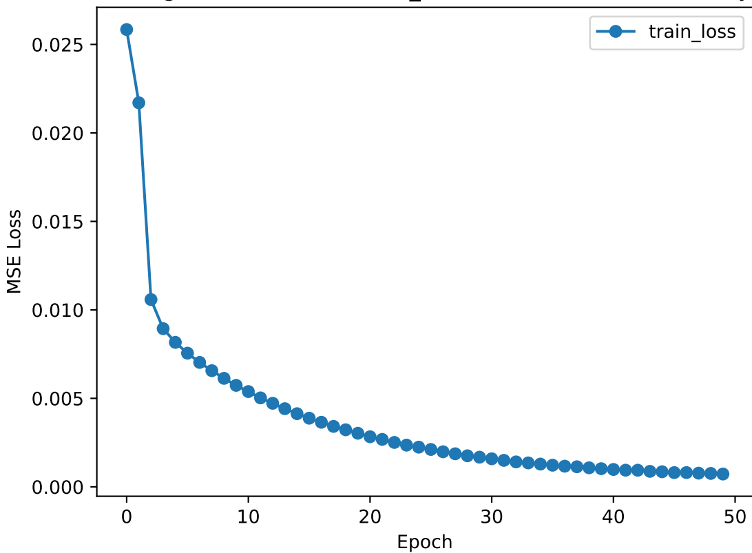
Training Loss (PEP, BASELINE_CLOSE, 50 stocks - Close Only)
