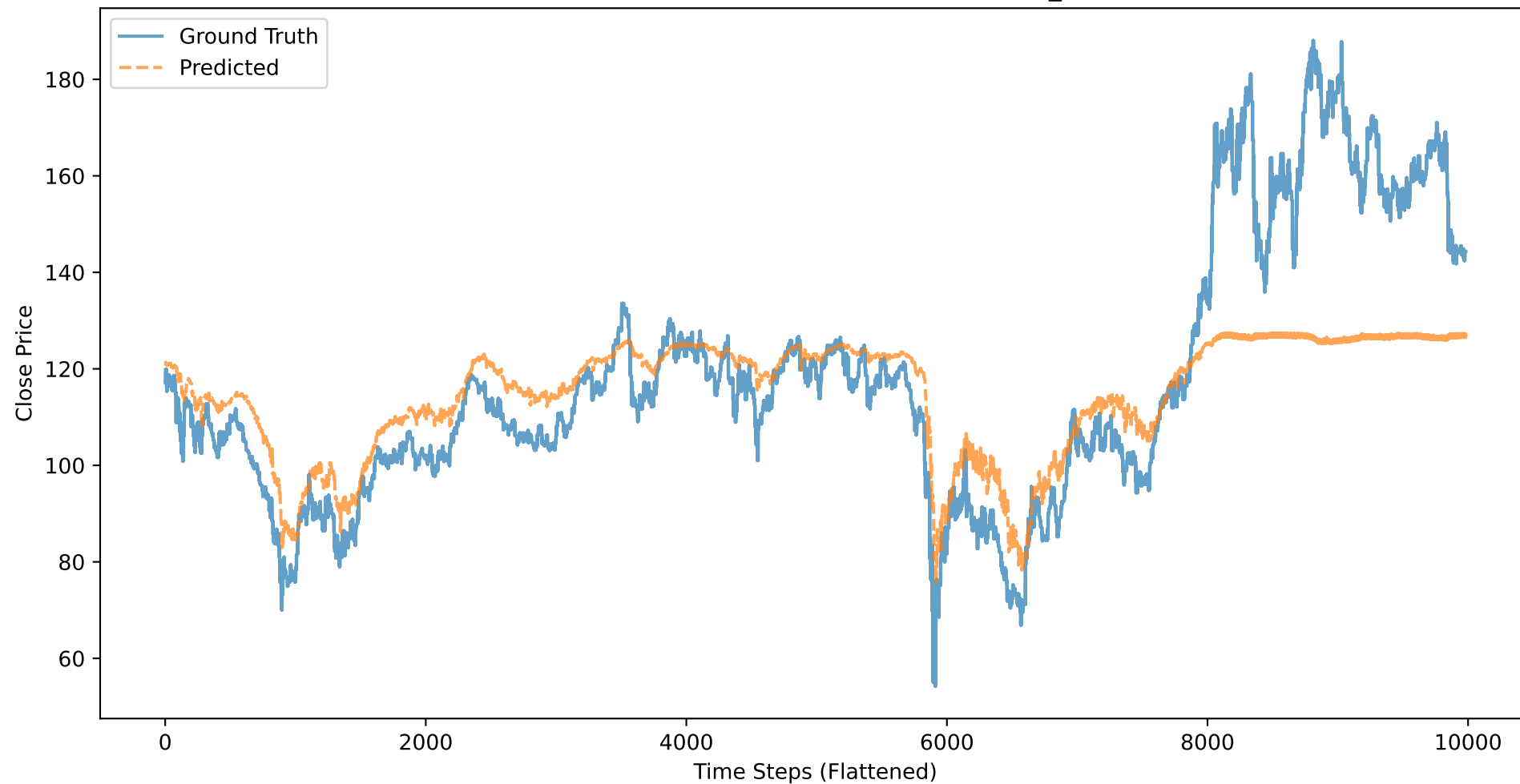
CVX: Close Price - Ground Truth vs Predicted (BASELINE_CLOSE, 50 stocks)
