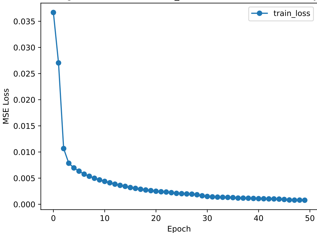
Training Loss (WFC, BASELINE_CLOSE, 50 stocks - Close Only)
