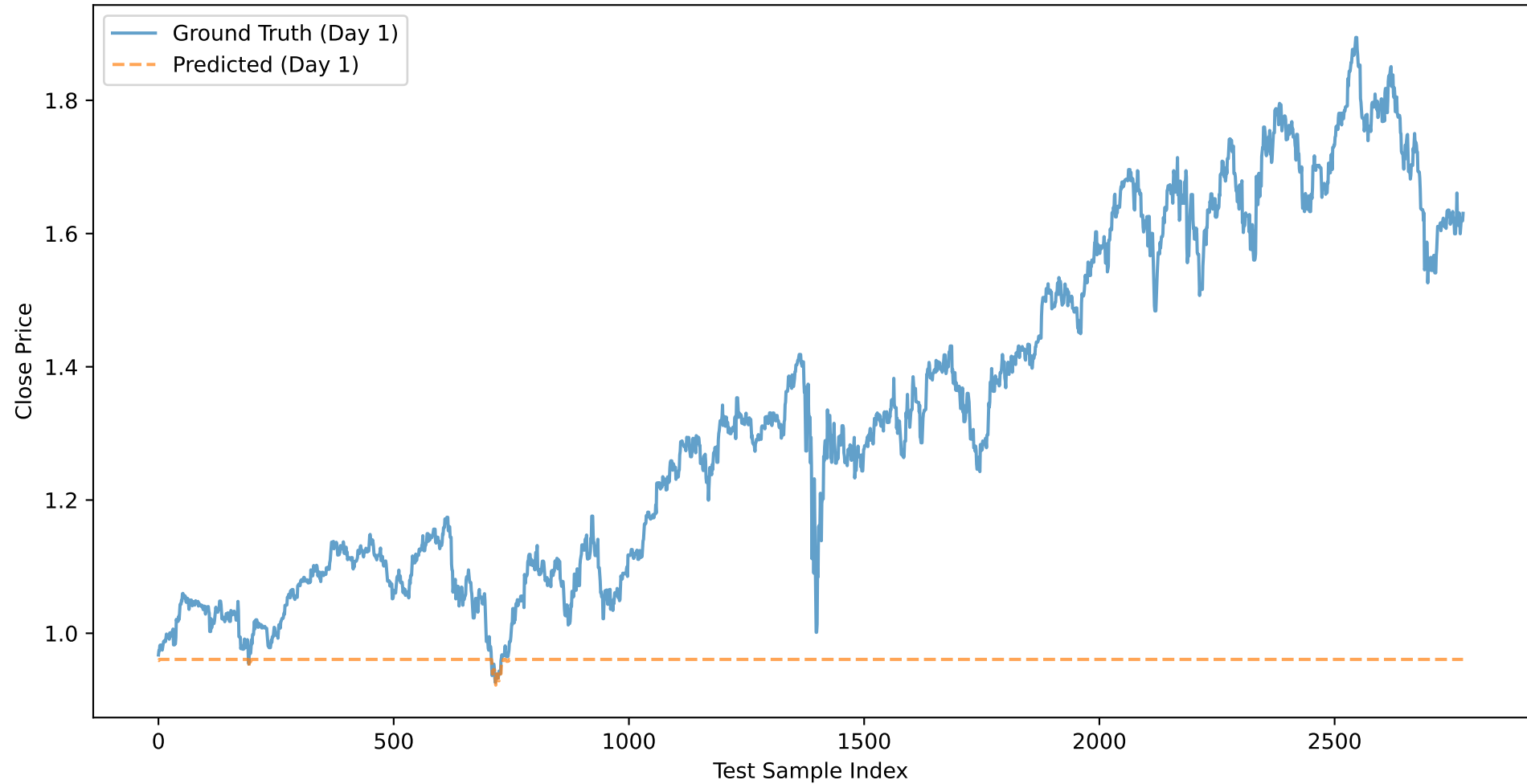
PEP: Close Price Prediction (Day 1) - NOVEL_XGB_CLOSE
