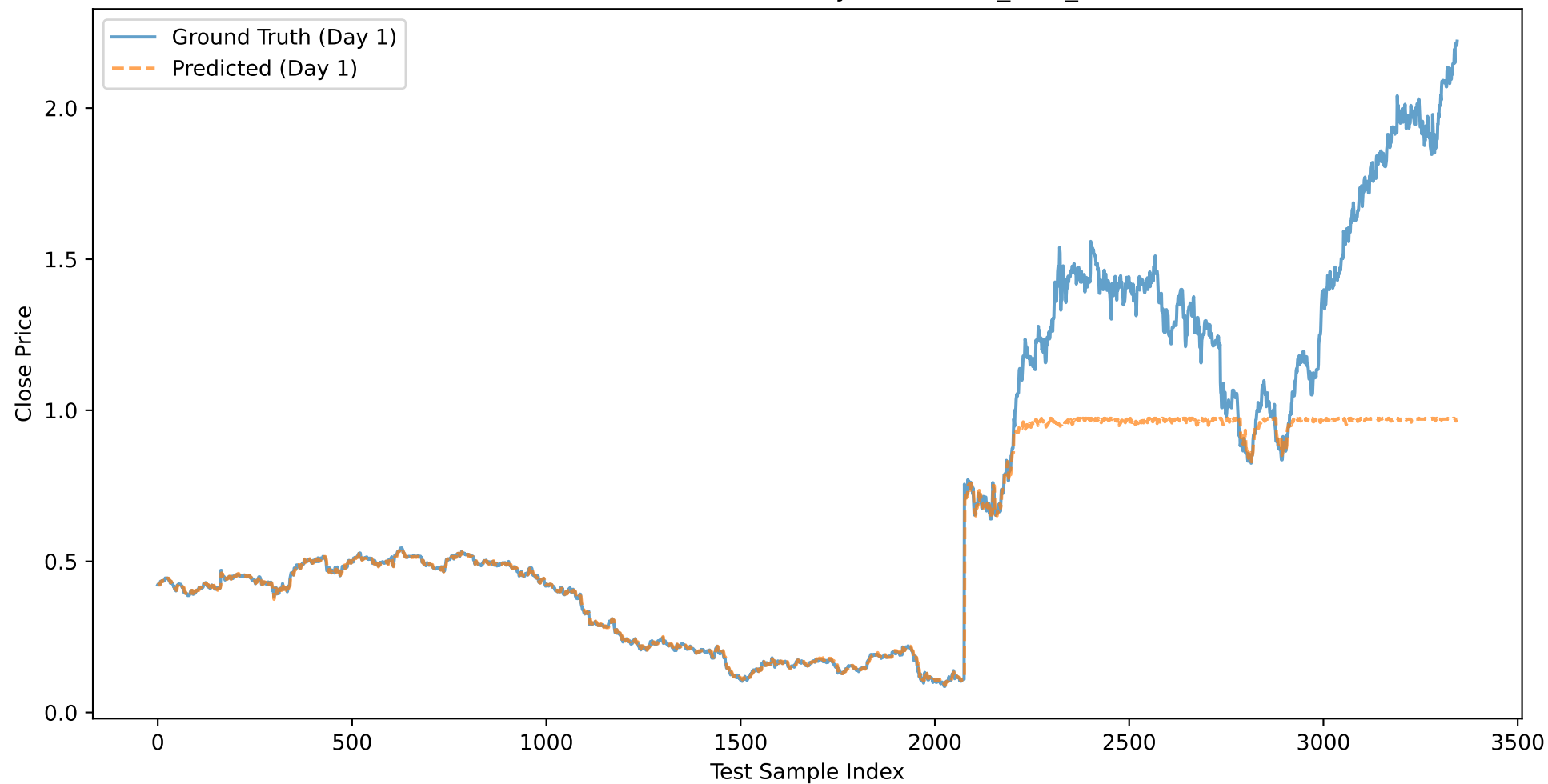
GE: Close Price Prediction (Day 1) - NOVEL_XGB_CLOSE
