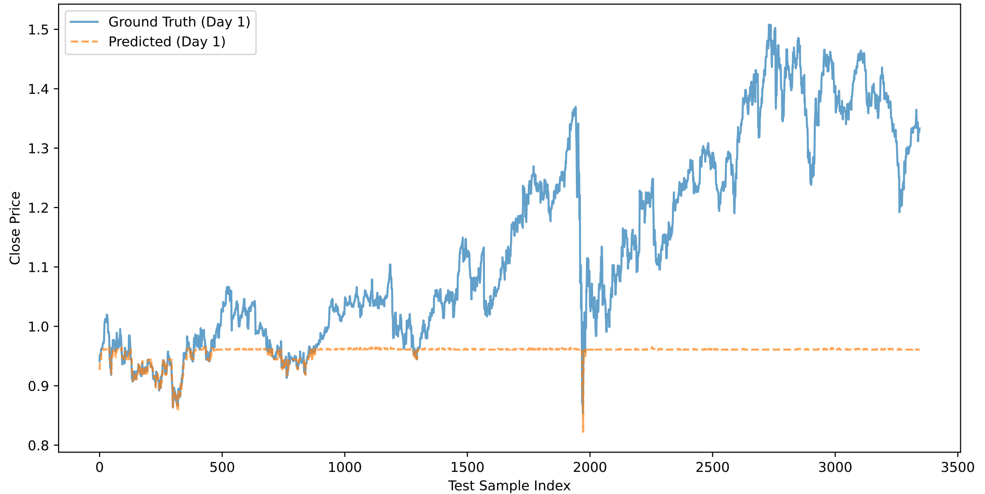
KO: Close Price Prediction (Day 1) - BASELINE_XGB_CLOSE
