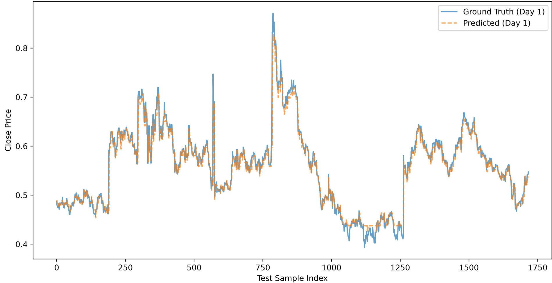
BIIB: Close Price Prediction (Day 1) - BASELINE_XGB_CLOSE
