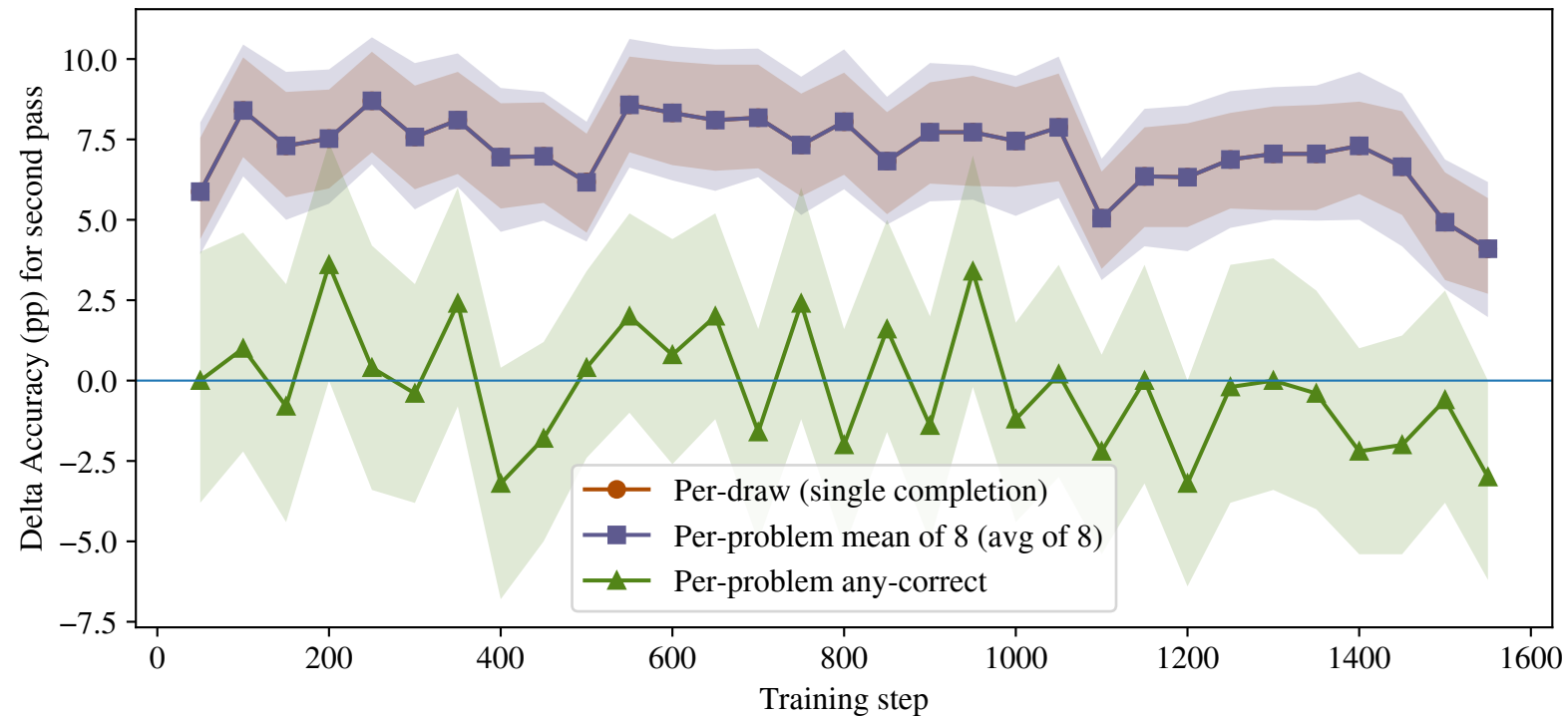
Stepwise \Delta — overlay of per-draw / mean-of-8 / any-correct (95% bootstrap CIs)
