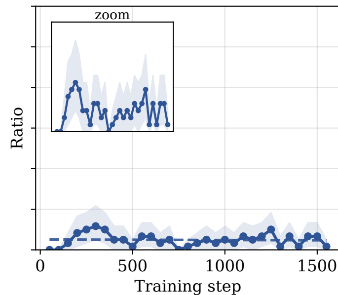
Formal "Aha!" (problem ratio per step) MATH-500, Qwen2.5-1.5B
