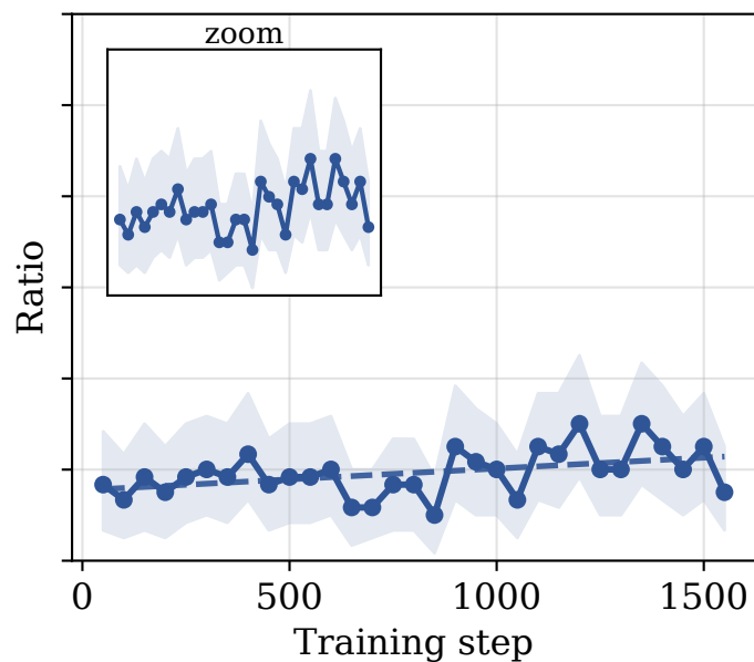
LLM-Detected "Aha!" (problem ratio per step) MATH-500, Qwen2.5-1.5B
