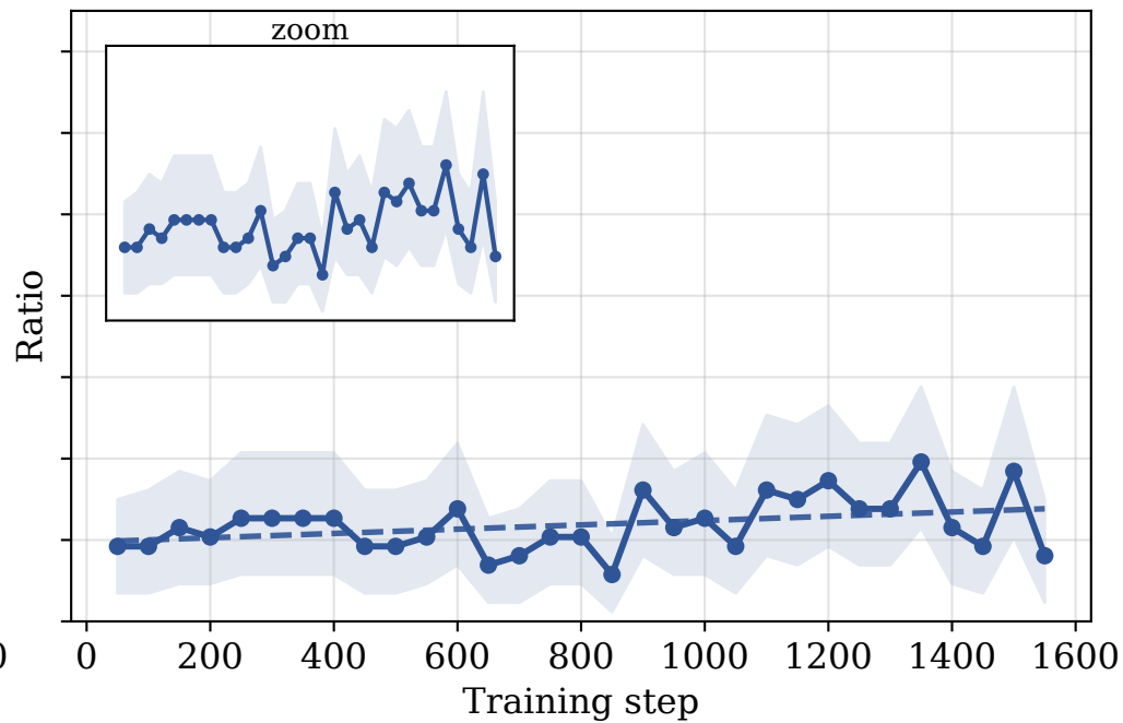
LLM-Detected "Aha!" (problem ratio per step) MATH-500, Qwen2.5-1.5B
