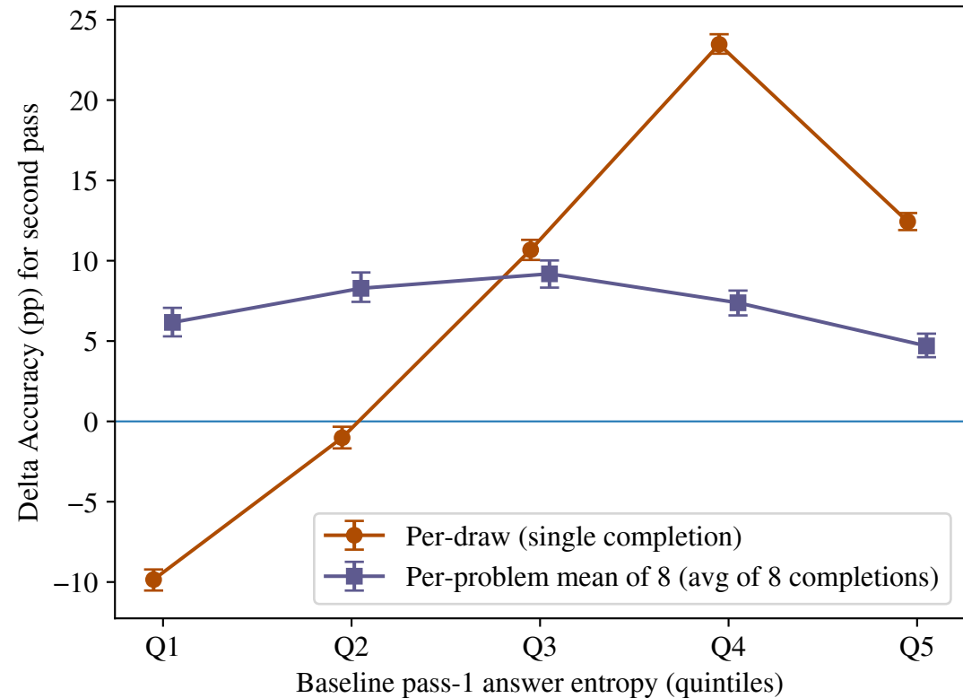
Uncertainty buckets: Forced Aha gains by entropy
