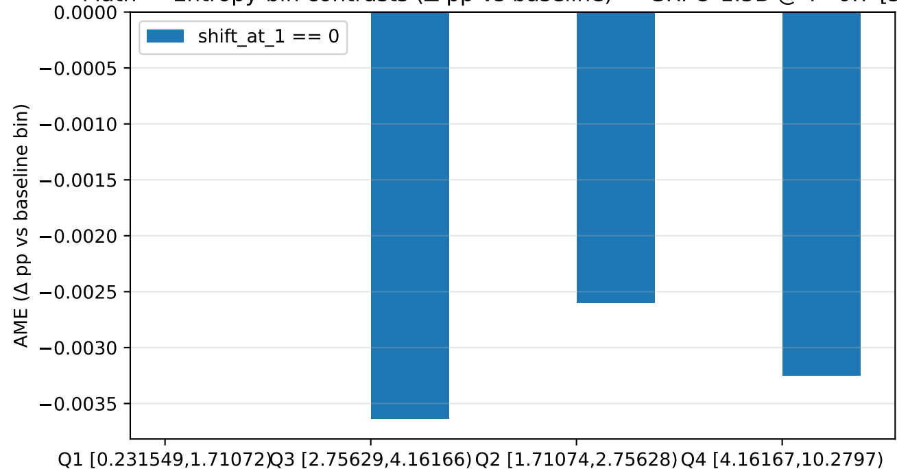
Math — Entropy-bin contrasts ( \Delta pp vs baseline) — GRPO-1.5B @ T=0.7 [sum]
