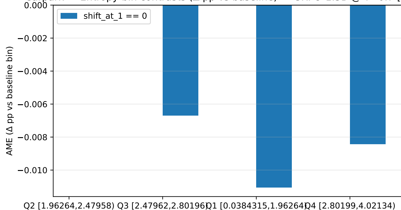
Carpark — Entropy-bin contrasts ( \Delta pp vs baseline) — GRPO-1.5B @ T=0.7 [think]
