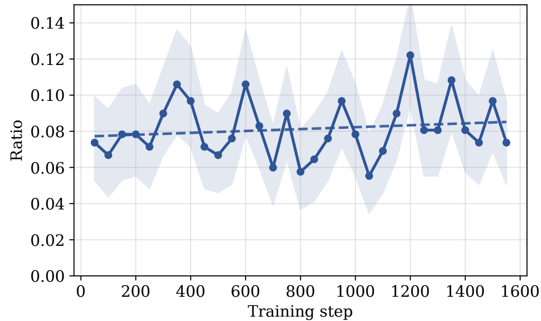
Words of "Aha!" String Detection (problem ratio per step) MATH-500, Qwen2.5-1.5B
