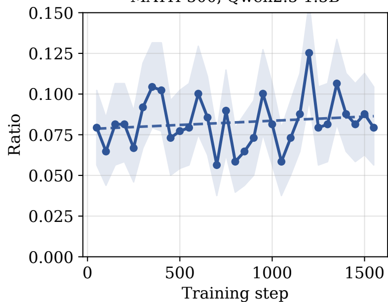
Words of "Aha!" String Detection (problem ratio per step) MATH-500, Qwen2.5-1.5B
