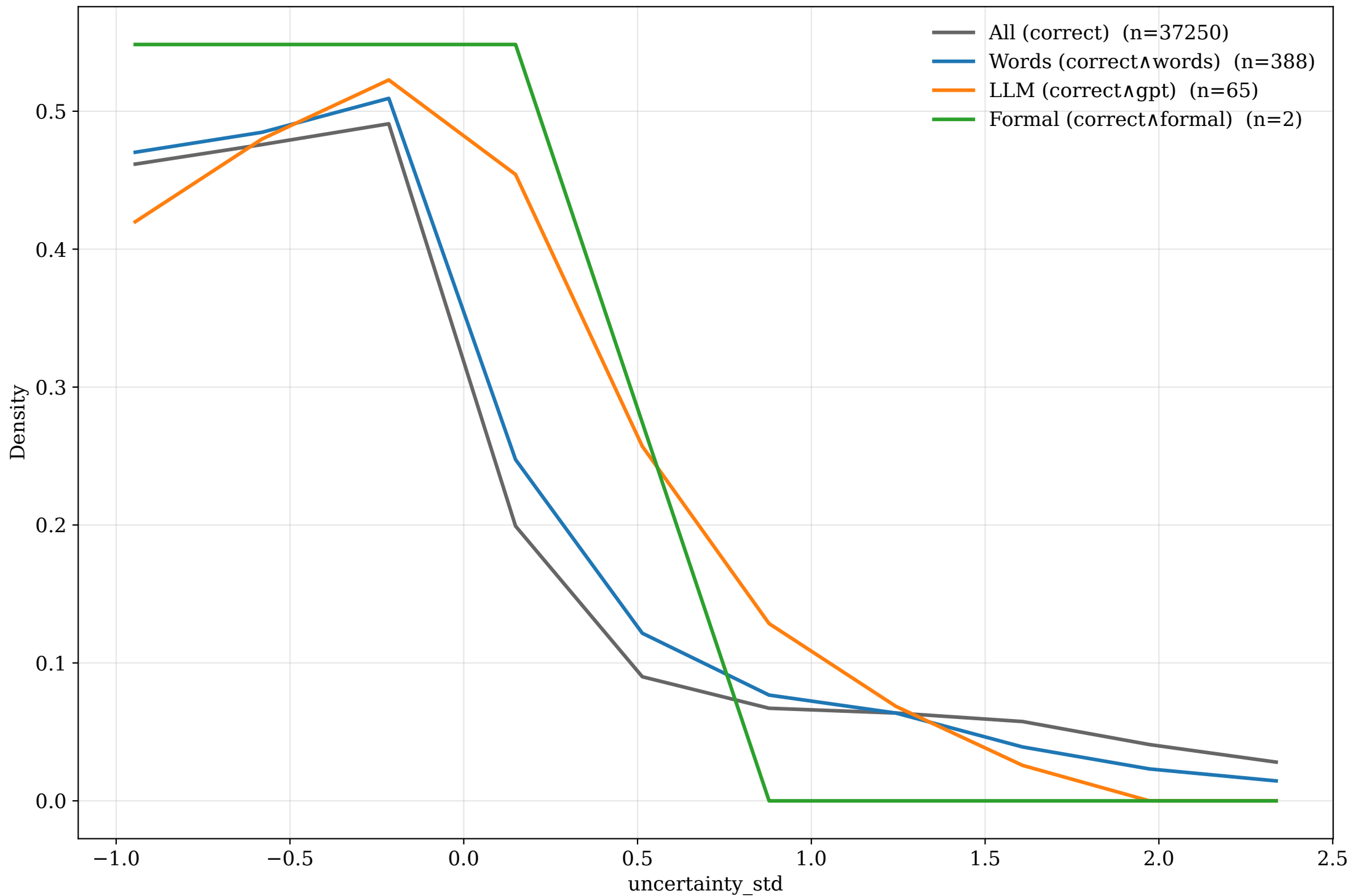
Area-normalized density of uncertainty_std (CORRECT only) MATH-500, Qwen2.5-1.5B
