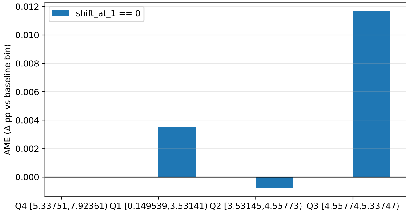
Carpark — Entropy-bin contrasts ( \Delta pp vs baseline) — GRPO-1.5B @ T=0.7 [sum]
