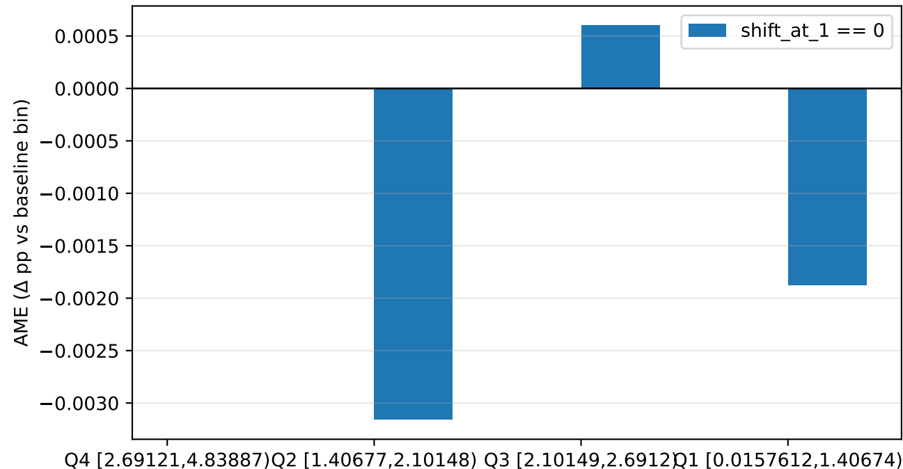
Carpark — Entropy-bin contrasts ( \Delta pp vs baseline) — GRPO-1.5B @ T=0.7 [answer]
