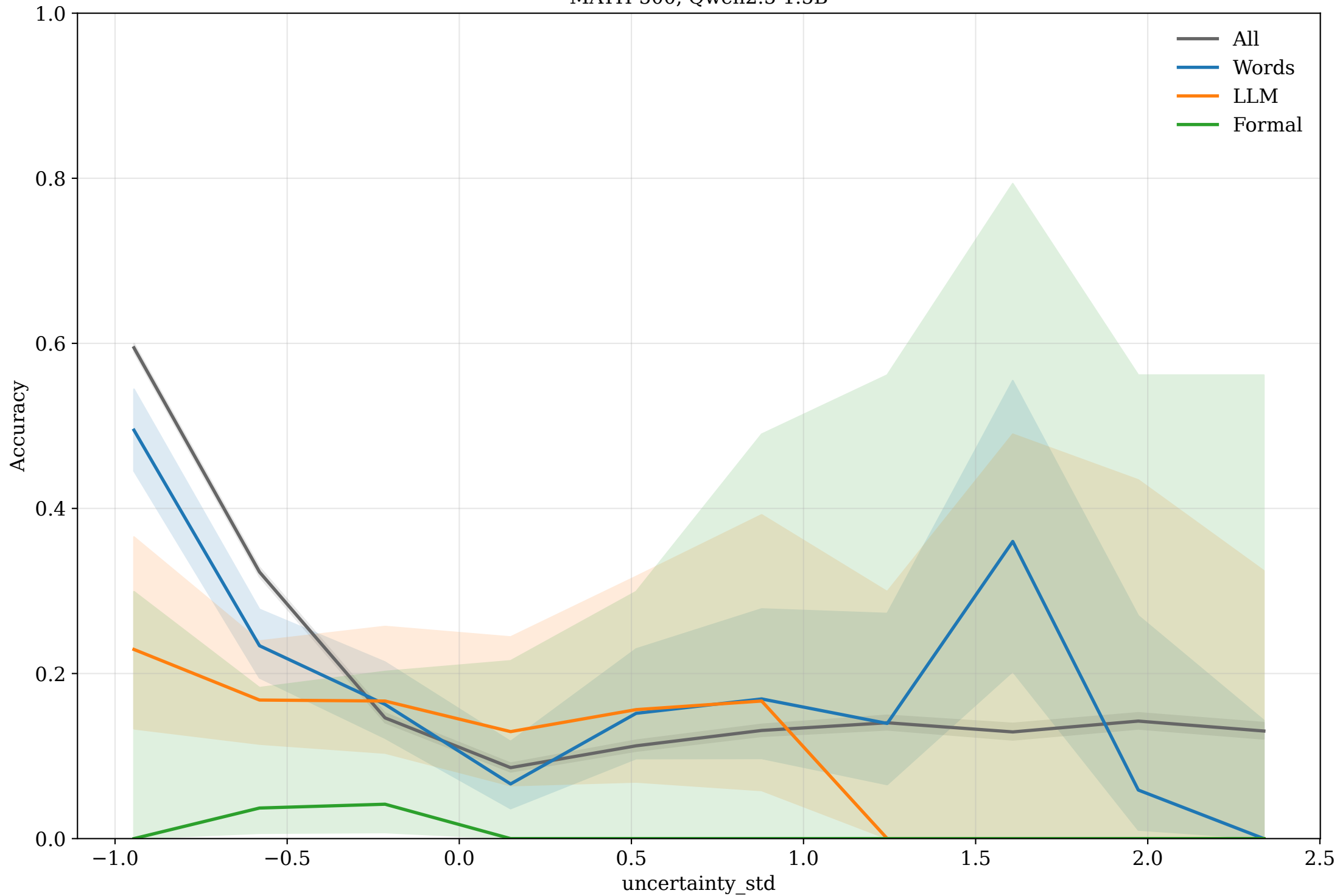
Per-bin accuracy with Wilson 95% CIs MATH-500, Qwen2.5-1.5B
