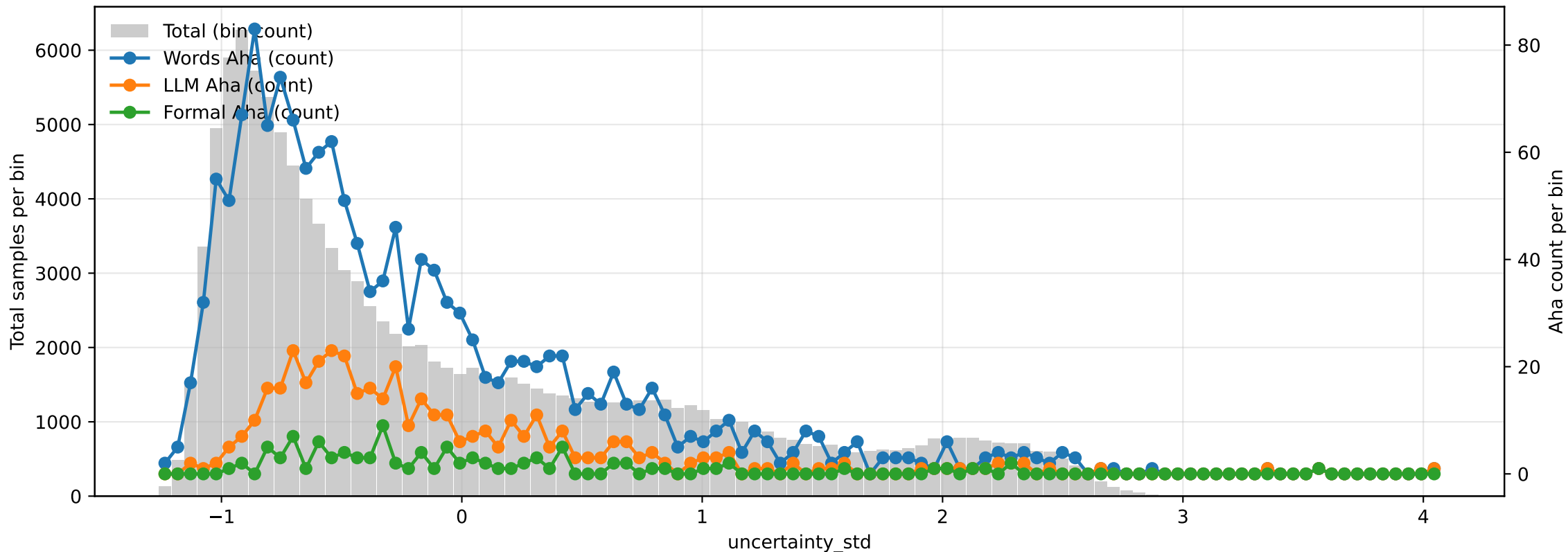
Uncertainty histogram (bins=100) with Aha counts MATH-500, Qwen2.5-1.5B
