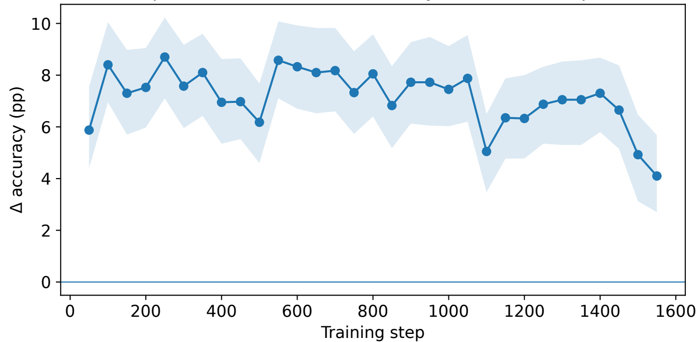
Stepwise \Delta — Per-draw accuracy (95% bootstrap CI)
