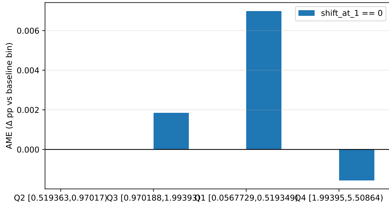
Math — Entropy-bin contrasts ( \Delta pp vs baseline) — GRPO-1.5B @ T=0.7 [answer]
