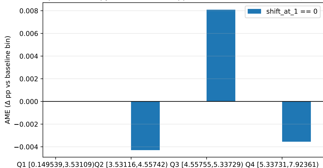
Carpark — Entropy-bin contrasts ( \Delta pp vs baseline) — GRPO-1.5B @ T=0.7
