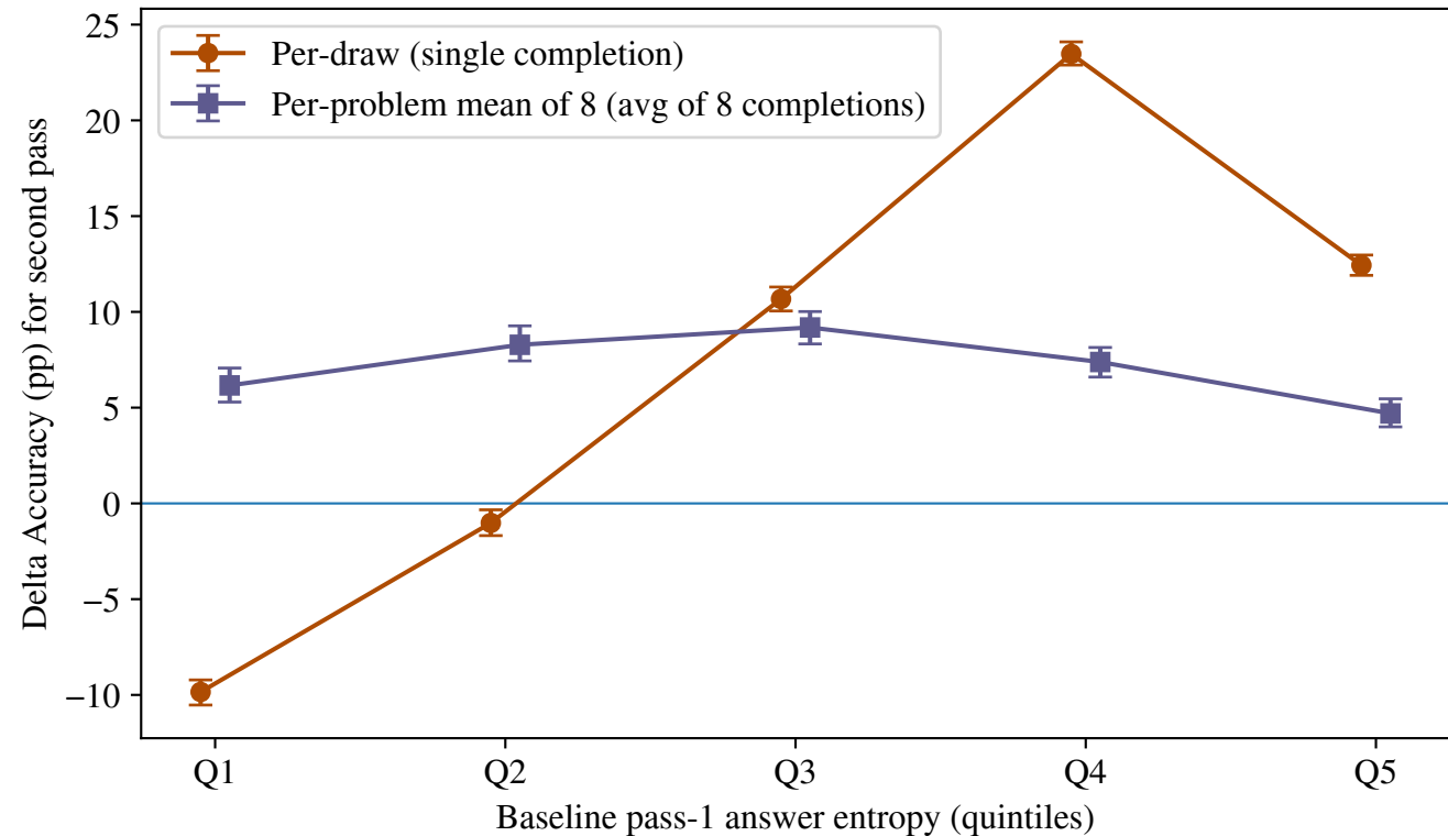
Uncertainty buckets: Forced Aha gains by entropy
