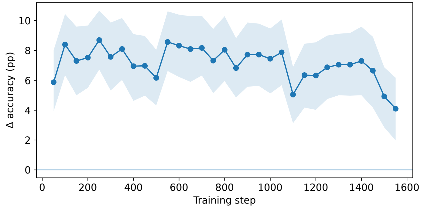
Stepwise \Delta — Per-problem mean of 8 (95% bootstrap CI)
