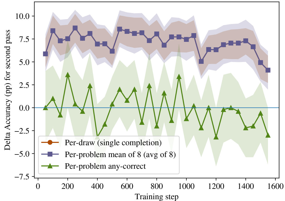
Stepwise \Delta — overlay (95% bootstrap CIs)
