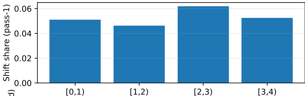
(B) Triggering reconsideration helps only when prior \geq 1/8
