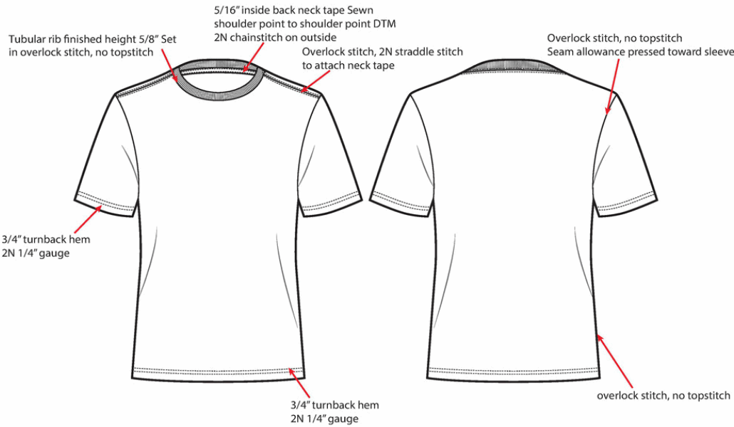
GBU Standard SS Tee Construction
