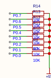
P0.x的上拉电阻
