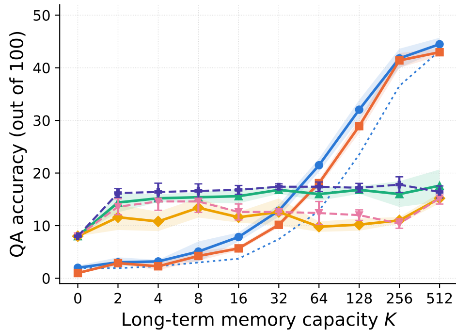
Train
