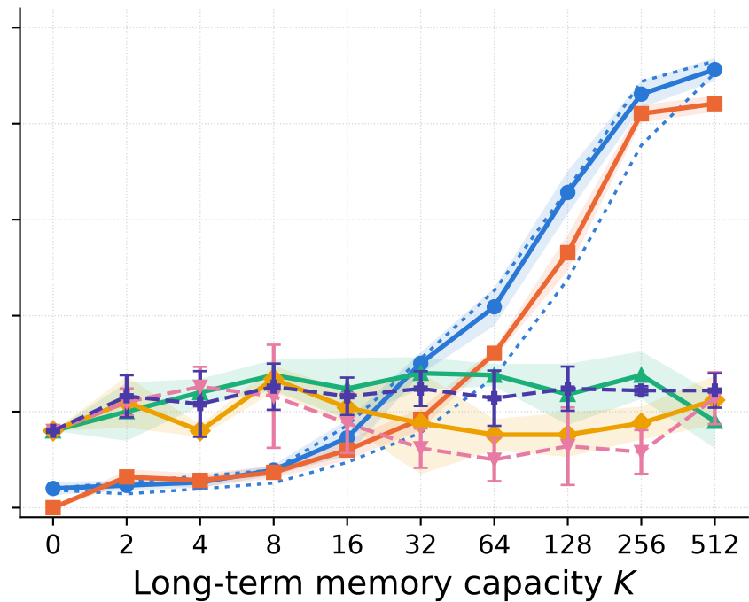
Test (held-out)
