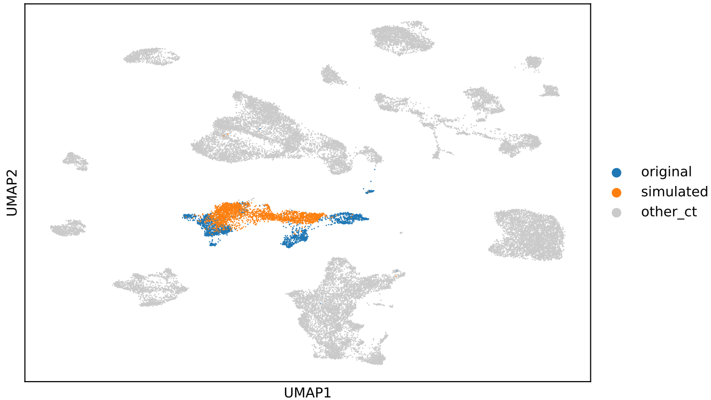
original + simulated B_cell (filtered)
