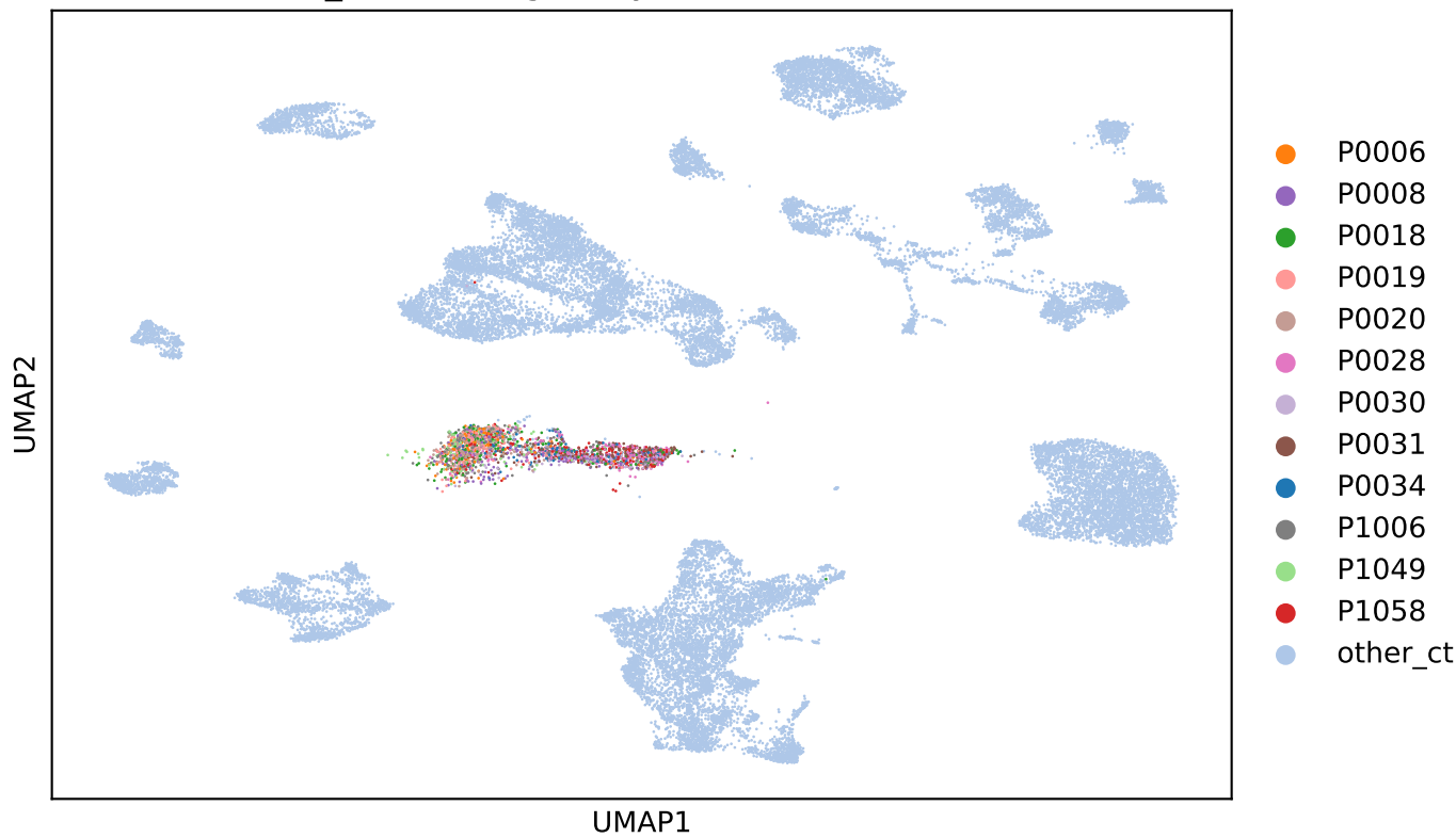
B_cell heterogeneity in simulated adata
