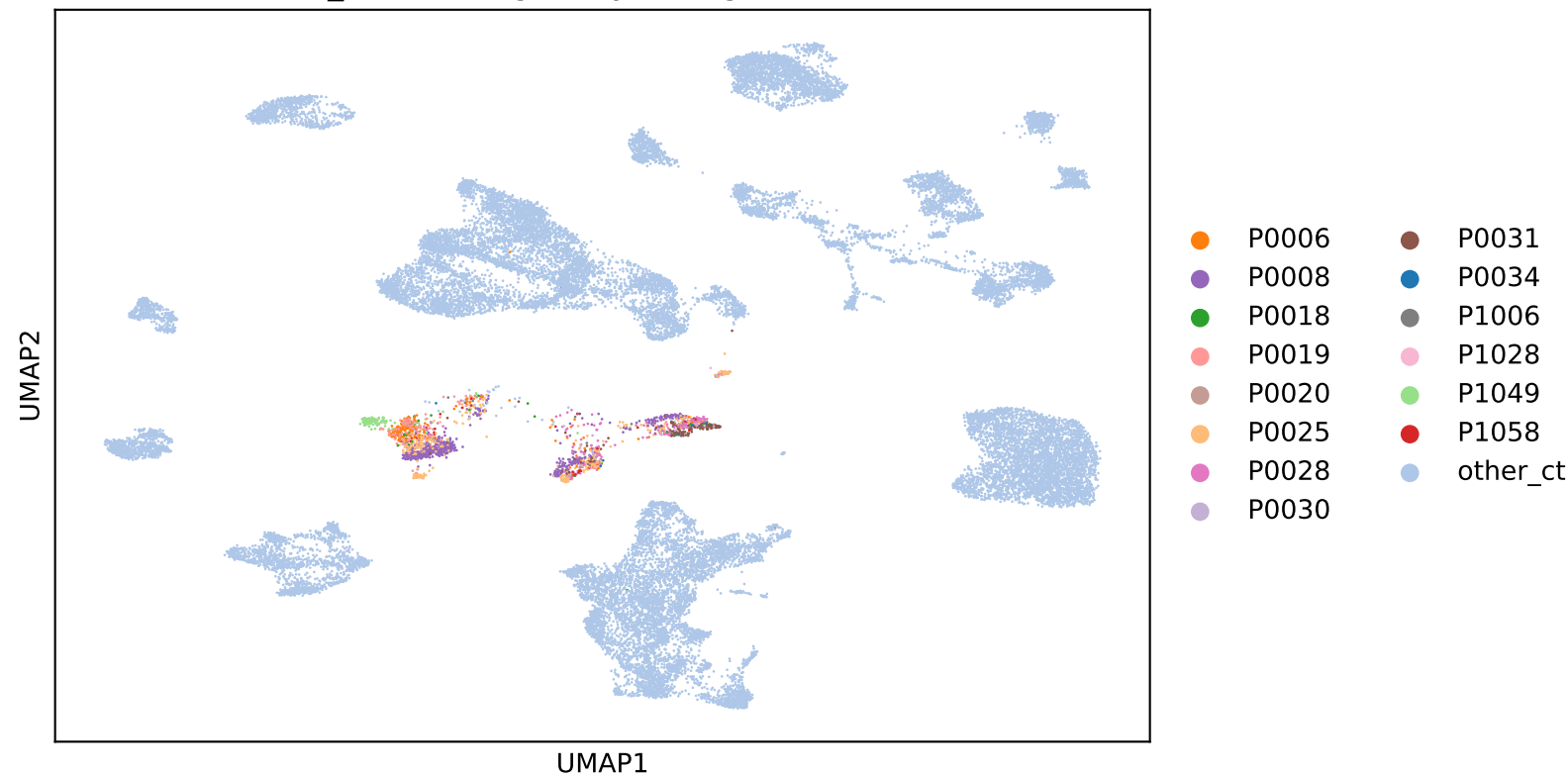
B_cell heterogeneity in original adata
