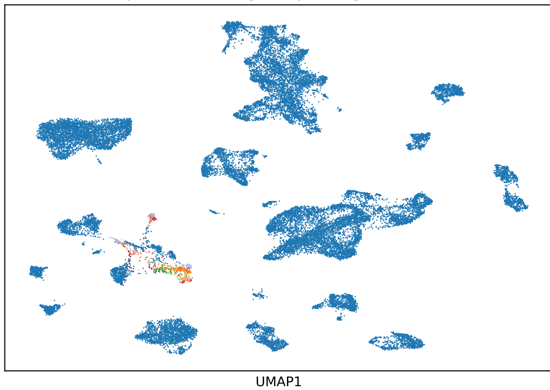
Epithelial heterogeneity in original adata
