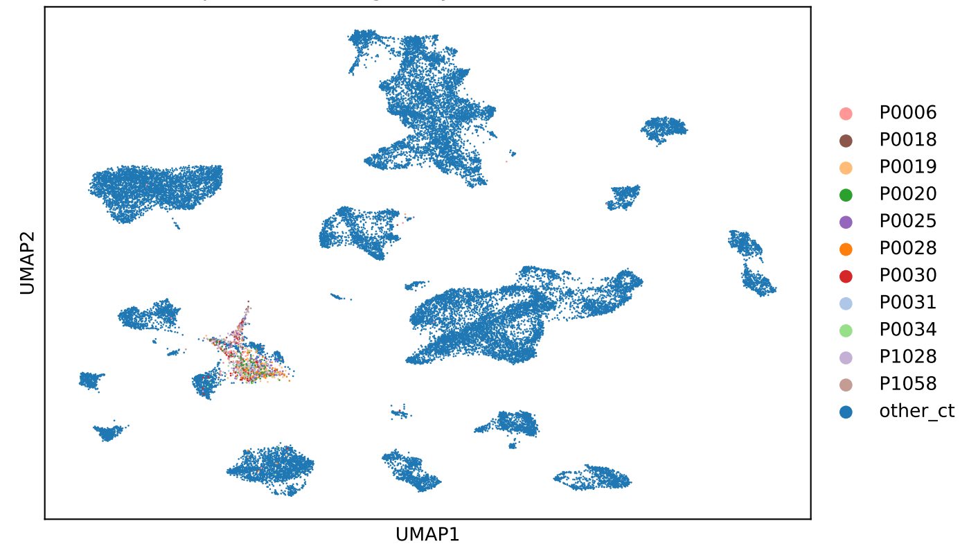
Epithelial heterogeneity in simulated adata
