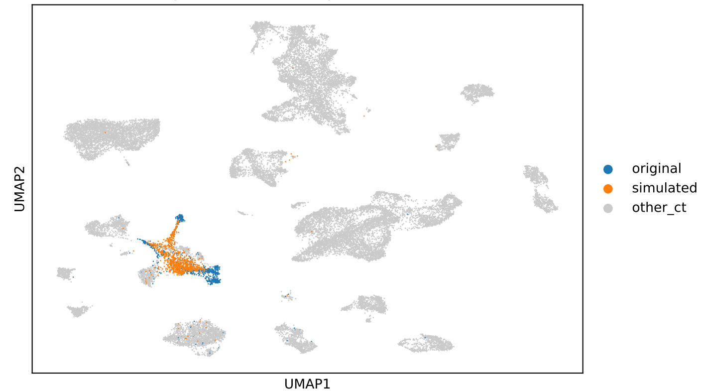
original + simulated Epithelial (filtered)
