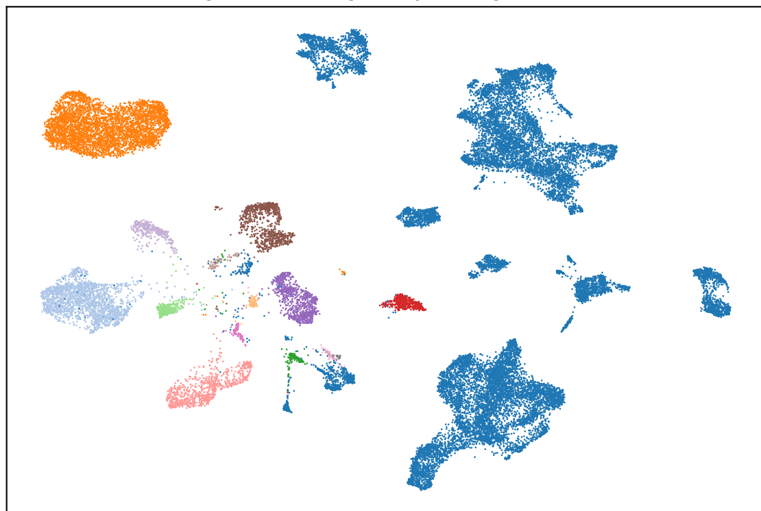
Malignant heterogeneity in original adata
