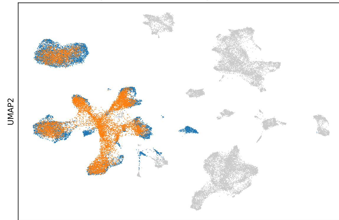
original + simulated Malignant (filtered)
