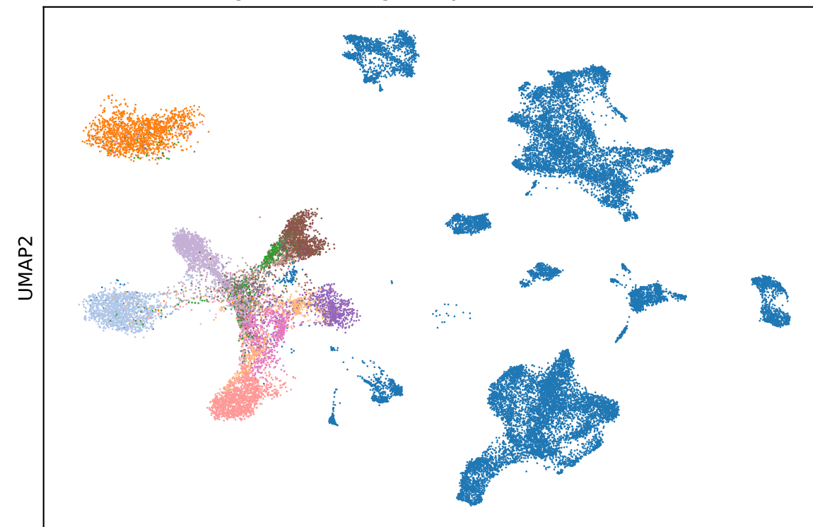
Malignant heterogeneity in simulated adata
