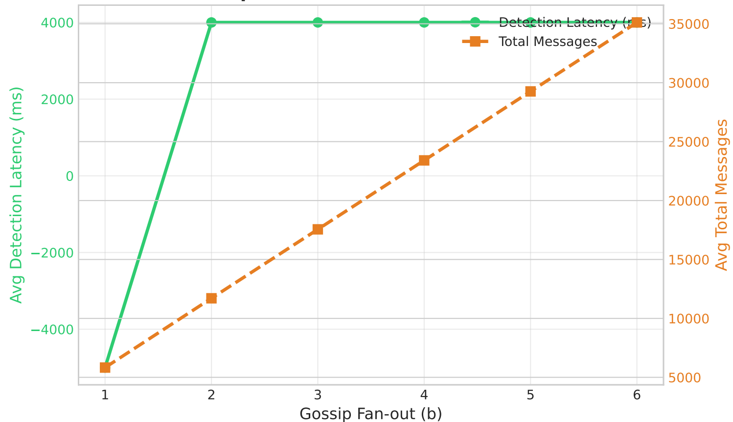
Effect of Gossip Fan-out (b) on Detection Performance
