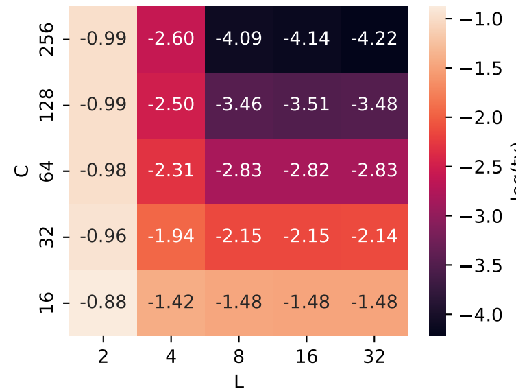
BLR Learnable
