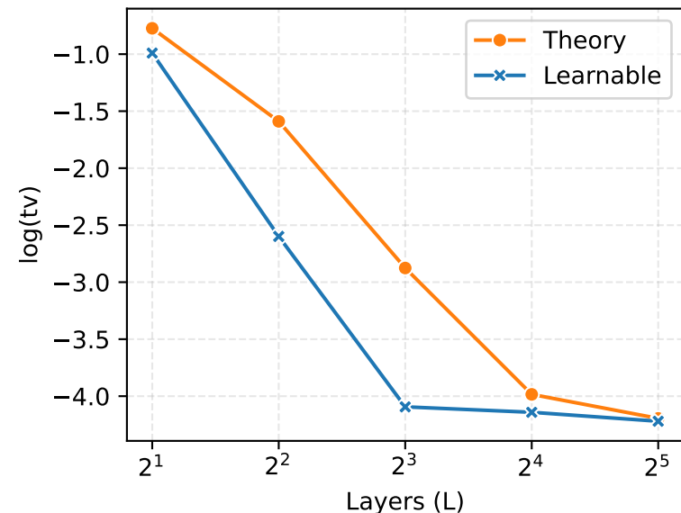
Fixed C = 256
