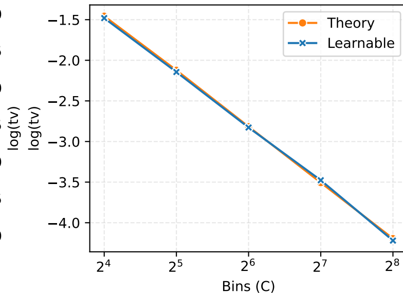
Fixed L = 32
