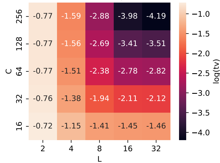
BLR Theory
