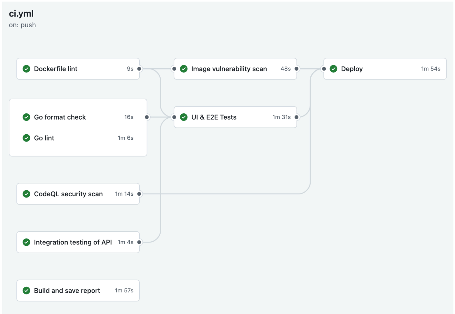
Figure 2: CI/CD pipeline flow diagram
