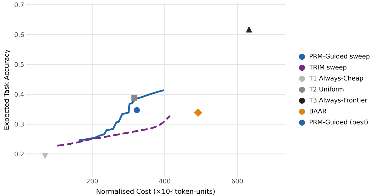
Cost-Accuracy Pareto Frontier
