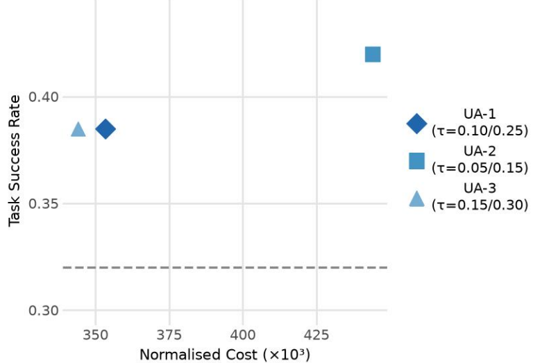
Uncertainty-Adaptive Thresholds
