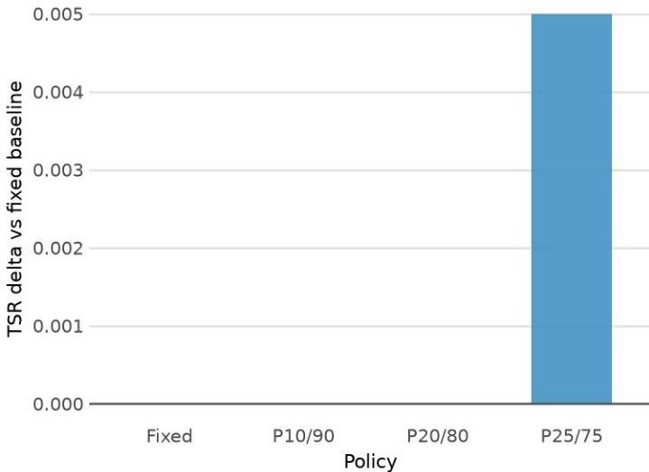
Percentile Dynamic Thresholds
