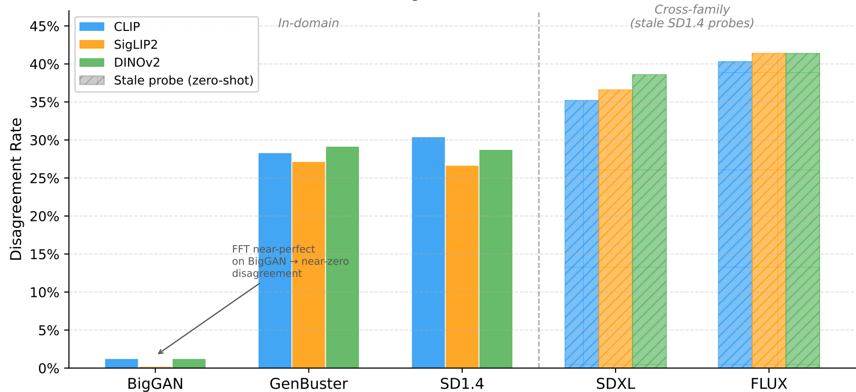
FFT-Semantic Disagreement Rate Across Datasets
