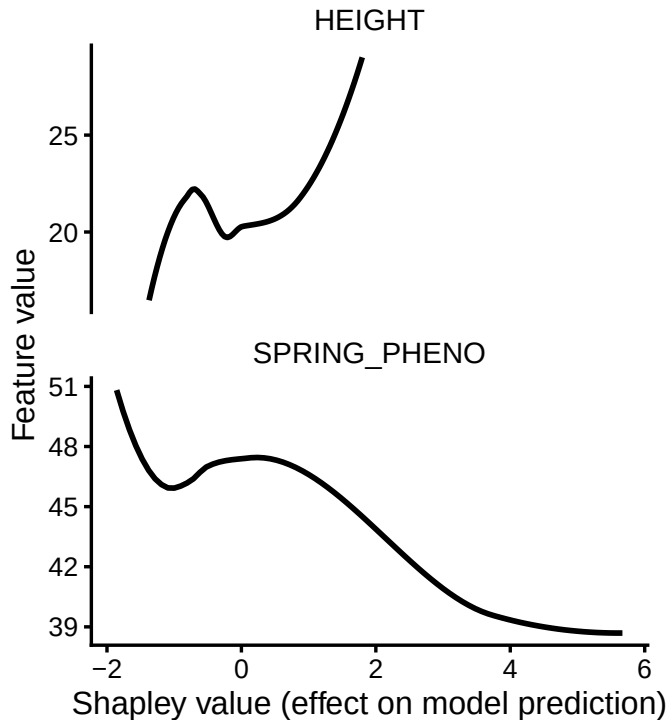
Mature acorns (litter traps)
