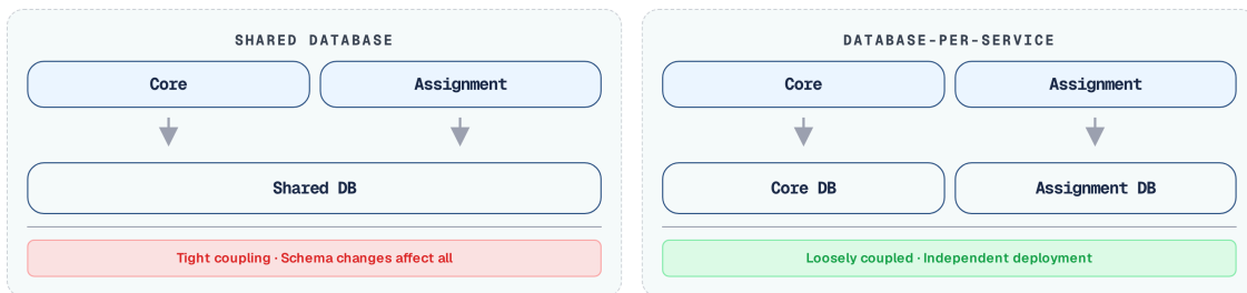
Hình 10.3: Shared Database (coupled) vs Database-per-Service (decoupled)
