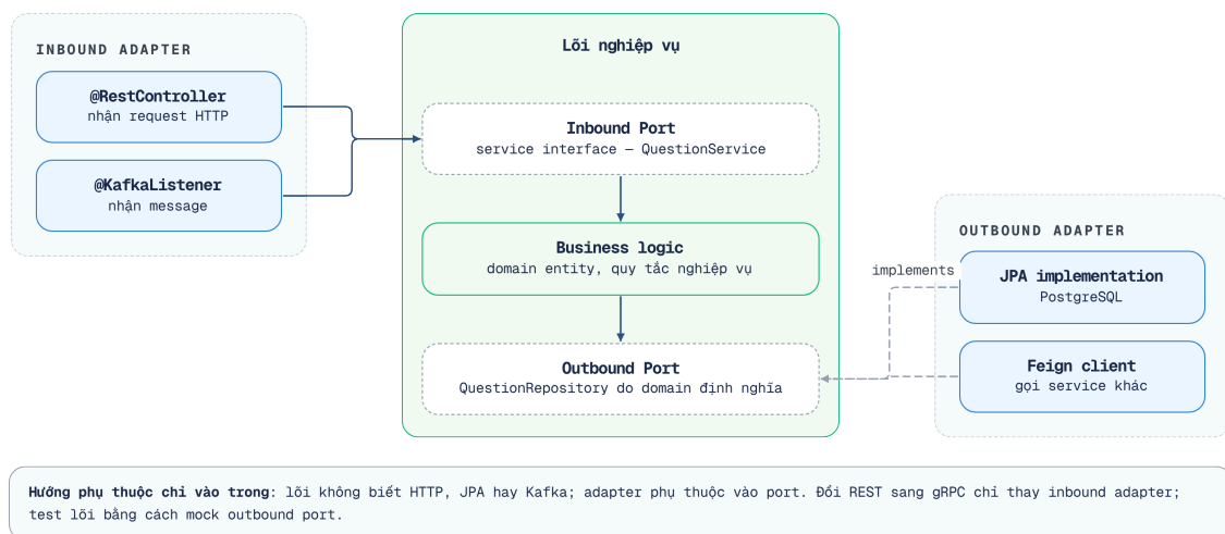
Hình 3.5: Hexagonal Architecture cho Core Service trong KBM
