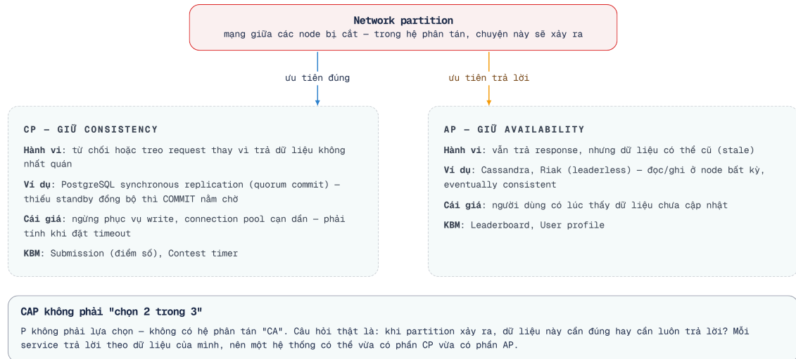
Hình 7.3: CAP Theorem – CP (chọn consistency) vs AP (chọn availability) khi partition
