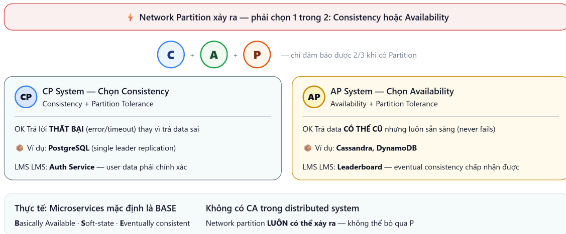
Hình 7.3: CAP Theorem — CP (chọn consistency) vs AP (chọn availability) khi partition
