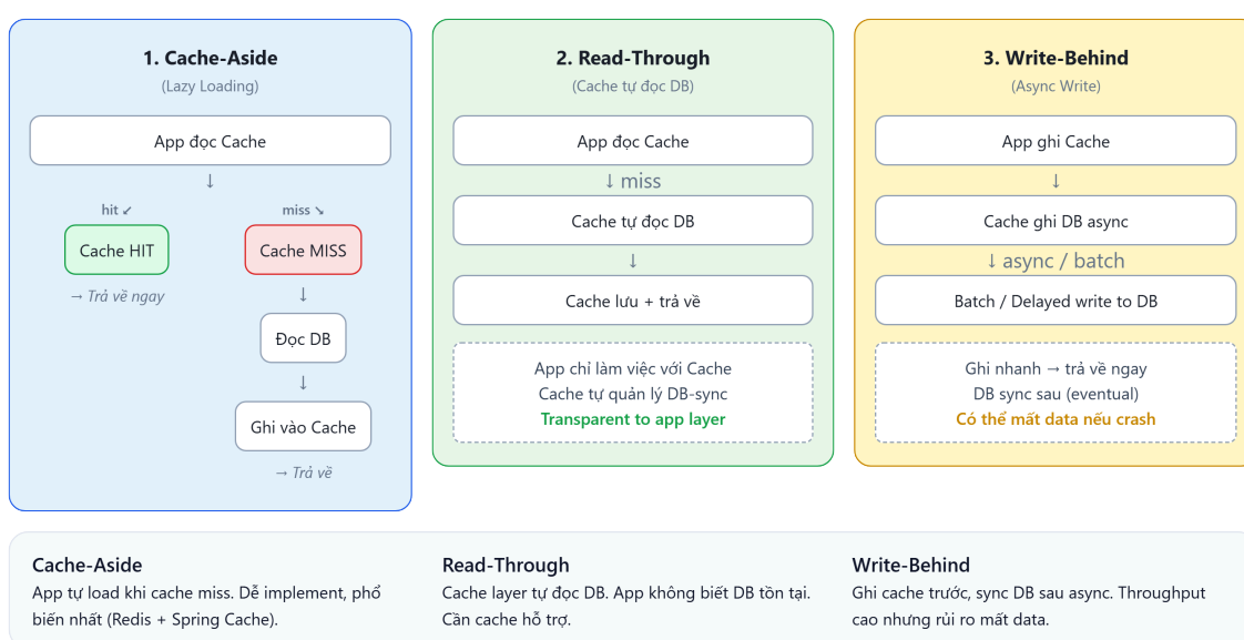
Hình 7.4: Ba caching patterns — Cache-Aside, Read-Through, Write-Behind
