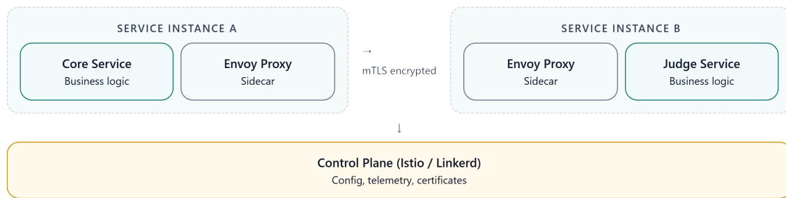
Hình 12.7: Sidecar Pattern — Proxy xử lý infrastructure concerns (mTLS, tracing)
