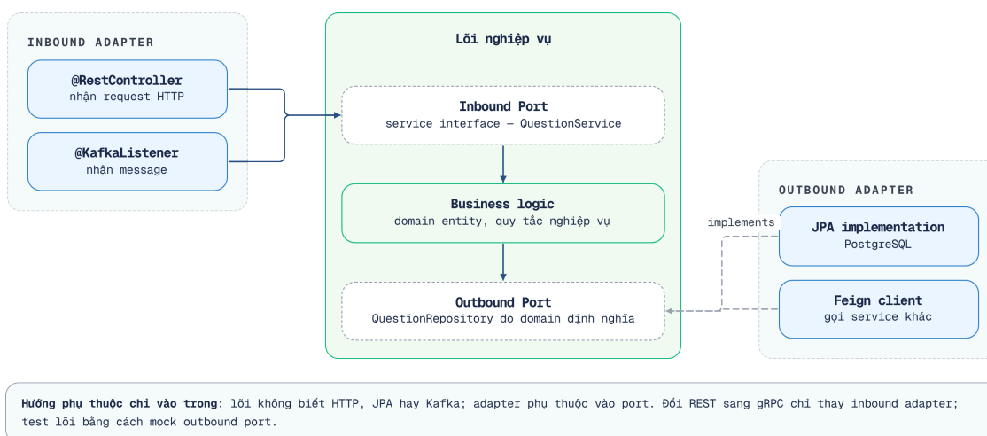
Hình 3.5: Hexagonal Architecture cho Core Service trong KBM
