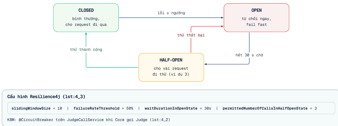
Hình 4.6: Circuit Breaker state machine — Closed, Open, Half-Open
