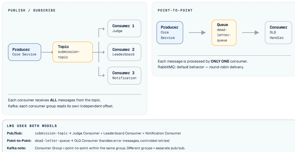
Hình 5.2: Point-to-Point (Queue) vs Publish/Subscribe (Topic)
