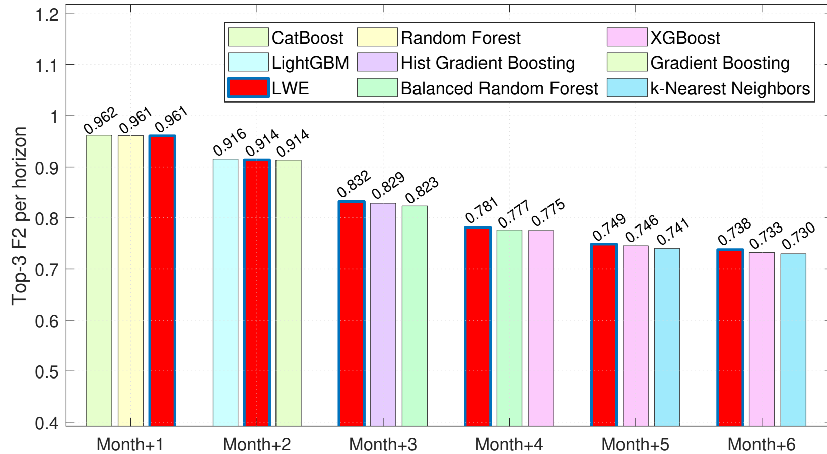
(C) Top-3 models per horizon — All datasets
