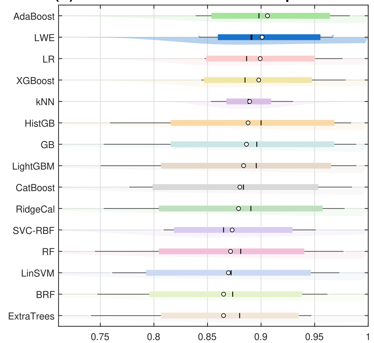
(C) France - Distribution of model performance
