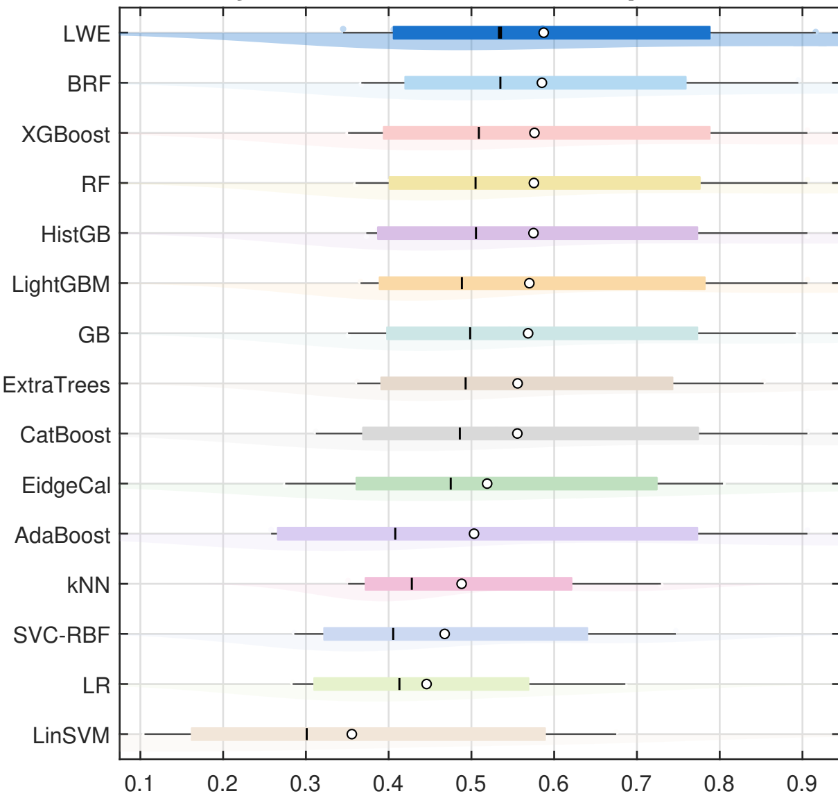
(A) Italy - Distribution of model performance
