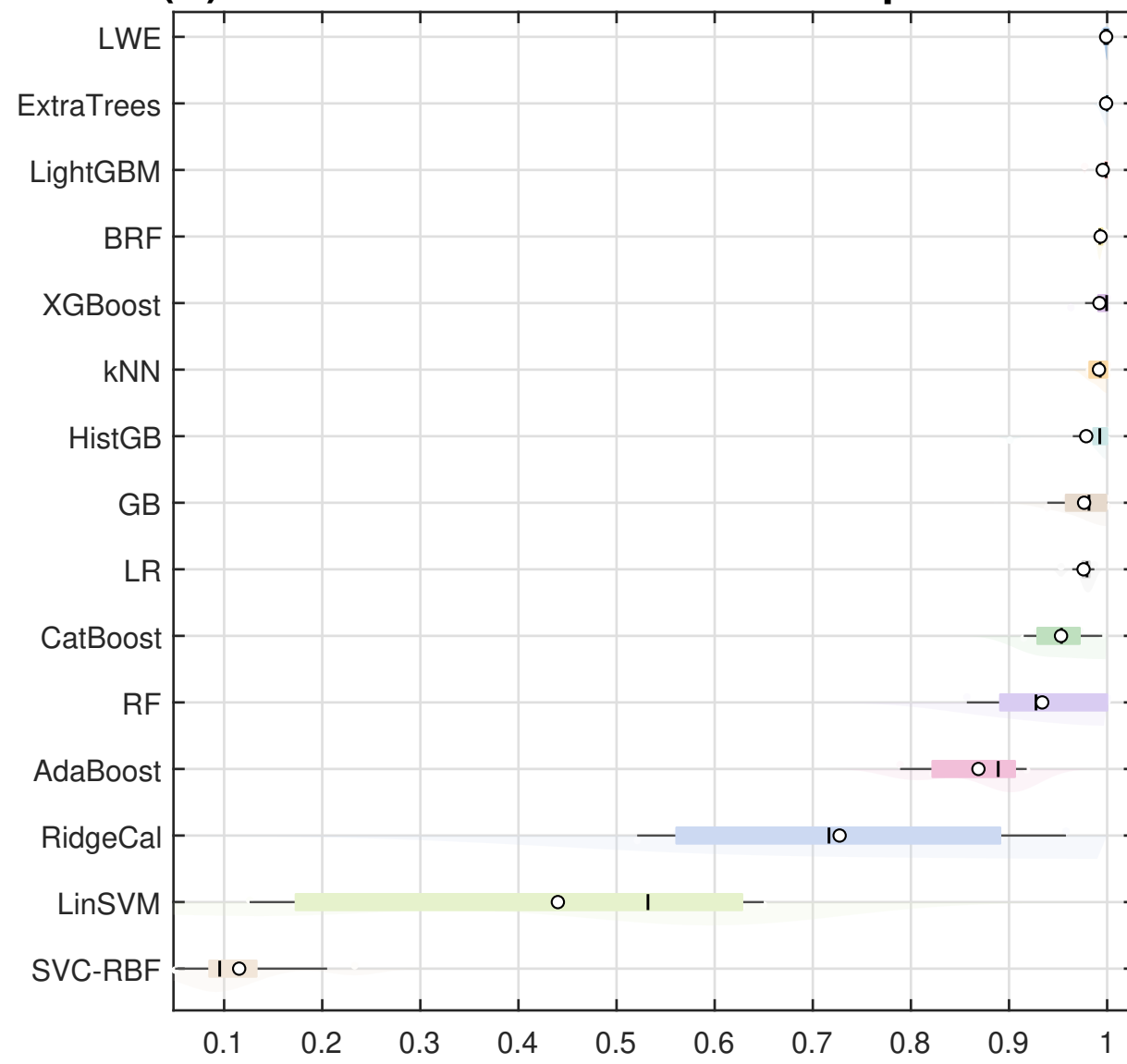
(B) Greece - Distribution of model performance
