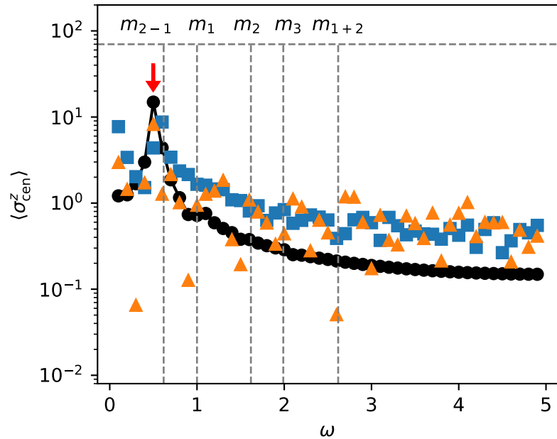
(a) initial state = |\uparrow \uparrow \downarrow \downarrow \downarrow \downarrow \uparrow \uparrow\rangle
