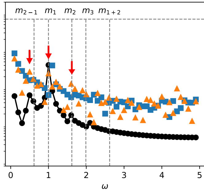
(b) initial state = |\uparrow \uparrow \uparrow \downarrow \downarrow \uparrow \uparrow \uparrow\rangle
