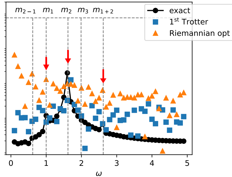
(c) initial state = |\uparrow \uparrow \uparrow \uparrow \uparrow \uparrow \uparrow \uparrow\rangle
