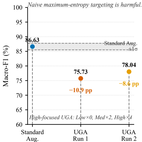
(B) UGA failure
