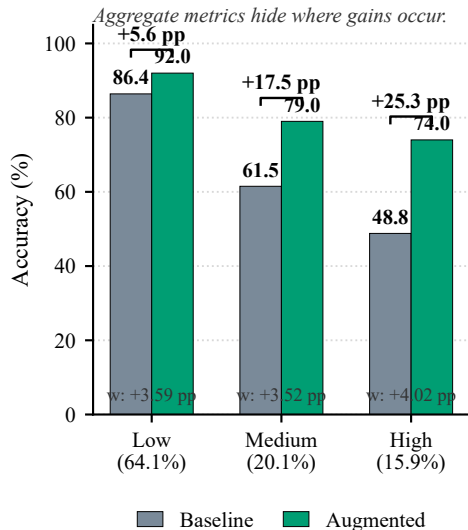
(A) Stratified gains
