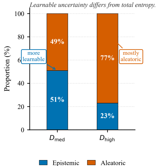
(C) BALD decomposition
