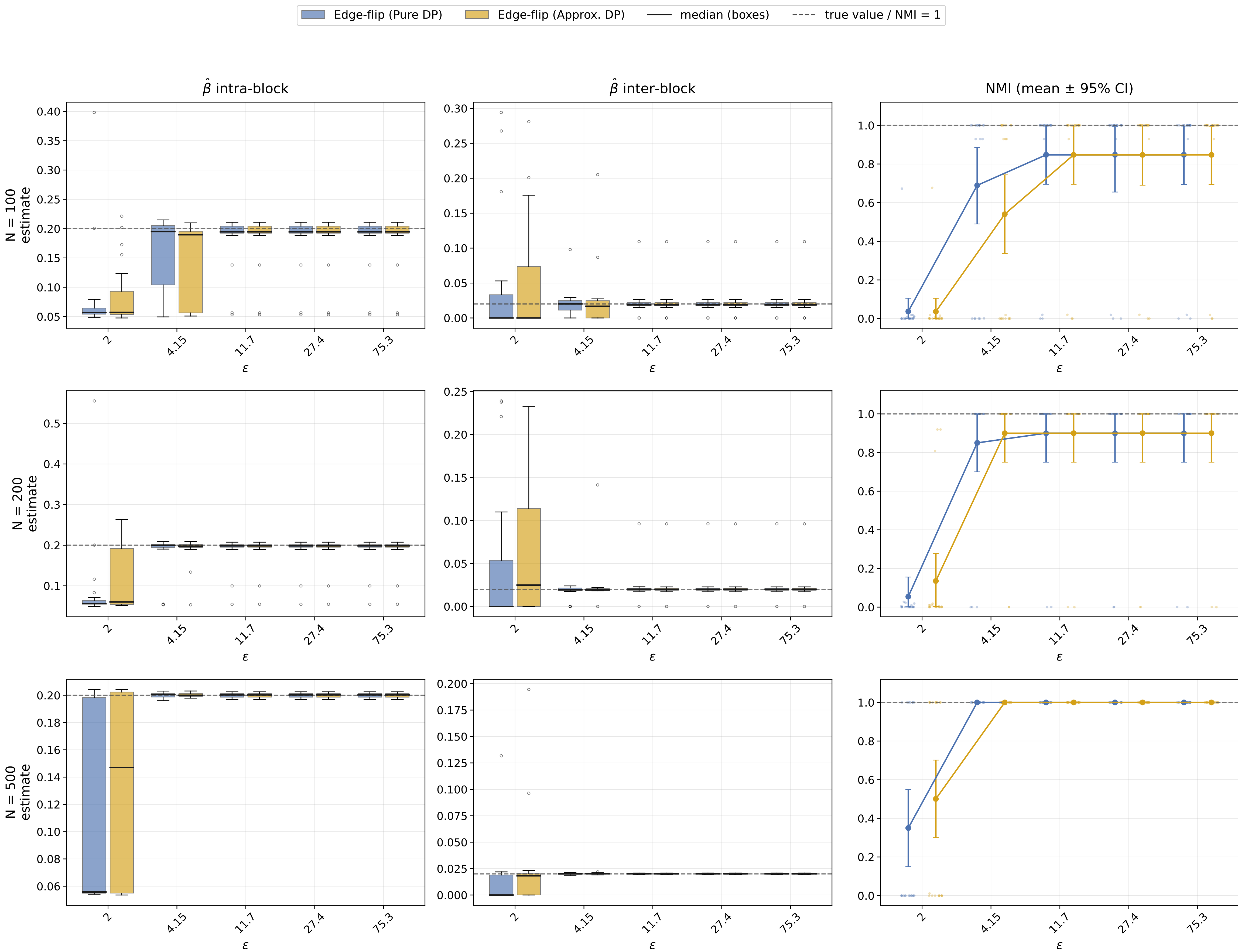
Edge-flip under Pure DP vs Approximate DP at matched \varepsilon ( \delta = 1e-05 )
