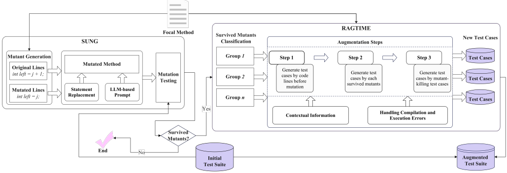
Fig. 1. Approach overview. The approach integrates mutation testing and test suite augmentation, where survived mutants from SUNG guide test case generation via RAGTIME.
