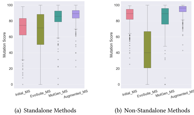
Fig. 10. Mutation score comparison. Results for MUTGEN and RAGTIME on non-standalone methods use 27 projects; EvoSuite uses 19.
