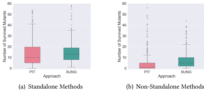
Fig. 8. Comparison of the number of survived mutants.
