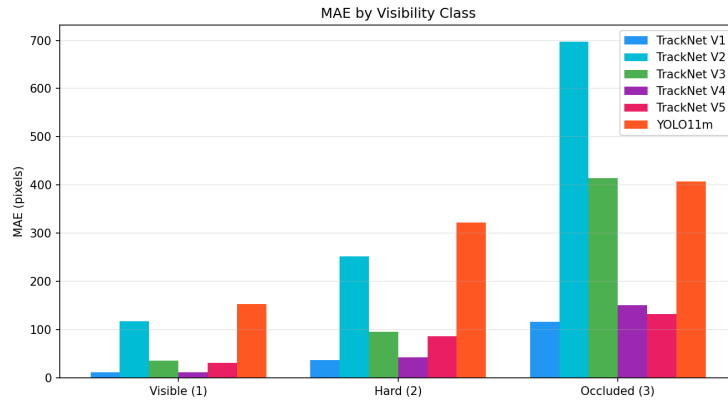
(d) Mean absolute error by visibility class.
