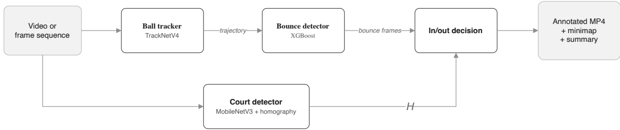
Figure 7.1: Data flow of the integrated pipeline. The ball tracker and the court detector both consume the input frames; the ball tracker yields a per-frame trajectory and the court detector yields a frame-pixel-to-court-metre homography H . The bounce detector marks bounce frames along the trajectory, and the in/out stage projects the ball’s position at each bounce through H and tests court-polygon containment. All outputs are composited into one annotated video with a top-down court minimap and a summary record.
