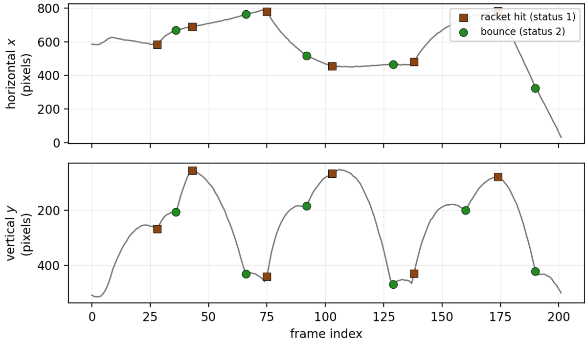
Figure 6.1: The bounce signature in the ball-coordinate time series, for one rally of the game7 test split with six bounces and six hits. The horizontal ( x ) and vertical ( y ) image coordinates are plotted against the frame index; the vertical axis is inverted so the court lies toward the bottom of the panel. Bounce frames (status 2) are marked in green and racket hits (status 1) in brown.
