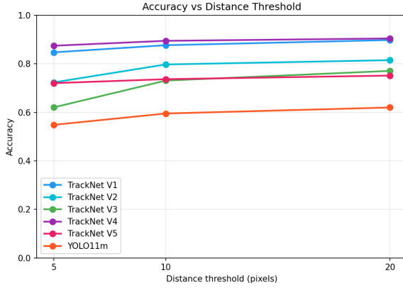
(a) Accuracy versus distance tolerance.
