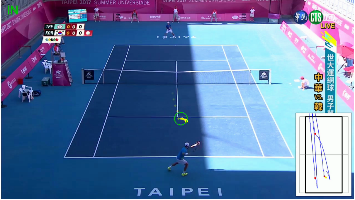
Figure 7.2: A representative frame from the end-to-end demonstration on a game10 test clip. The ball is tracked with a fading trail (yellow); a detected bounce is marked by an expanding ring on the court and announced by the banner at the top left, here IN (green). The court minimap composited into the bottom-right corner shows the singles and doubles court lines, the ball trajectory projected into court-metre space (blue), the bounce positions accumulated so far (red), and the current ball position (yellow). The line call is a qualitative geometric output, not a validated measurement (Section 7.2).
