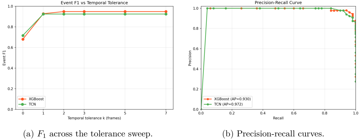
Figure 6.3: Bounce-detection comparison on the game7 test split, for the selected XGBoost model against the temporal network. (a) Event F_1 as the matching tolerance k widens from 0 (exact frame) to 7 frames. At the exact frame the temporal network achieves the higher F_1 (0.717 against XGBoost’s 0.680), but from k = 2 onward XGBoost leads, and both models plateau by k = 2 . (b) The precision-recall curves traced by sweeping the decode threshold, whose areas are the average precisions of Table 6.2: the temporal network encloses the larger area (AP 0.972 against 0.930).
