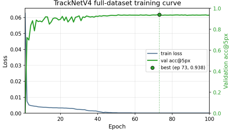
Figure 4.3: Training curve of the final TrackNetV4 on the full dataset split (game1–game9 for training and validation). The training loss (left axis) and validation accuracy at five pixels (right axis) are both plotted on linear scales against the epoch count. The training loss falls steeply over the first few epochs and then continues to decrease; validation acc@5px climbs to a plateau around 0.93 and peaks at 0.938 at epoch 73 (marked), the checkpoint carried forward for evaluation.
