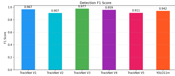
(c) Detection F_1 .
