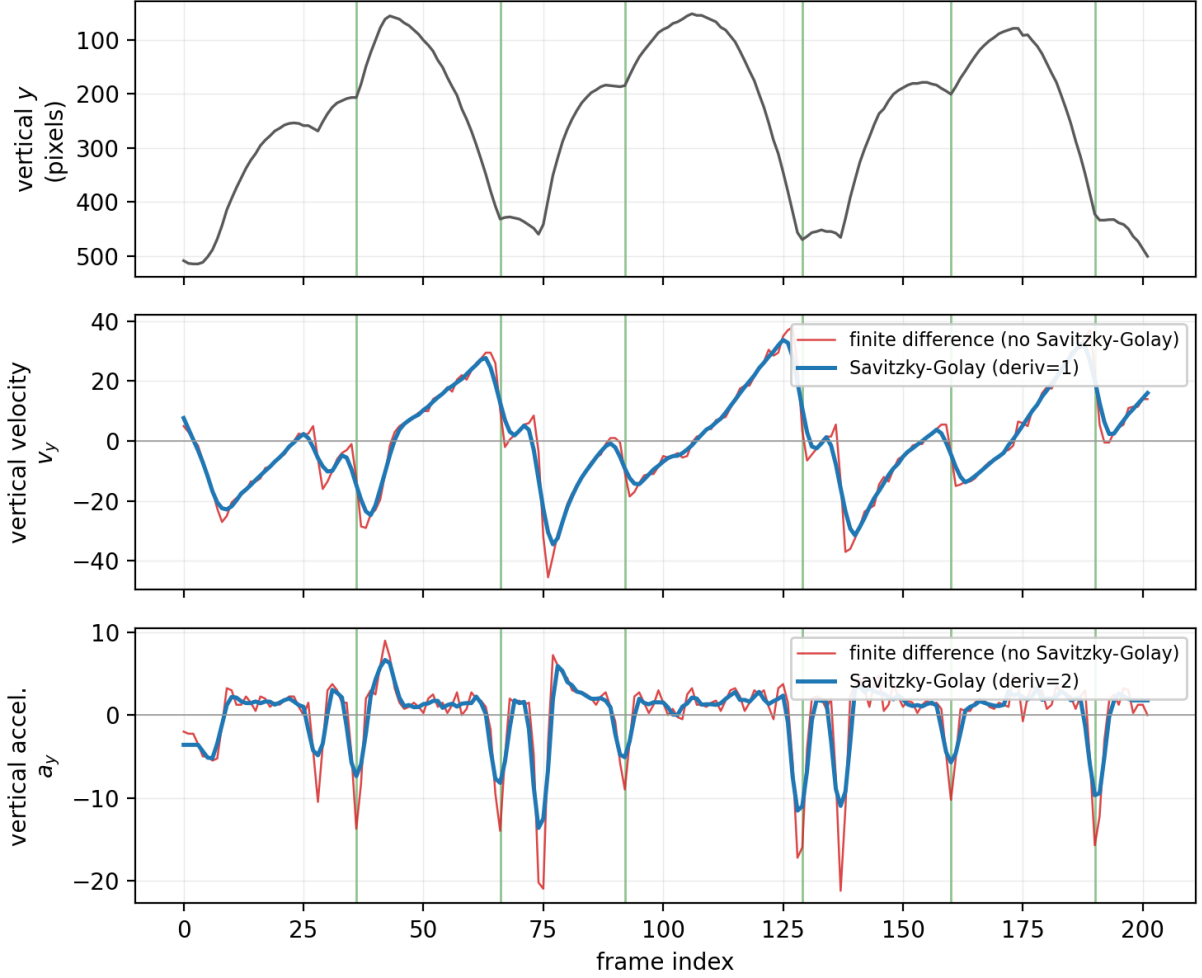
Figure 6.2: Velocity and acceleration recovered from the vertical ball trajectory of one rally, comparing a naive finite difference (red) with the Savitzky-Golay smoothing-differentiation filter (blue). Top: the vertical image coordinate y against the frame index, with bounce frames marked in green. Middle: the first derivative v_y . Bottom: the second derivative a_y . The finite difference amplifies the per-frame jitter in the tracked positions, most severely in the acceleration, while the Savitzky-Golay estimate keeps the reversal at each bounce and rejects the noise.
