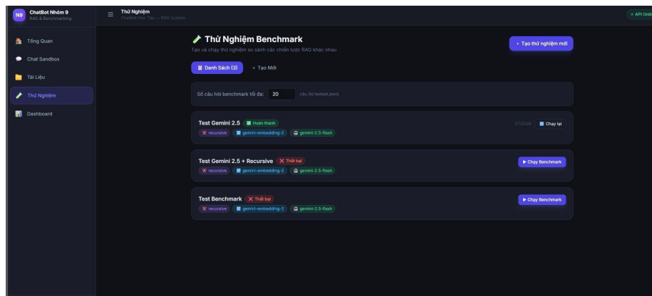
Figure 6.1: Chạy Benchmark
