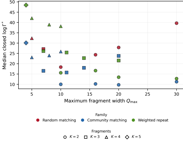
Fig. 5. E9 width-overhead tradeoff restricted to cells closed for all three seeds. Colors denote families; markers denote K . Each point is the median \log \Gamma^* for its cell. This avoids conditioning the plot on solver-successful seeds.
