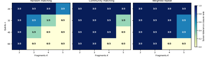
Fig. 4. E9 solver-tolerance closure counts under a 10-s SCIP limit. Each heatmap cell reports closed runs out of three fixed seeds. The boundary depends materially on graph family, K , and seed.
