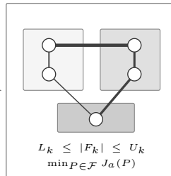
(c) K -way partition
