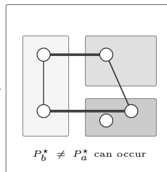
(g) New partition
