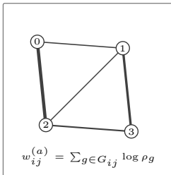
(b) Graph G^{(a)}
