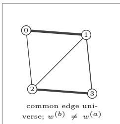
(f) Graph G^{(b)}
