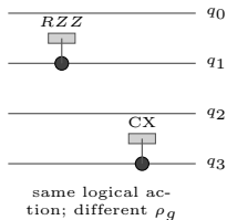
(e) Circuit b
