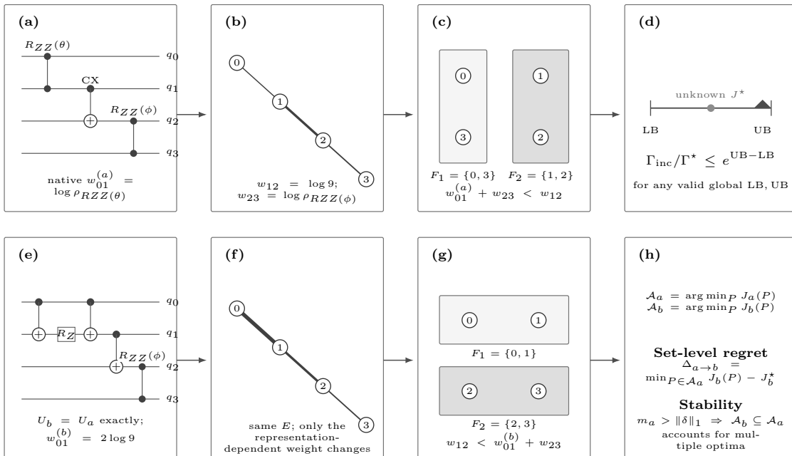
Schematic four-qubit witness: the gate identity is exact; edge width denotes independent-QPD log cost.
