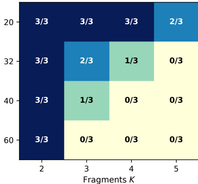
Random matching
