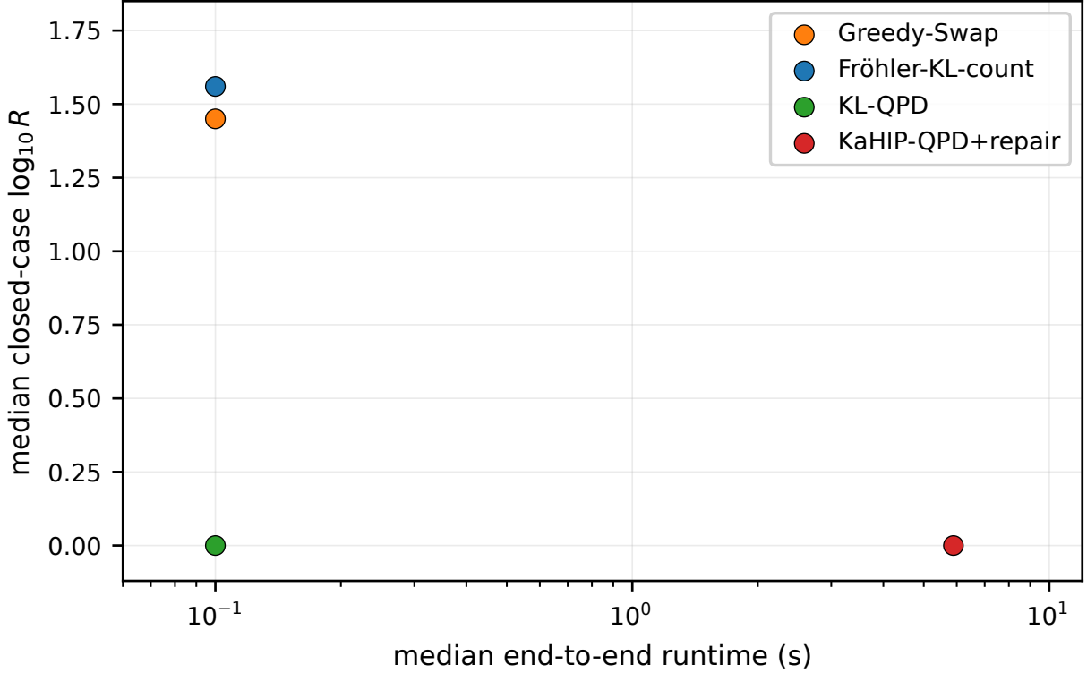
Figure 4: E9 closed-case median quality–runtime comparison. Greedy and KL use the shared 0.1-s budget; KaHIP has no binding-level native time limit and is shown for contextual runtime quality.
