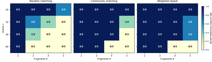
Figure 6: E9 solver-tolerance closure counts under a 10-s SCIP limit. Each heatmap cell reports closed runs out of three fixed seeds. The boundary depends materially on graph family, K , and seed.
