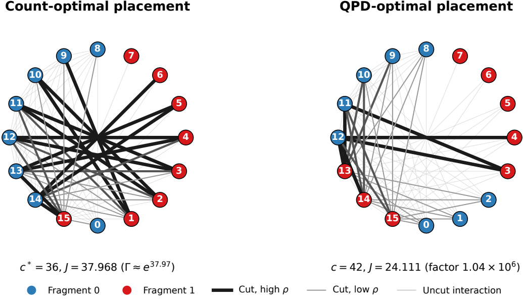
FIG. 2. Draper QFT-adder interaction topology at n = 16 under exact balanced bipartition. Left: count-optimal placement ( c^* = 36, J \approx 37.97 ). Right: independent-QPD-optimal placement ( c = 42, J \approx 24.11 ). Darker cut edges carry larger \log \rho ; the QPD plan trades cut count for avoidance of high-overhead controlled phases.
