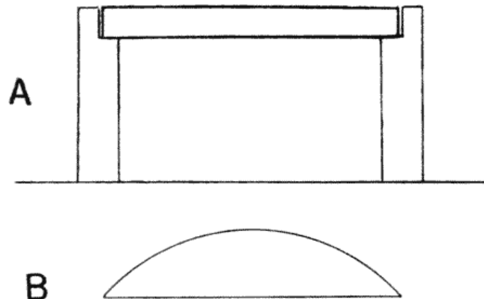
Fig. 340. A, Span of proposed bridge. B, Stress diagram, or diagram of bending-moments 628 .
