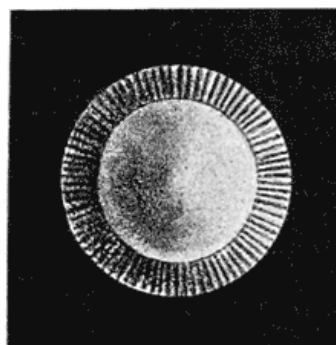
Fig. 196. A single calcospherite, with central “nucleus,” and striated, iridescent border. (After Harting.)
