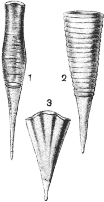
Fig. 295. Pteropod shells: (1) Cuvierina columnella ; (2) Cleodora chierchiaie ; (3) C. pygmaea . (After Boas.)
