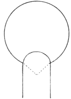
Fig. 112. Young antheridium of Chara .
