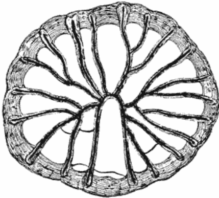
Fig. 173. Heterophyllia angulata . (After Nicholson.)
