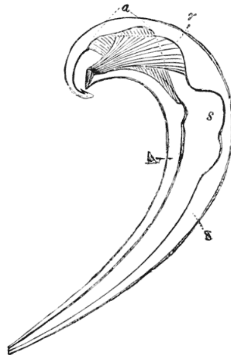
Fig. 291. Section of Productus ( Strophomena ) sp. (From Woods.)
