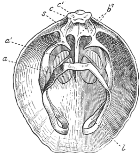
Fig. 292. Skeletal loop of Terebratula . (From Woods.)
