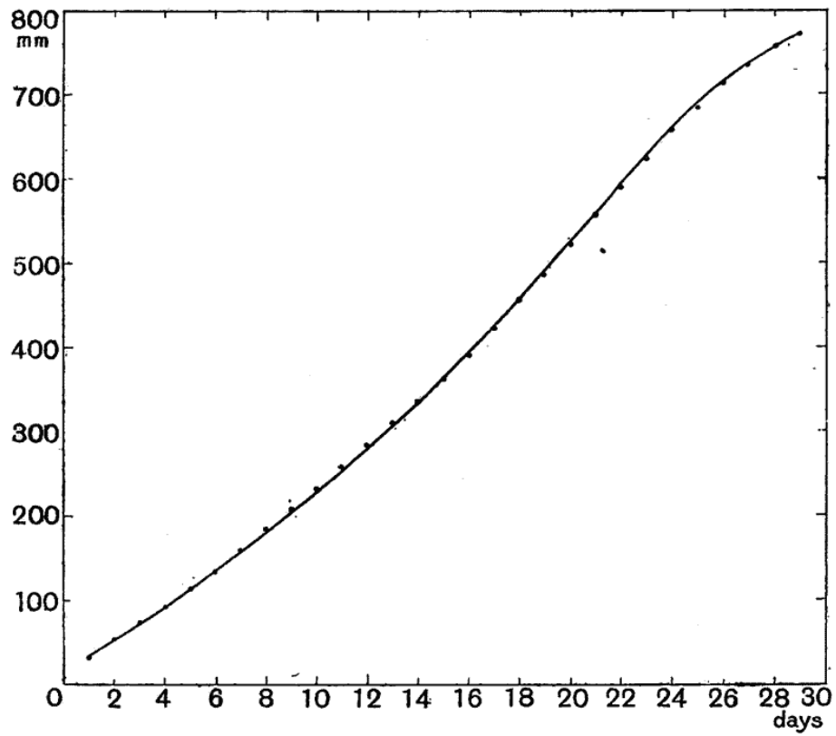
Fig. 10. Curve of growth of bamboo (from Ostwald, after Kraus).
