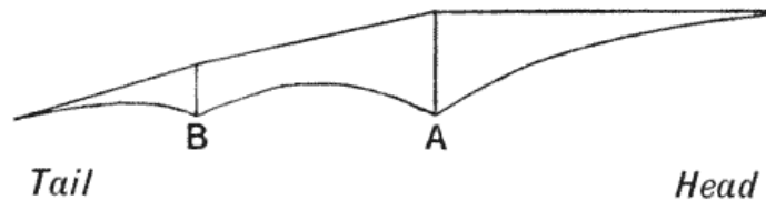
Fig. 347. Stress-diagram of horse's backbone.
