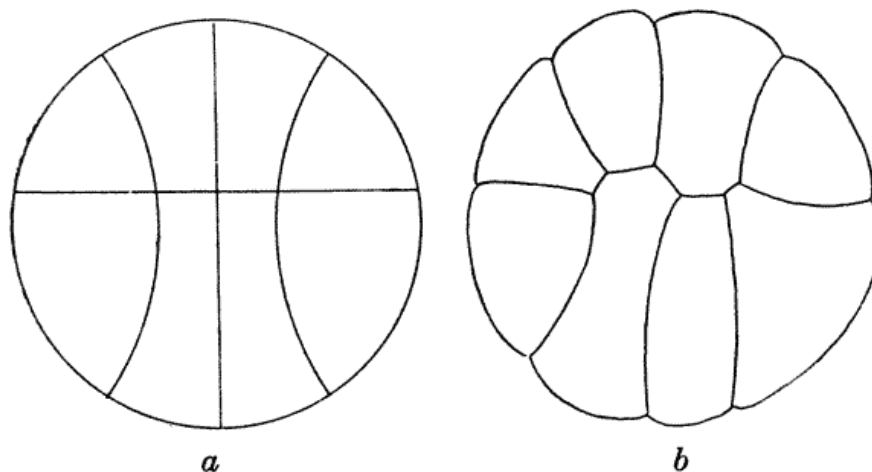
Fig. 162. (a) Section of apical cone of Salvinia . (After Pringsheim 394 .) (b) Diagram of probable actual arrangement.
