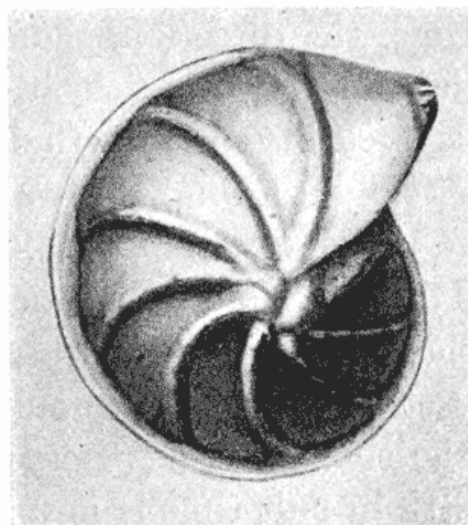
Fig. 260. Another spiral foraminifer, Crstellaria .
