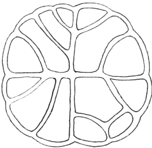
Fig. 192. Section through frond of Girardia sphacelaria . (After Goebel.)
