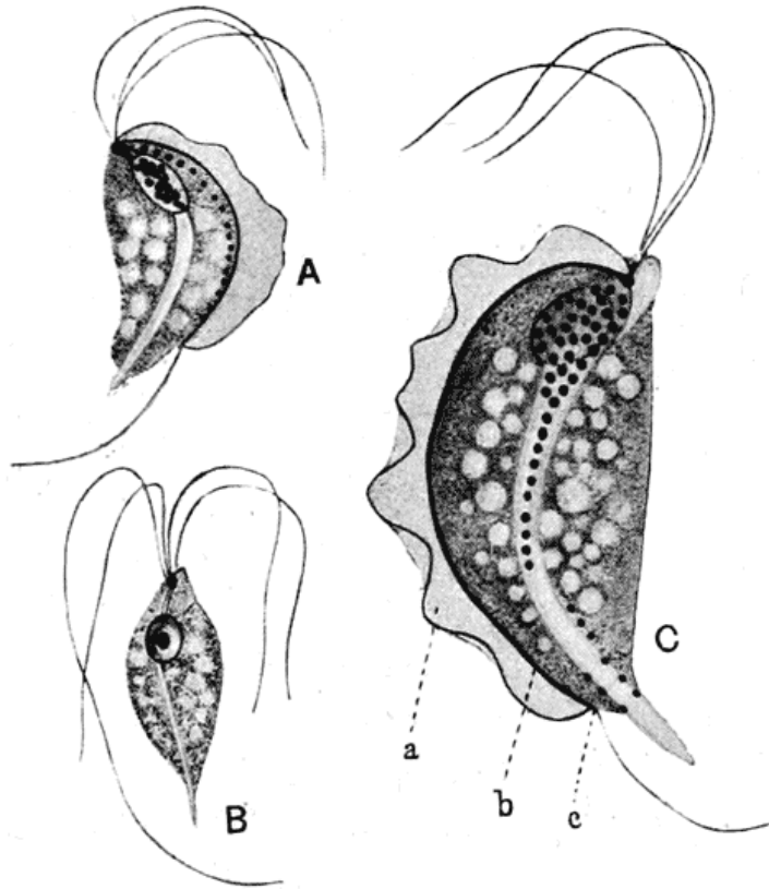
Fig. 91. A, Trichomonas muris , Hartmann; B, Trichomastix serpentis , Dobell; C, Trichomonas angusta , Alexeieff. (After Kofoed.)
