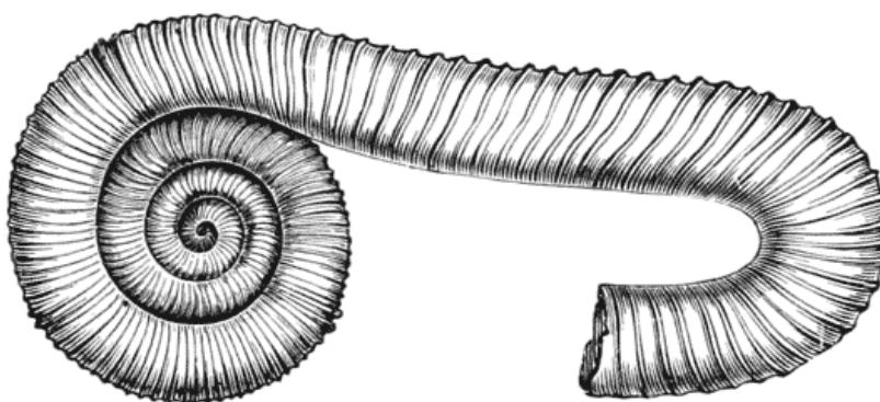
Fig. 281. An ammonitoid shell ( Macroscephites ) to shew change of curvature.
