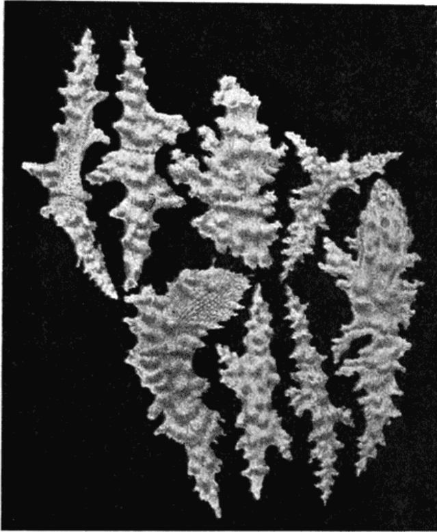
Fig. 200. Additional illustrations of Alcyonarian spicules: Eunicea . (After Studer.)
