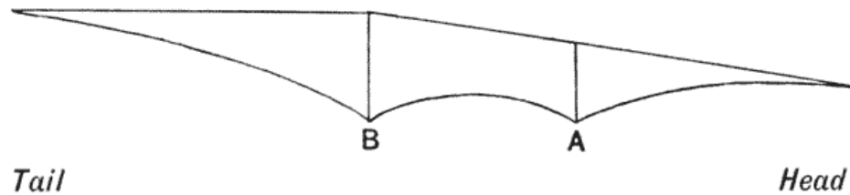
Fig. 348. Stress-diagram of backbone of Dinosaur.
