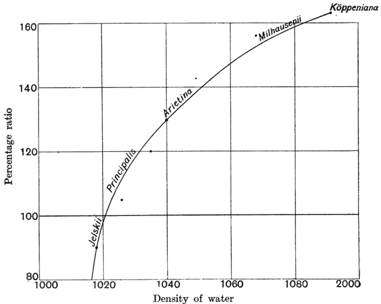
Fig. 34. Percentage ratio of length of abdomen to cephalothorax in brine-shrimps, at various salinities. (After Abonyi.)
