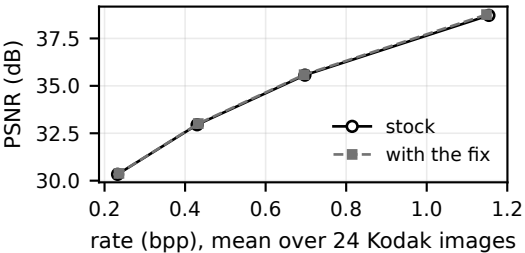
(a) Kodak, four values of \lambda
