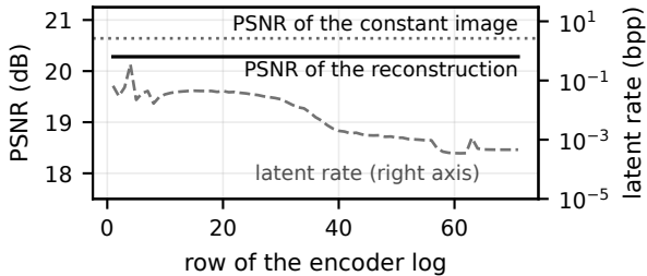
(b) stock encode of code01, \lambda = 0.0002
