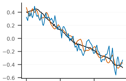
Acceleration lateral FM 1.86/r 0.30 · OC 1.39/r 0.09
