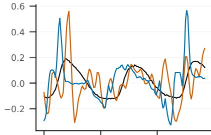
Acceleration vertical FM 3.45/r 0.11 · OC 4.24/r 0.16
