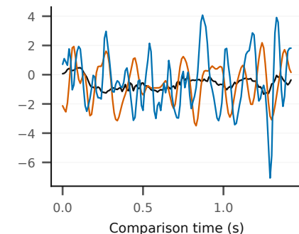
Acceleration lateral FM 1.86/r 0.30 · OC 1.39/r 0.09
