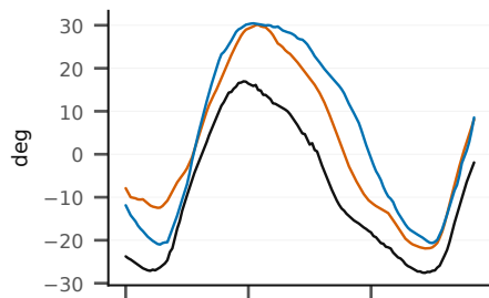
Hip flexion L FM 14.7°/r 0.94 · OC 11.4°/r 0.98
