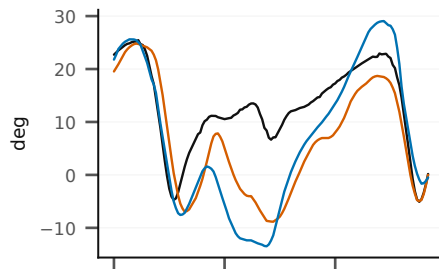
Ankle flexion L FM 10.9°/r 0.75 · OC 9.3°/r 0.76
