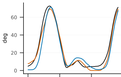
Knee flexion L FM 7.7°/r 0.96 · OC 4.3°/r 0.99
