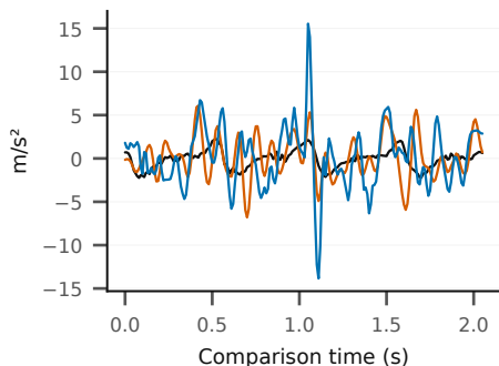
Acceleration progression FM 3.37/r 0.30 · OC 2.41/r 0.24
