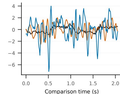
Acceleration lateral FM 1.82/r 0.15 · OC 0.98/r 0.26
