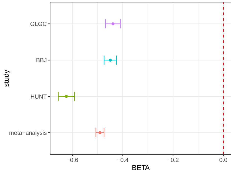
Forest plot for APOE (19:44897490:A:T)
