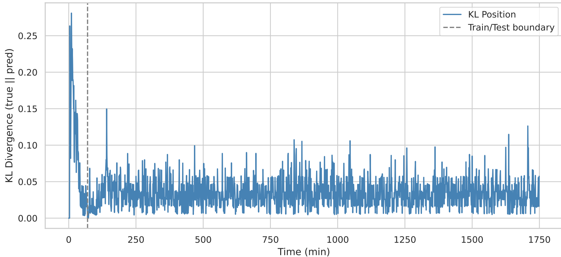
Final Position KL Divergence: mamba — Pos KL=0.0574
