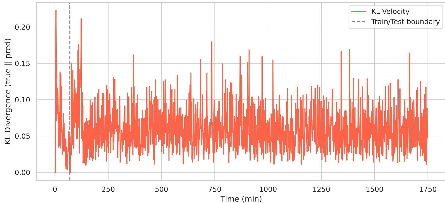
Final Velocity KL Divergence: mamba — Vel KL=0.0472
