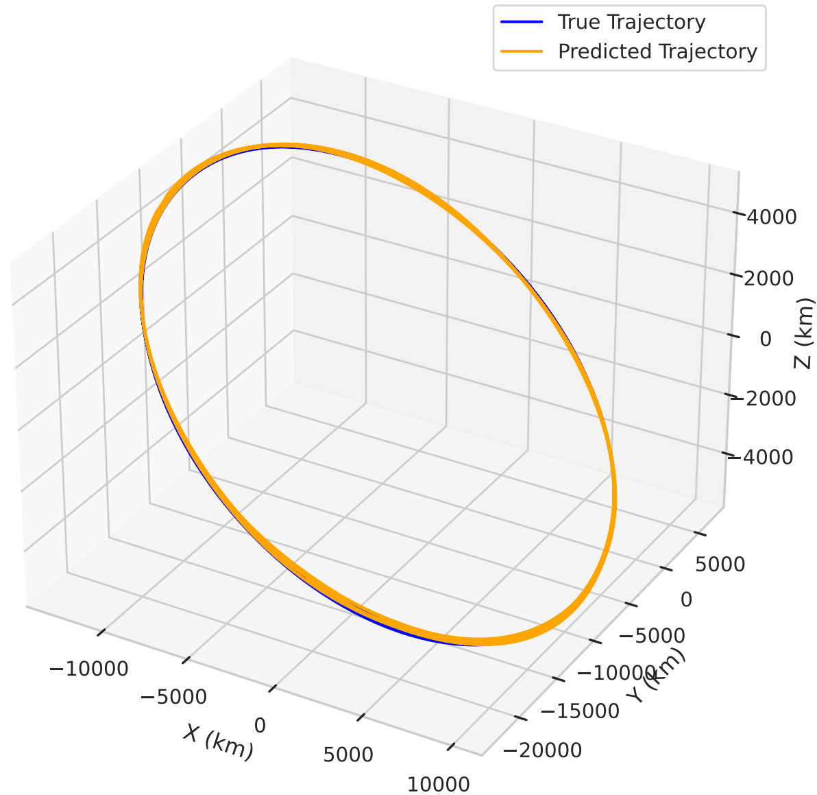
MAMBA Prediction for Trajectory 124 Orbit: HEO, Propagation: 1750min, Train Ratio: 0.1, Epochs: 10
