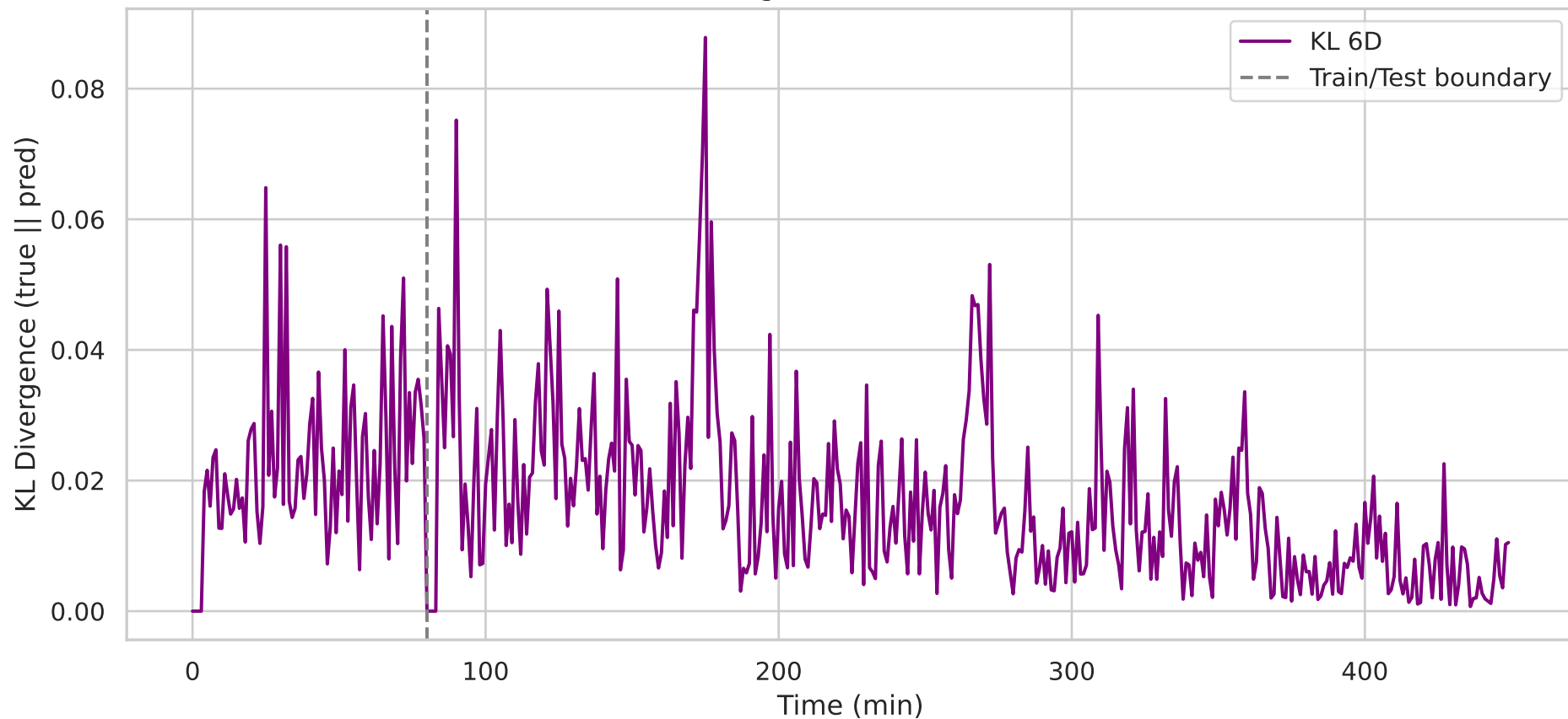
Full 6D KL Divergence: mamba — KL=0.0105
