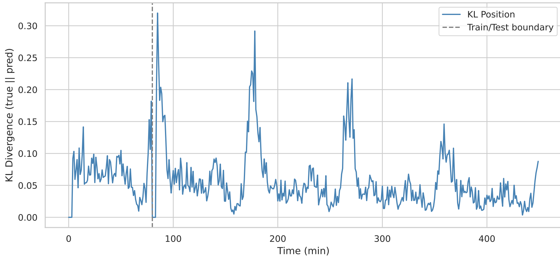
Final Position KL Divergence: mamba — Pos KL=0.0877
