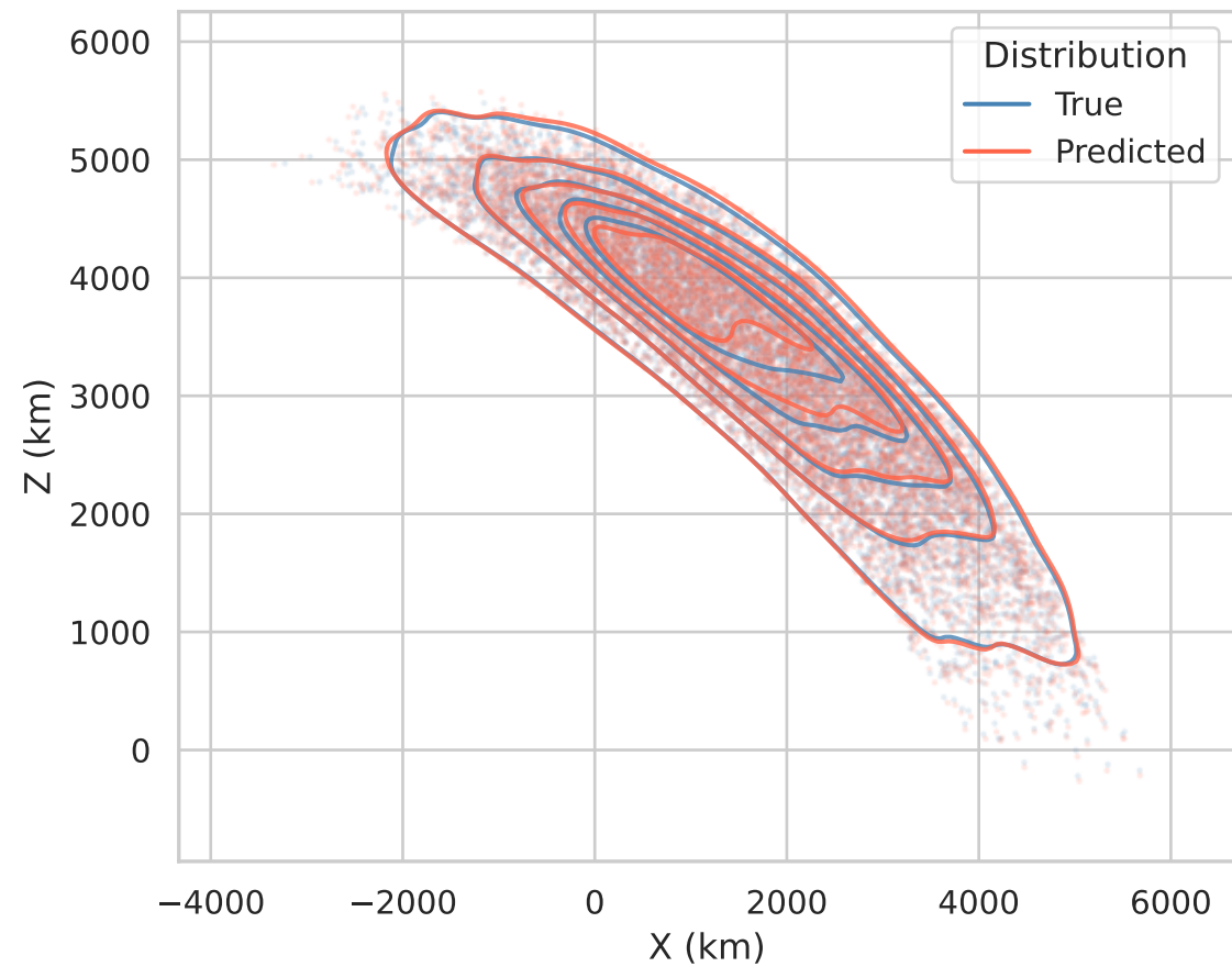
Final State PDF: mamba
